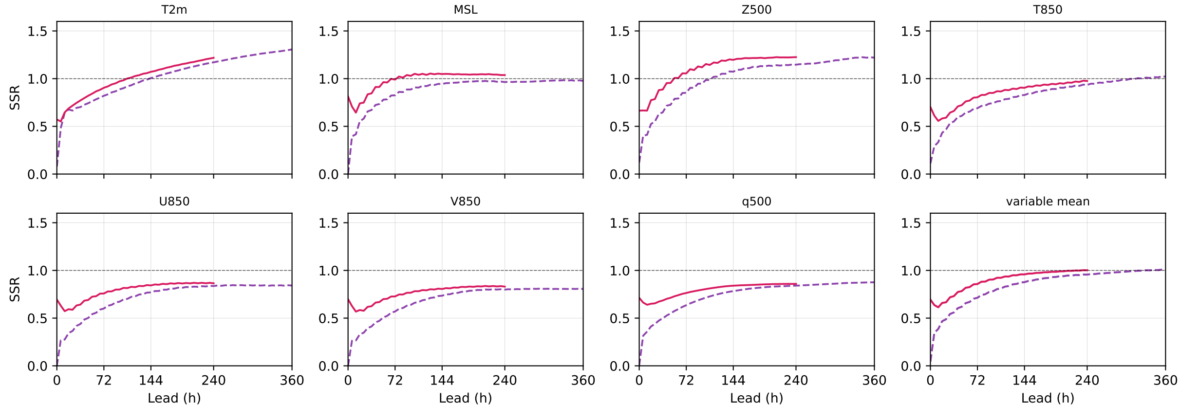
Phase 5 AIFS: lead-resolved SSR, weight-only vs IFS-ENS-IC + weight
