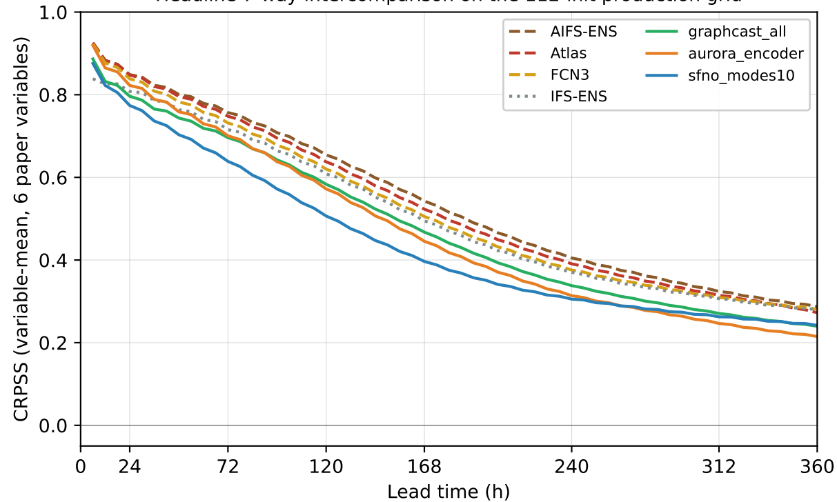
Headline 7-way intercomparison on the 112-init production grid
