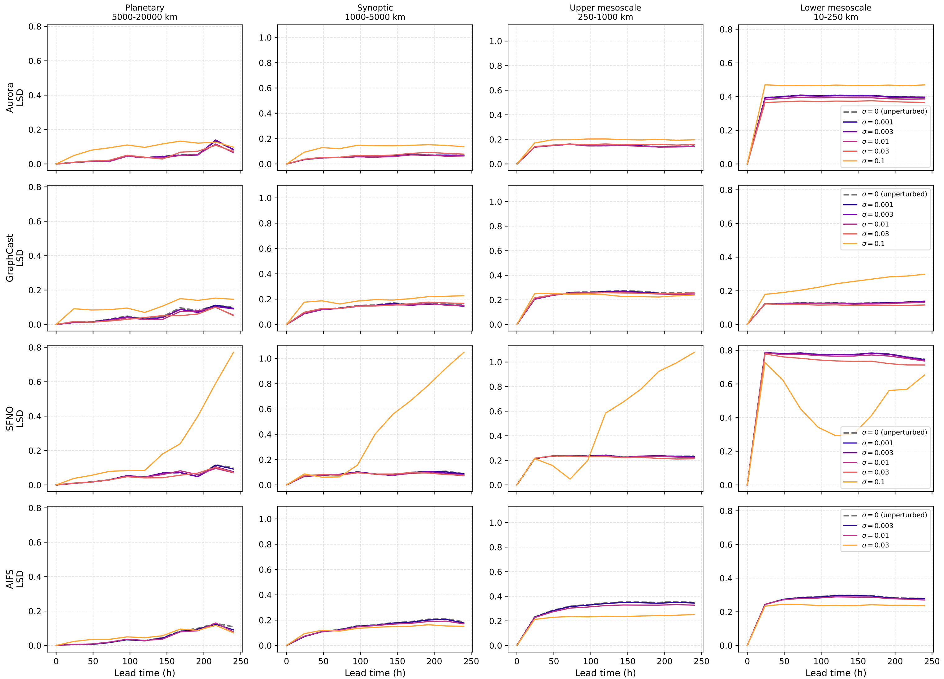
Band-integrated log spectral distance, 10m_u_component_of_wind (Phase-1 sweep, ensemble-pooled)
