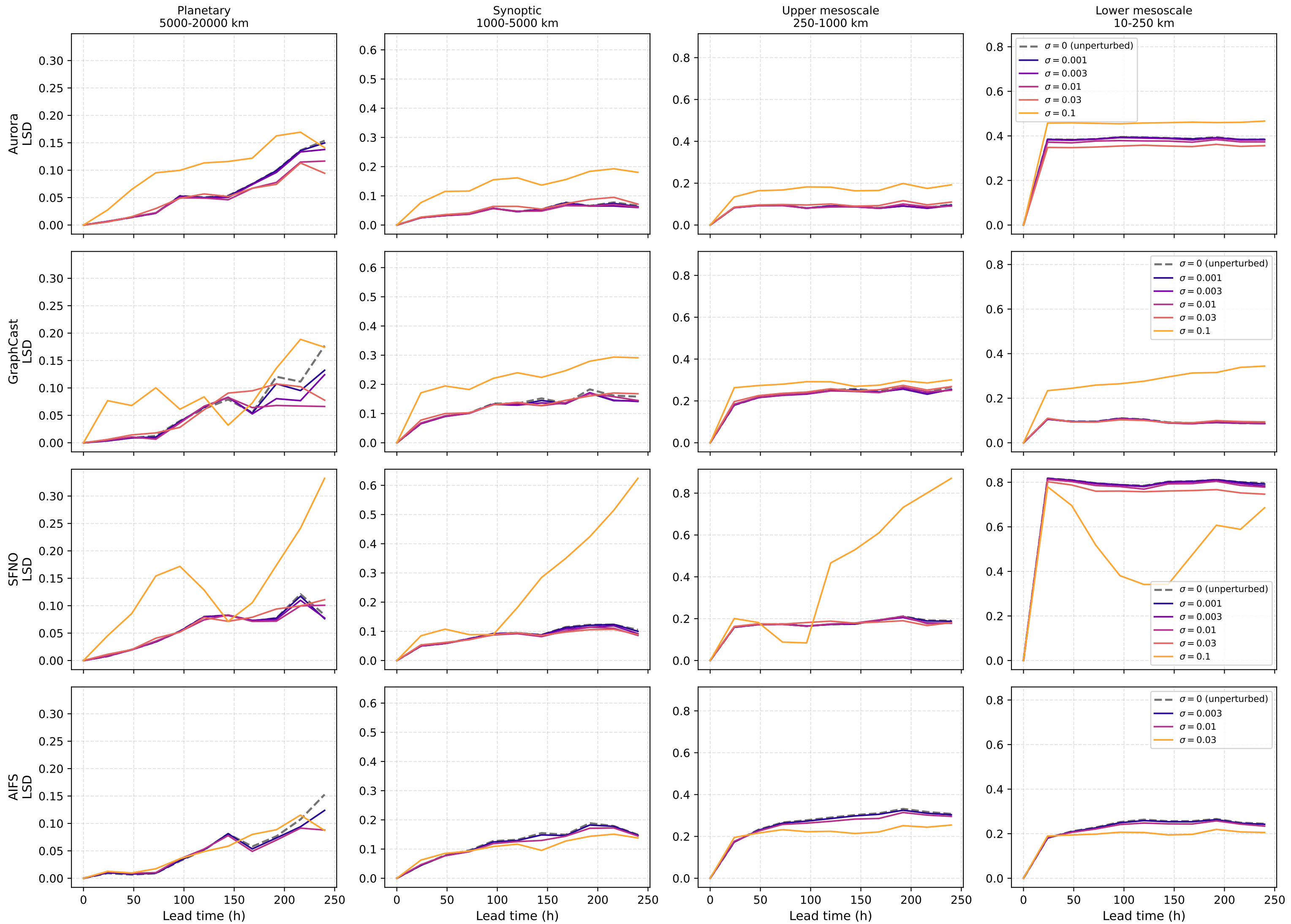
Band-integrated log spectral distance, 10m_v_component_of_wind (Phase-1 sweep, ensemble-pooled)
