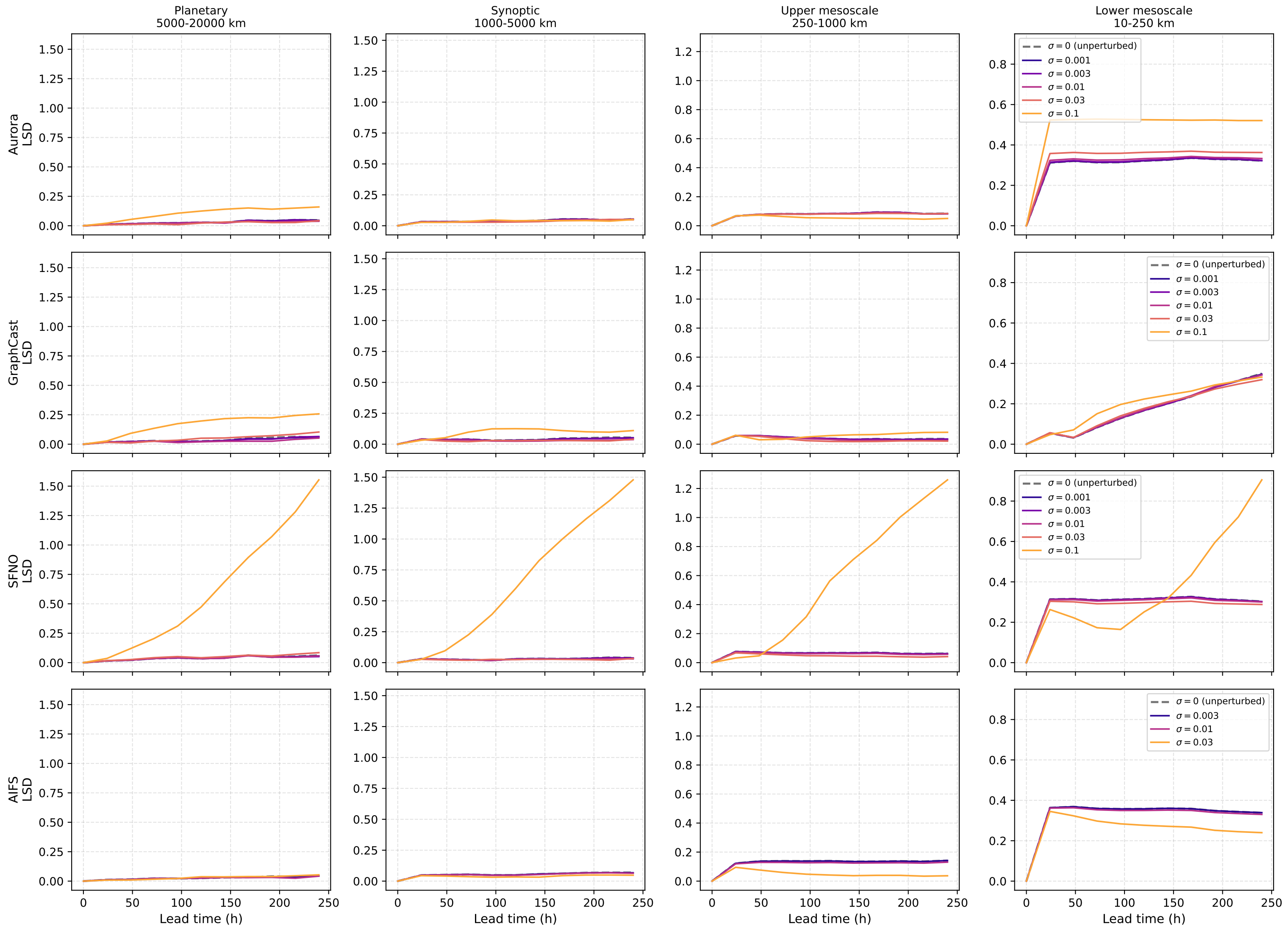
Band-integrated log spectral distance, 2m_temperature (Phase-1 sweep, ensemble-pooled)
