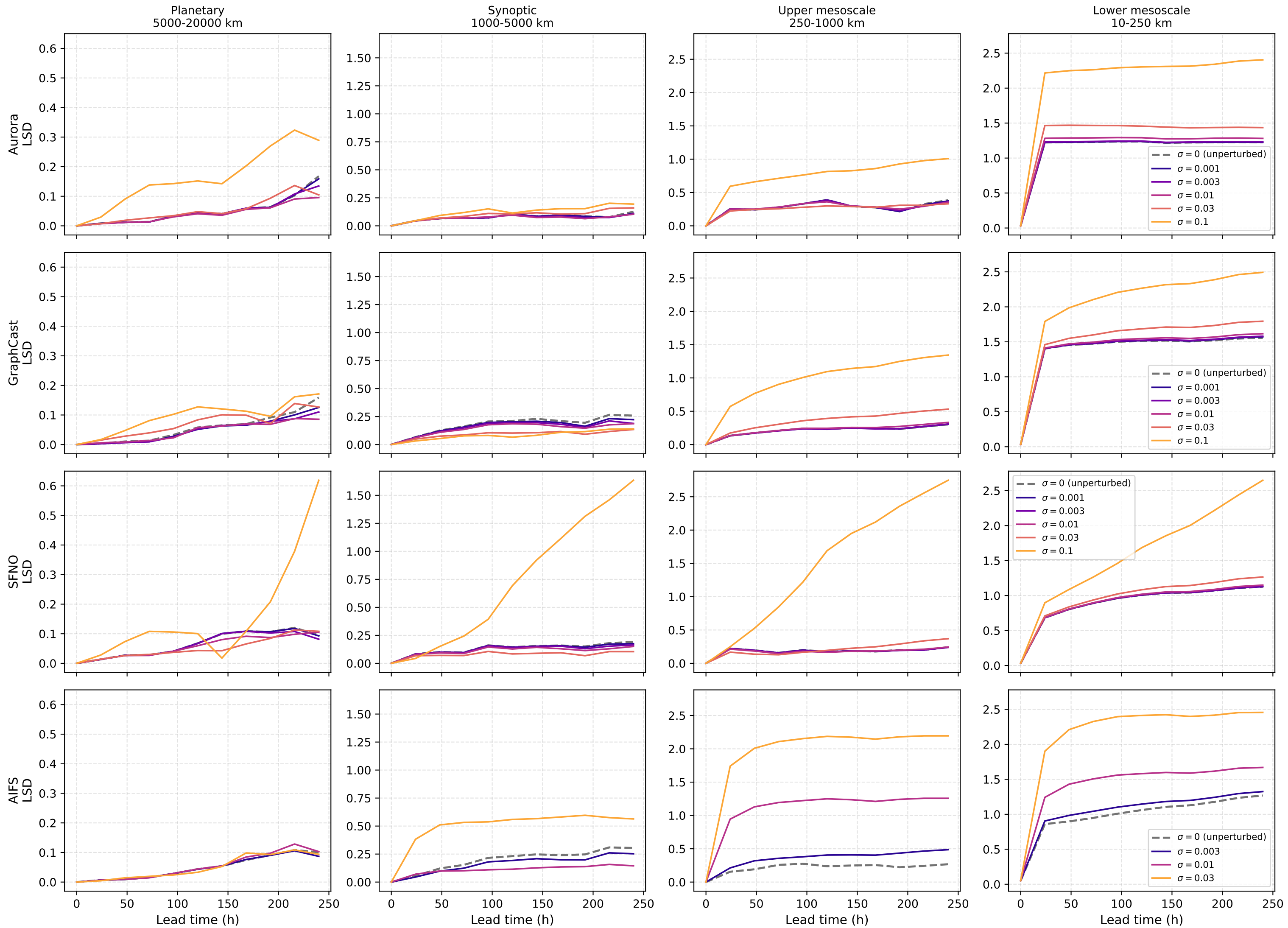
Band-integrated log spectral distance, geopotential@500hPa (Phase-1 sweep, ensemble-pooled)
