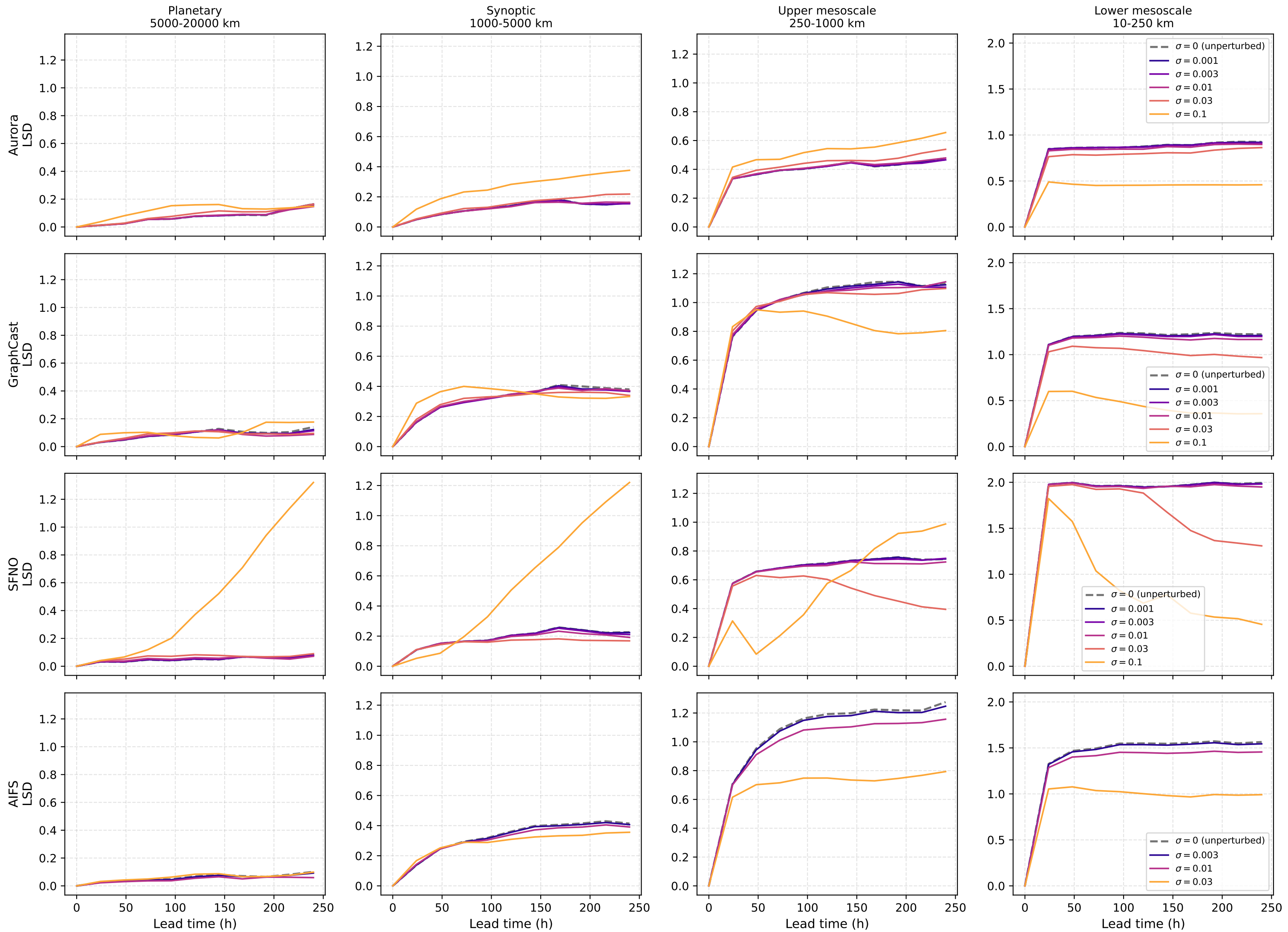
Band-integrated log spectral distance, specific_humidity@500hPa (Phase-1 sweep, ensemble-pooled)
