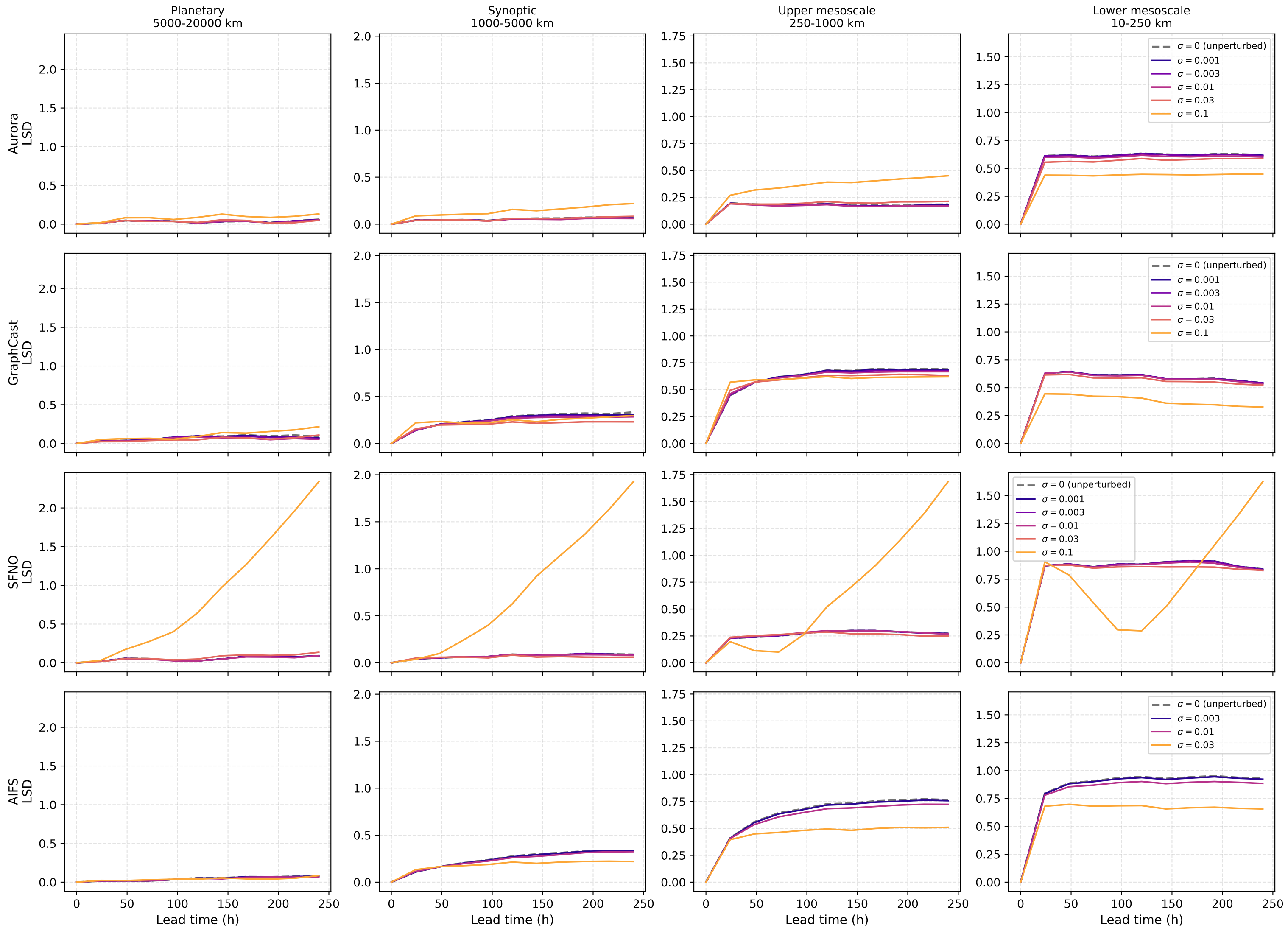
Band-integrated log spectral distance, specific_humidity@850hPa (Phase-1 sweep, ensemble-pooled)
