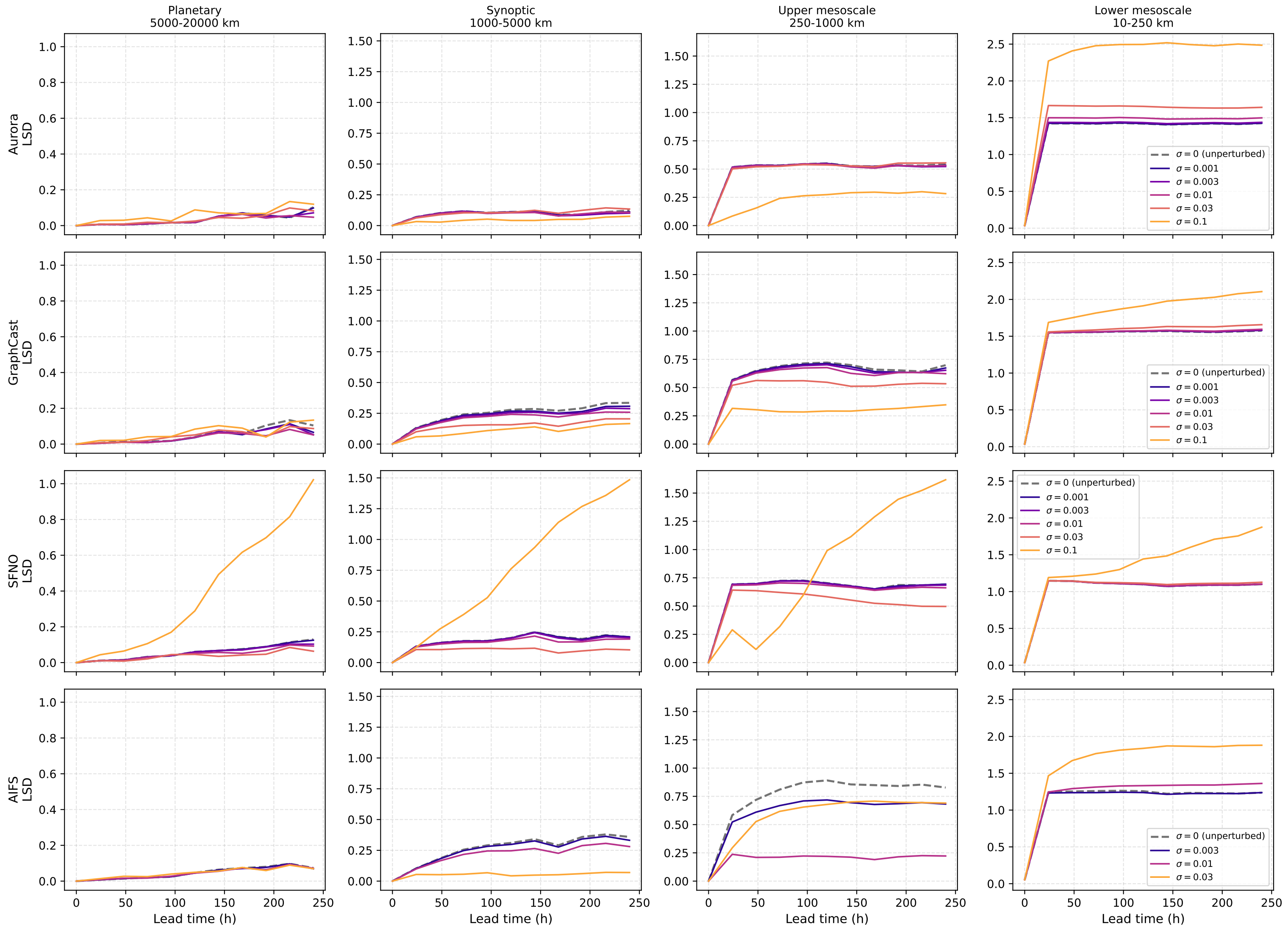
Band-integrated log spectral distance, temperature@500hPa (Phase-1 sweep, ensemble-pooled)
