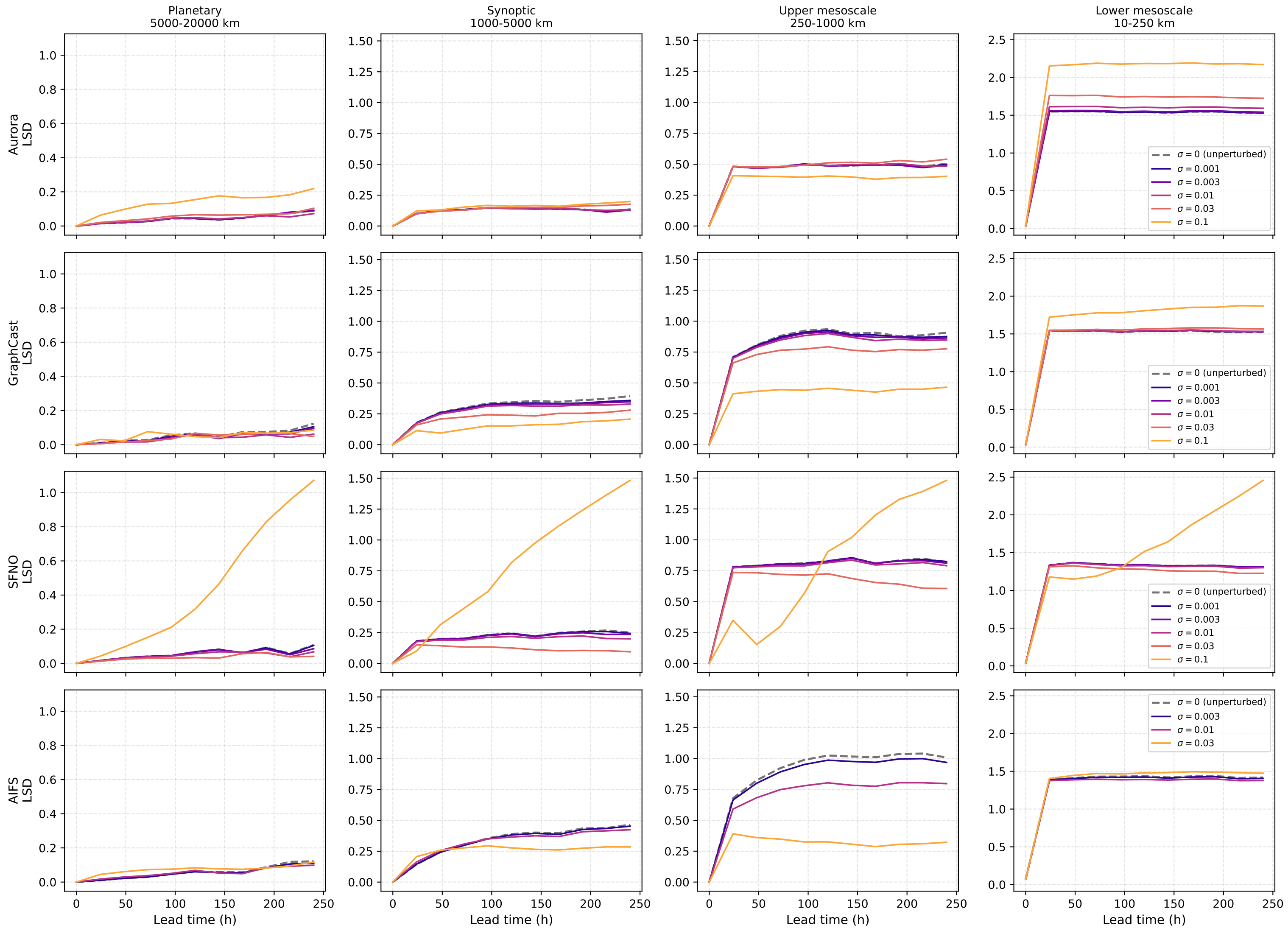
Band-integrated log spectral distance, u_component_of_wind@500hPa (Phase-1 sweep, ensemble-pooled)
