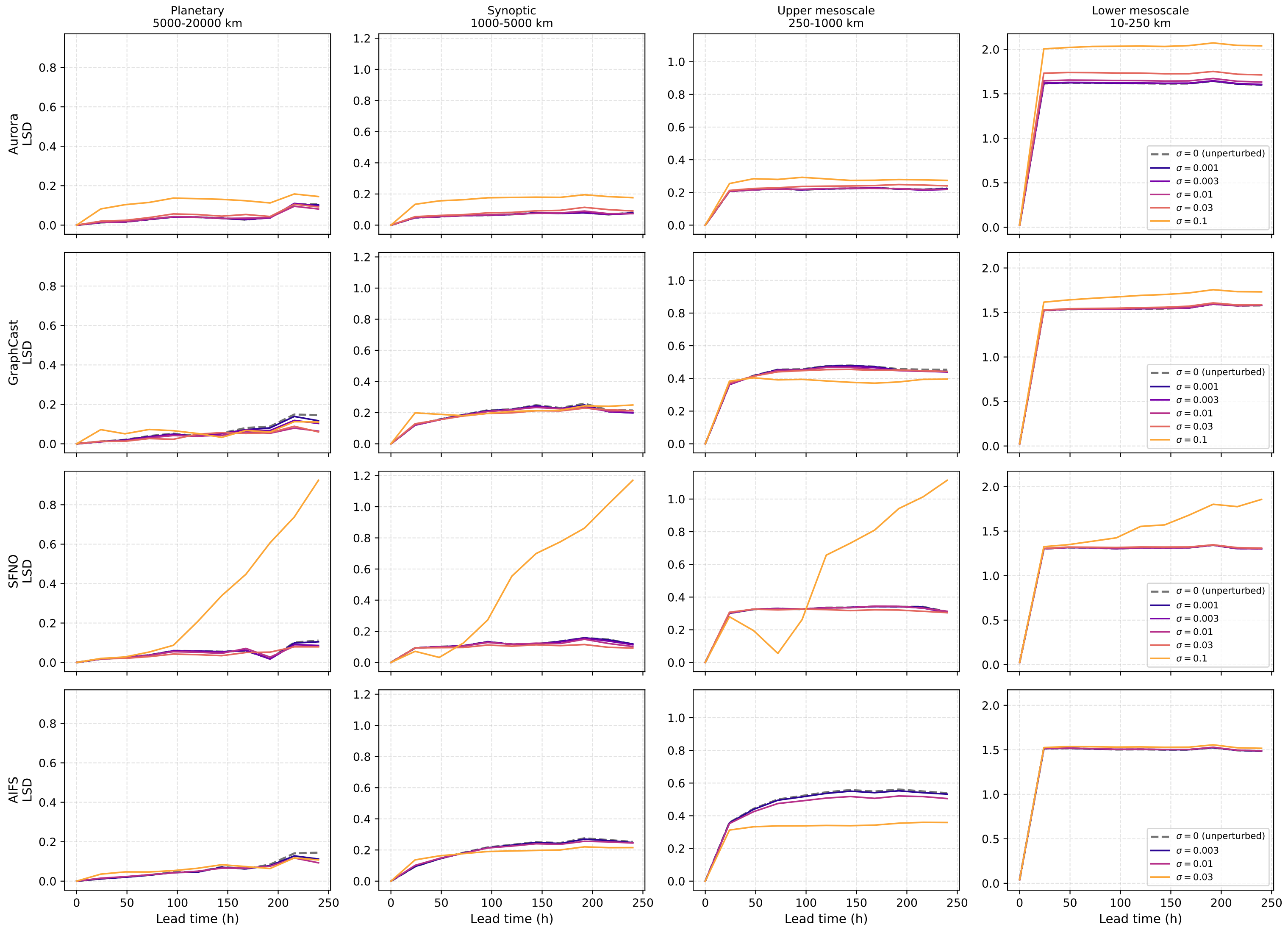
Band-integrated log spectral distance, u_component_of_wind@850hPa (Phase-1 sweep, ensemble-pooled)
