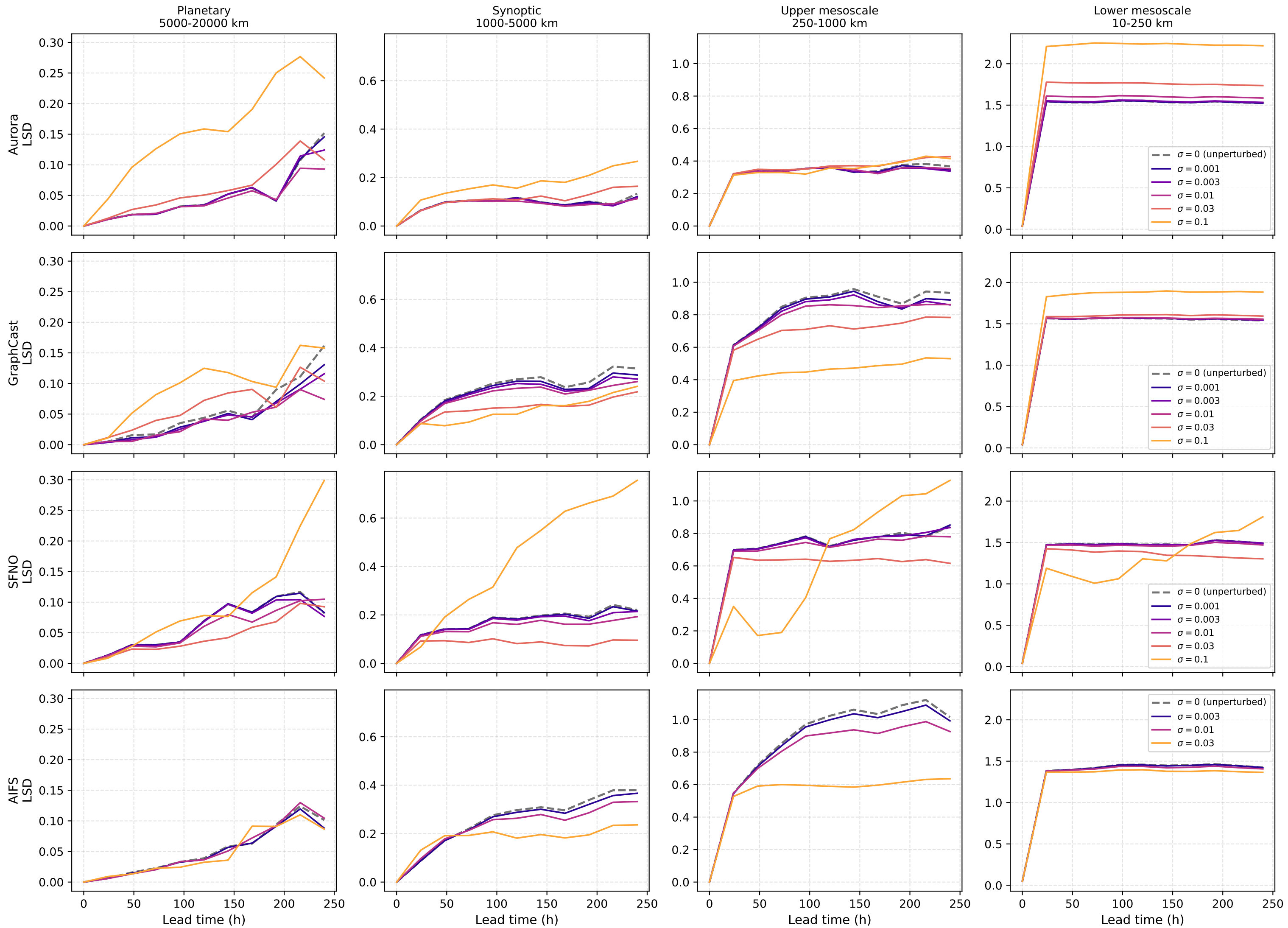
Band-integrated log spectral distance, v_{\text{component\_of\_wind@500hPa}} (Phase-1 sweep, ensemble-pooled)
