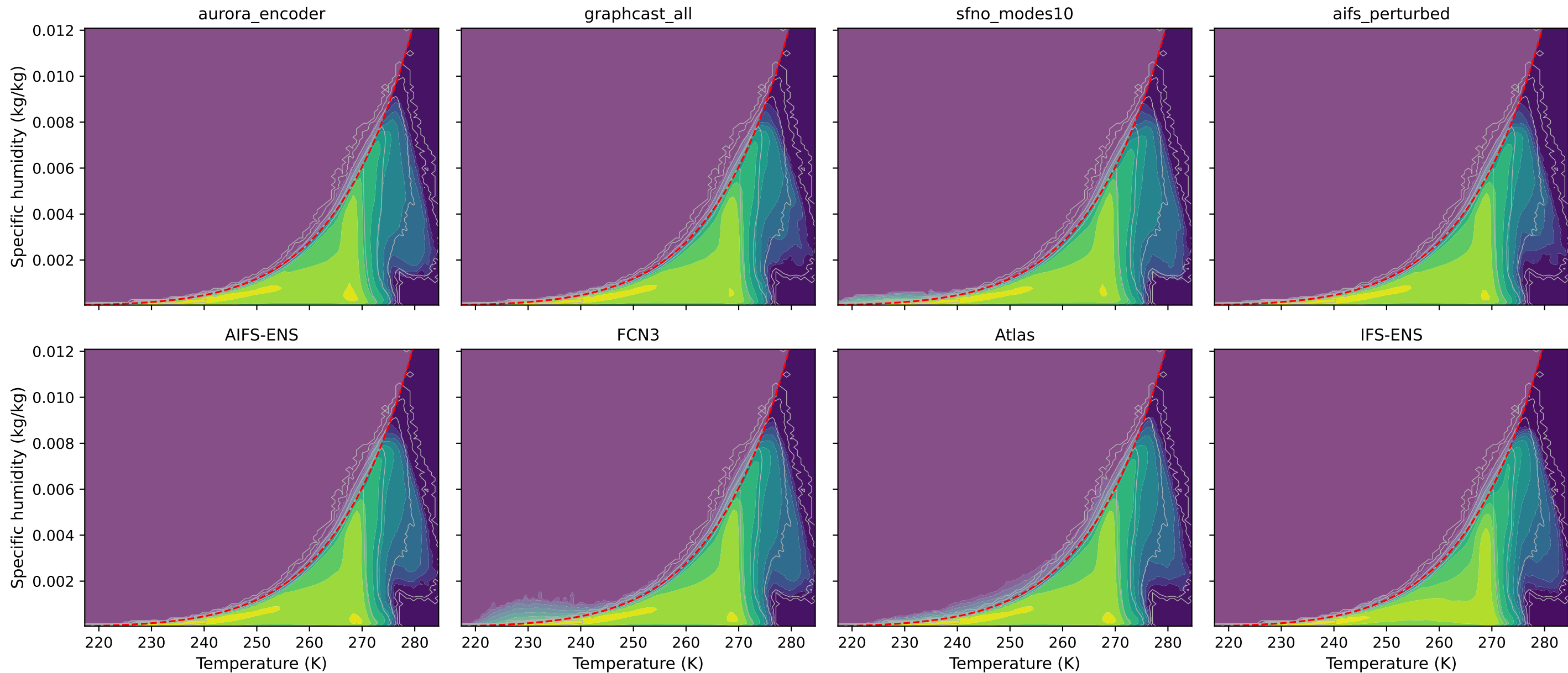
Joint T - q distribution at 500 hPa (forecast filled, truth grey)
