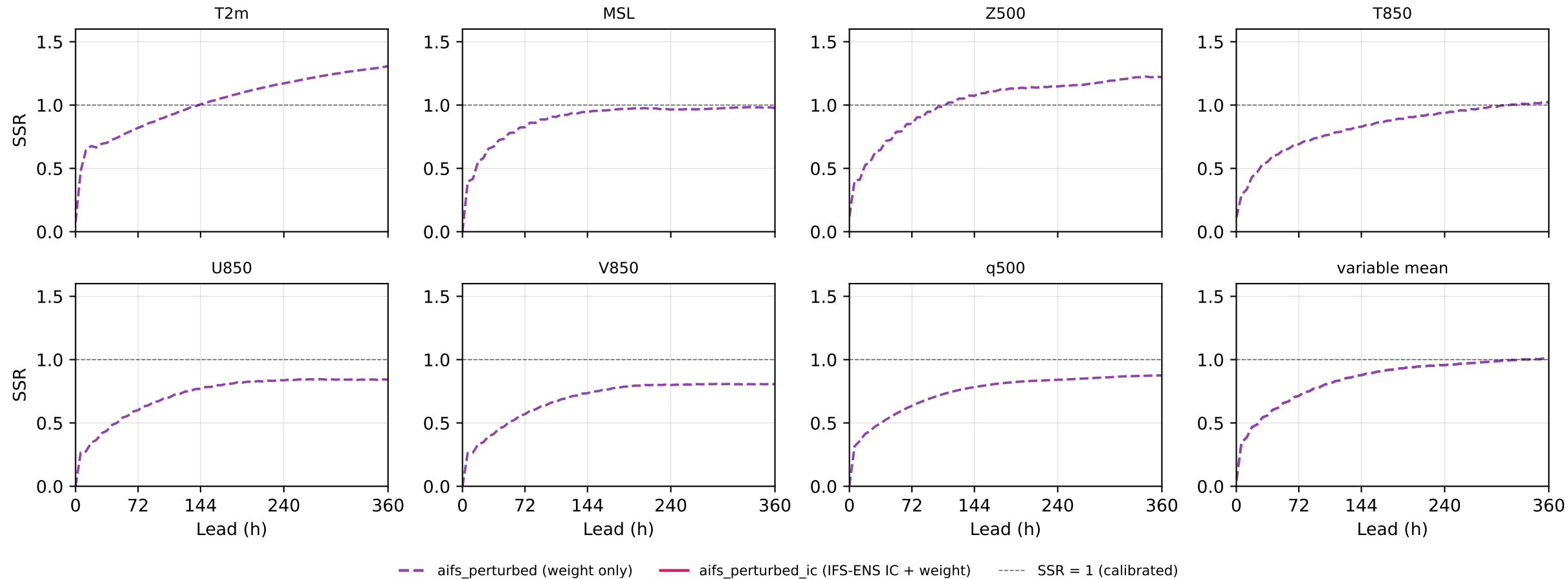
Phase 5 AIFS: lead-resolved SSR, weight-only vs IFS-ENS-IC + weight
