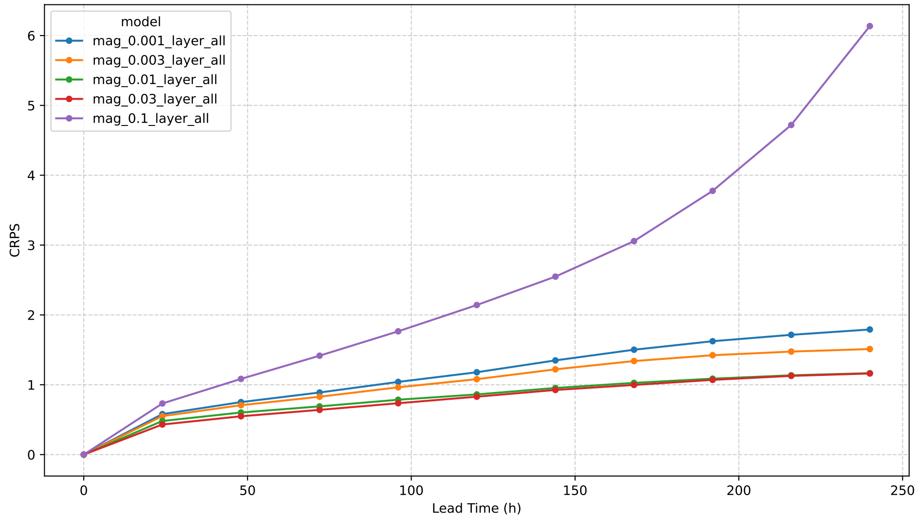
CRPS vs Lead Time — T2m
