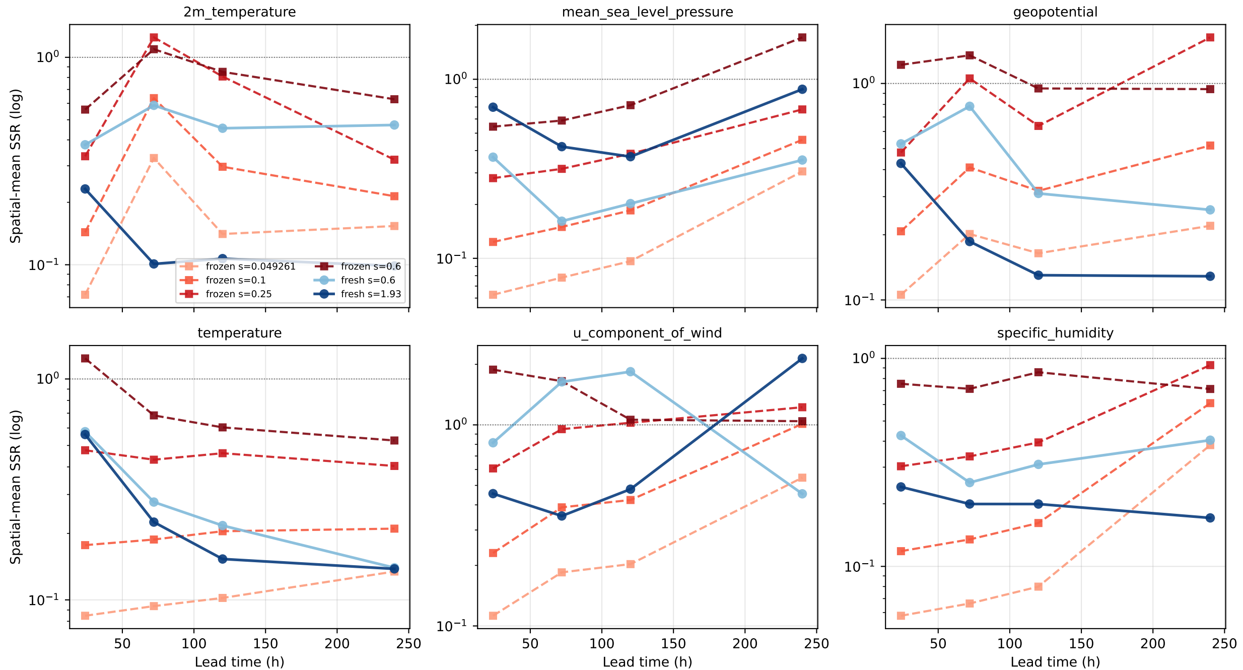
Phase 6 SFNO: spatial-mean SSR -- fresh-per-step vs frozen, modes10
