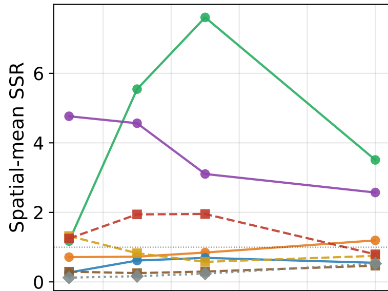
2 m temperature (2t)
