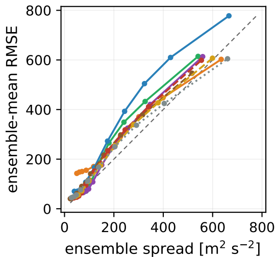
z500 500 hPa, lead 120 h
