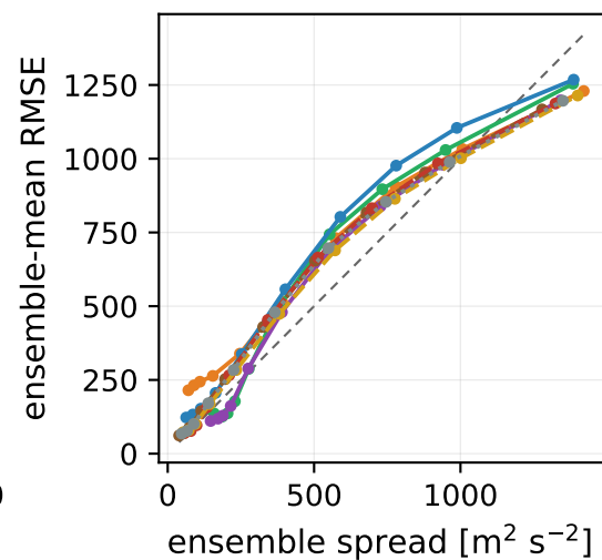
z500 500 hPa, lead 240 h
