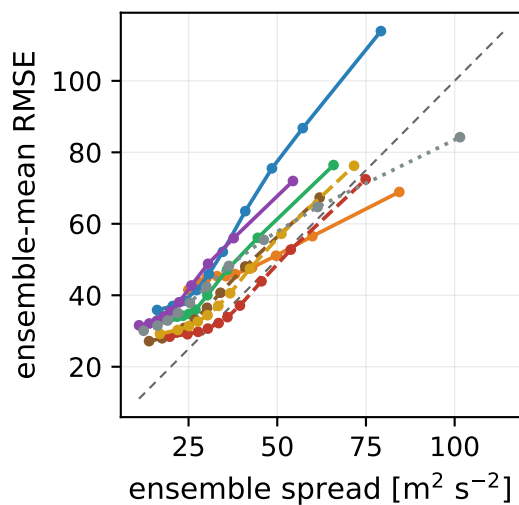
z500 500 hPa, lead 24 h
