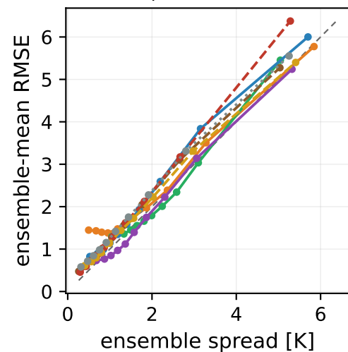
z500 500 hPa, lead 240 h
