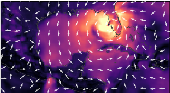
AIFS-perturbed
