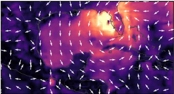
AIFS-ENS
