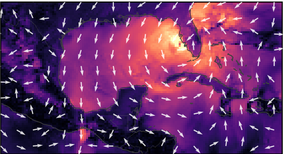
IFS-ENS
