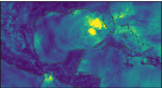
10 m wind speed ( \text{m s}^{-1} )
