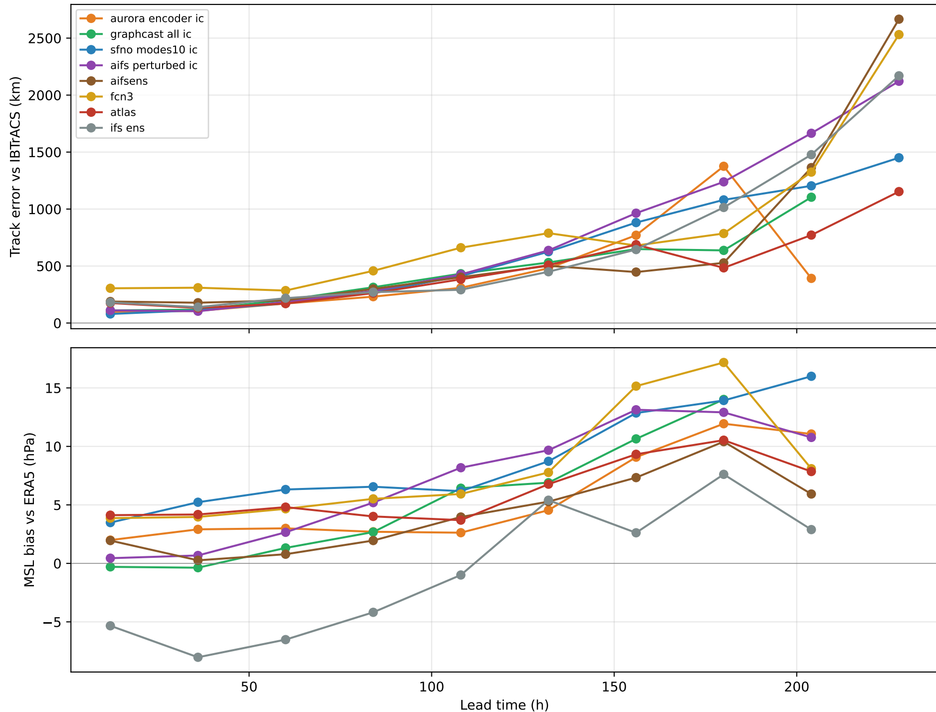
Milton verification: track position error and MSL intensity bias vs lead time
