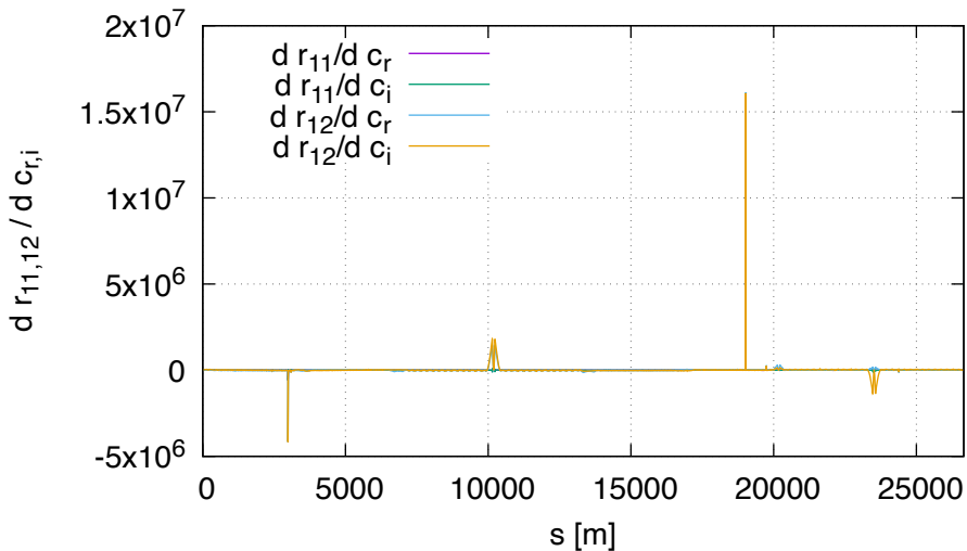
Sensitivity of R11,R12 DA (lhcb1, order 2)
