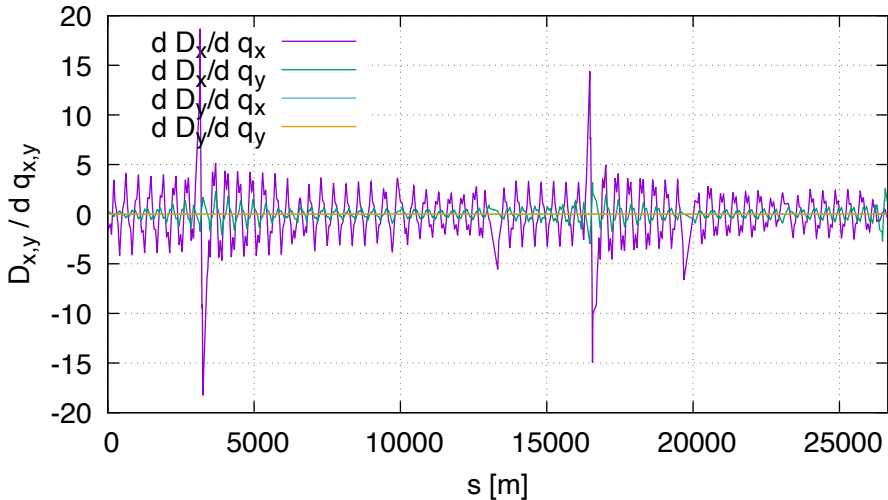
Sensitivity of disp FD (lhcb2, order 2)
