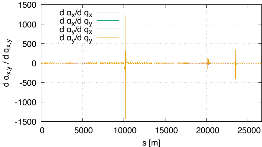
Sensitivity of alf DA (lhcb1, order 2)
