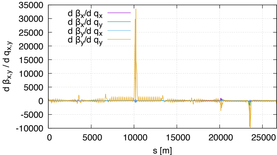
Sensitivity of bet DA (lhcb1, order 2)
