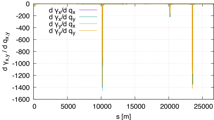
Sensitivity of gamma FD (lhcb1, order 2)
