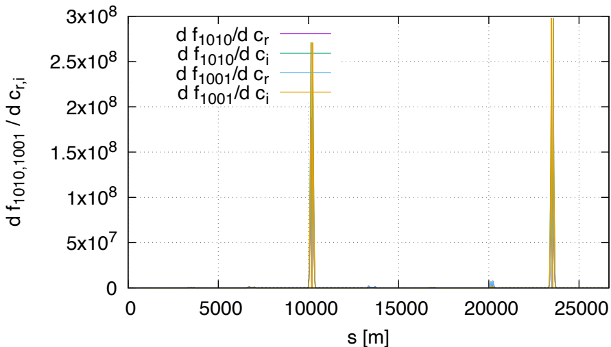
Sensitivity of f1010,f1001 FD (lhcb1, order 1)
