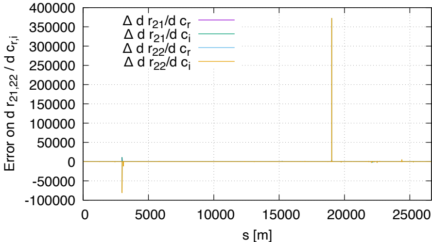
Sensitivity error of R21,R22 FD vs DA (lhcb1, order 2)
