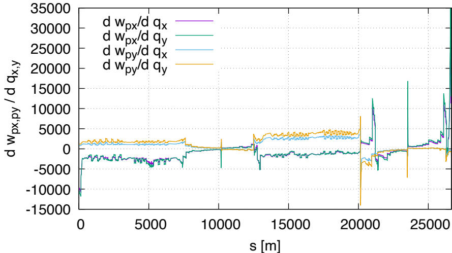
Sensitivity of wp FD (lhcb1, order 2)
