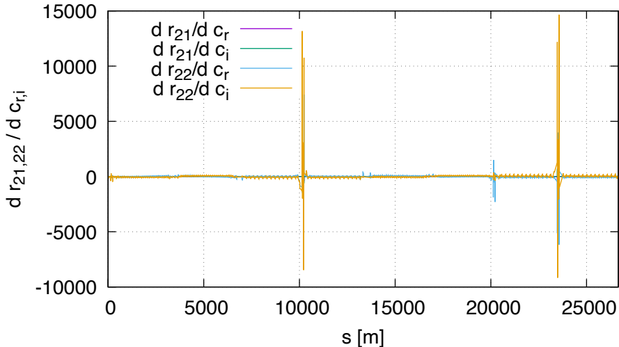
Sensitivity of R21,R22 FD (lhcb1, order 1)
