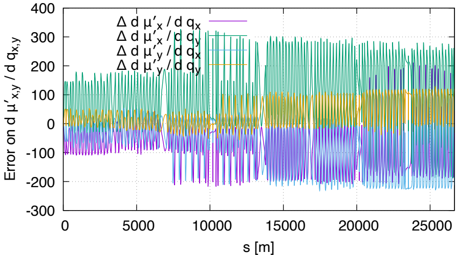
Sensitivity error of dm \mu FD vs DA (lhcb1, order 1)
