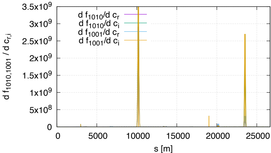
Sensitivity of f1010,f1001 DA (lhcb1, order 2)
