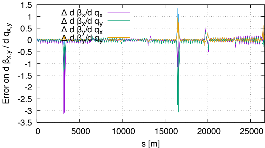
Sensitivity error of bet FD vs DA (lhcb2, order 1)
