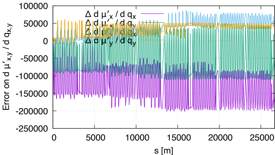
Sensitivity error of dm \mu FD vs DA (lhcb2, order 2)
