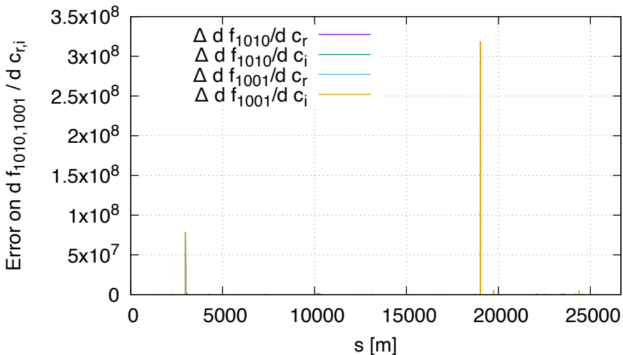
Sensitivity error of f1010,f1001 FD vs DA (lhcb1, order 2)
