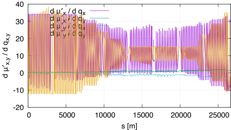
Sensitivity of dm \mu DA (lhcb2, order 1)
