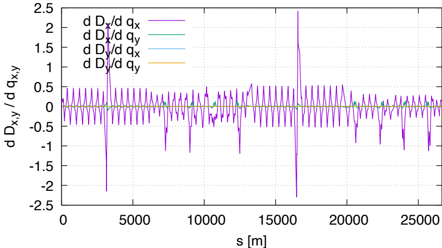
Sensitivity of disp DA (lhcb2, order 1)
