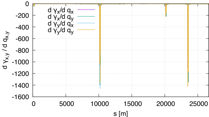
Sensitivity of gamma DA (lhcb1, order 2)
