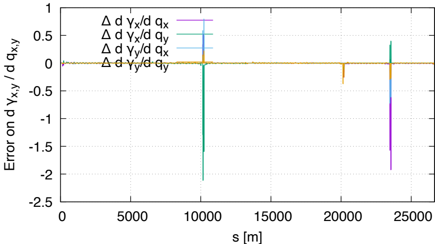
Sensitivity error of gamma FD vs DA (lhcb1, order 2)
