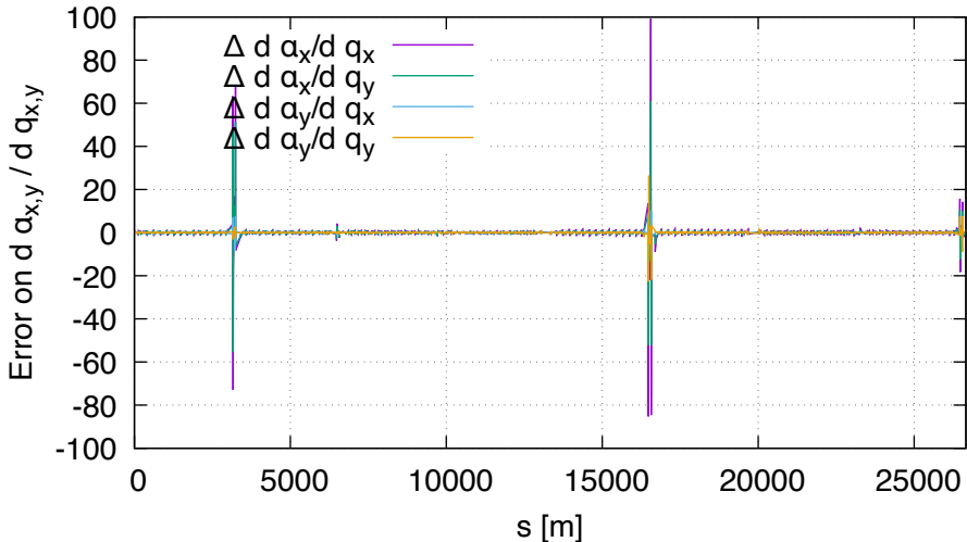
Sensitivity error of alpha FD vs DA (lhcb2, order 2)
