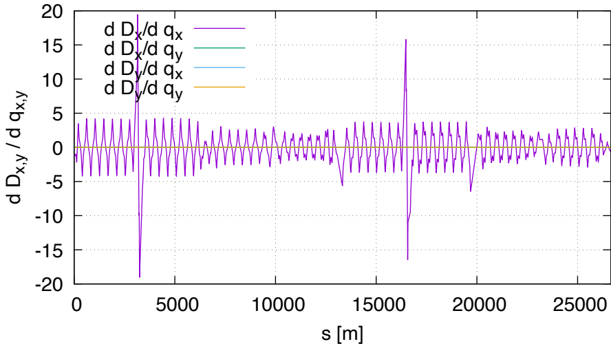
Sensitivity of disp DA (lhcb2, order 2)
