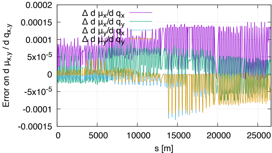
Sensitivity error of mu FD vs DA (lhcb2, order 1)
