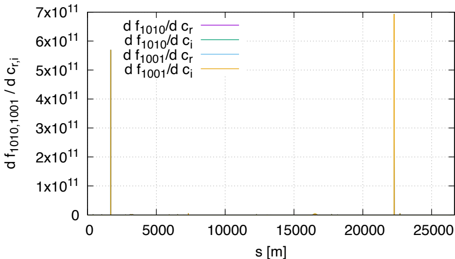
Sensitivity of f1010,f1001 DA (lhcb2, order 2)
