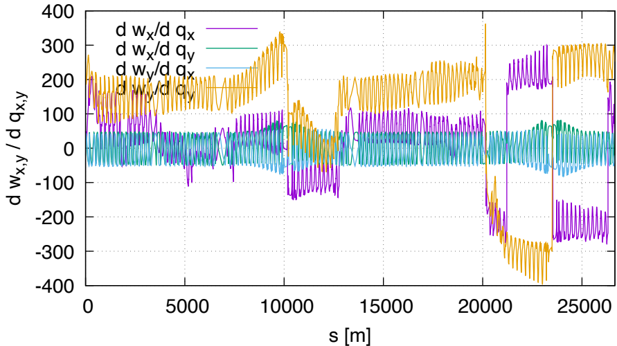
Sensitivity of w DA (lhcb1, order 1)
