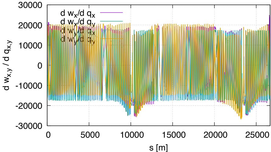
Sensitivity of w DA (lhcb1, order 2)
