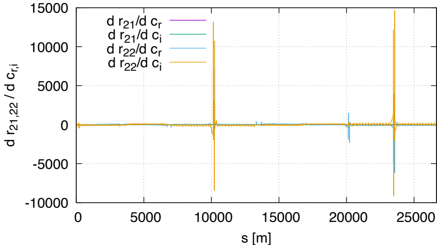
Sensitivity of R21,R22 DA (lhcb1, order 1)
