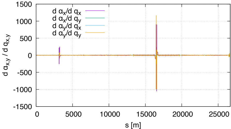
Sensitivity of alf DA (lhcb2, order 2)
