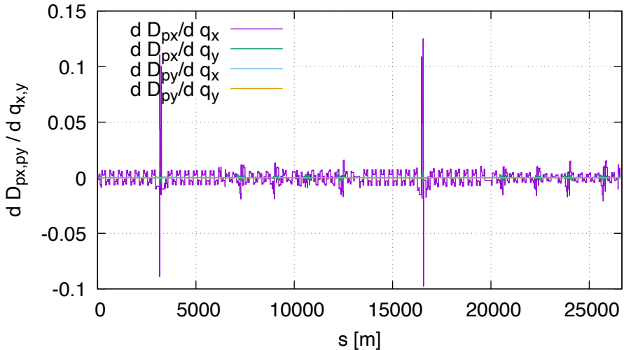
Sensitivity of dispp FD (lhcb2, order 1)
