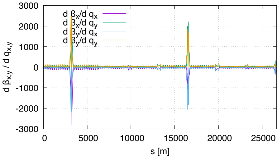
Sensitivity of beta FD (lhcb2, order 1)
