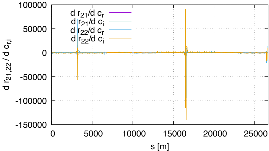
Sensitivity of R21,R22 FD (lhcb2, order 2)
