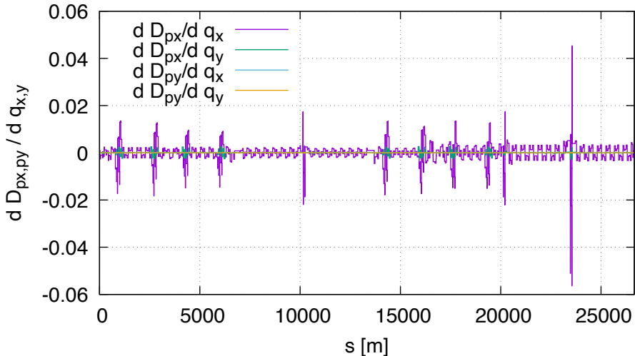
Sensitivity of dispp FD (lhcb1, order 1)
