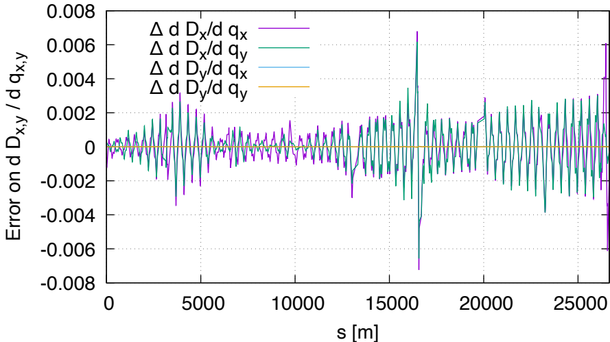
Sensitivity error of disp FD vs DA (lhcb2, order 1)
