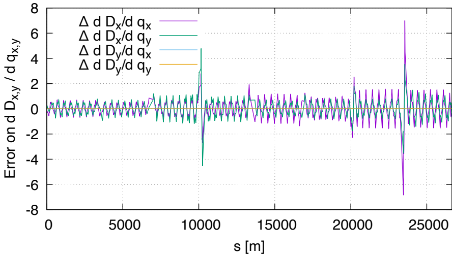
Sensitivity error of disp FD vs DA (lhcb1, order 2)
