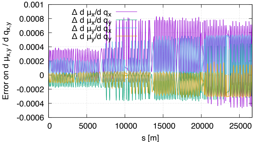
Sensitivity error of mu FD vs DA (lhcb1, order 1)
