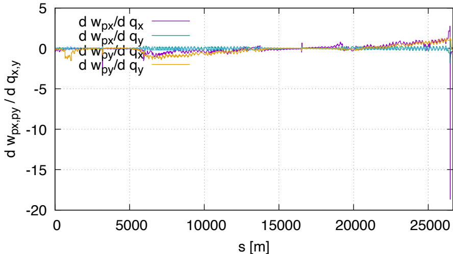
Sensitivity of wp DA (lhcb2, order 1)
