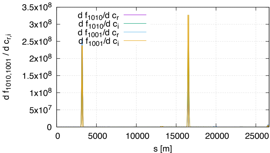
Sensitivity of f1010,f1001 FD (lhcb2, order 1)
