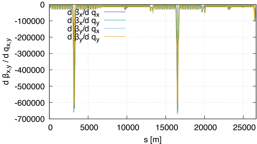
Sensitivity of beta DA (lhcb2, order 2)
