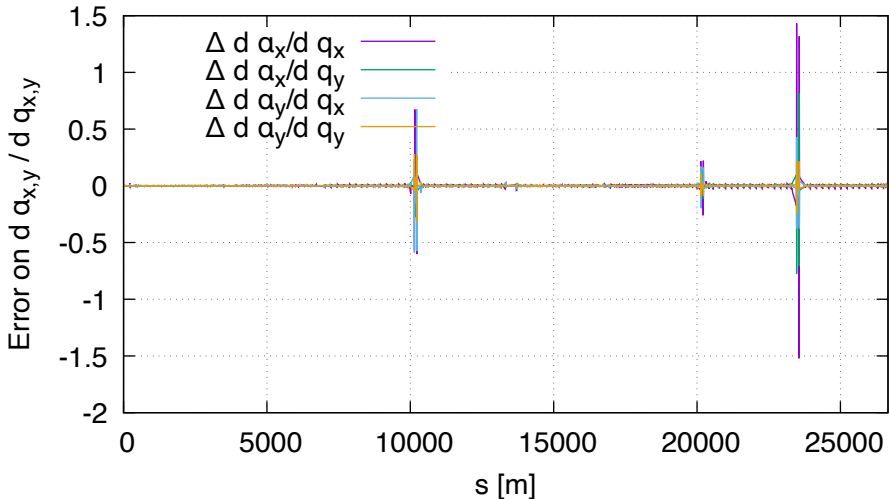
Sensitivity error of alpha FD vs DA (lhcb1, order 1)
