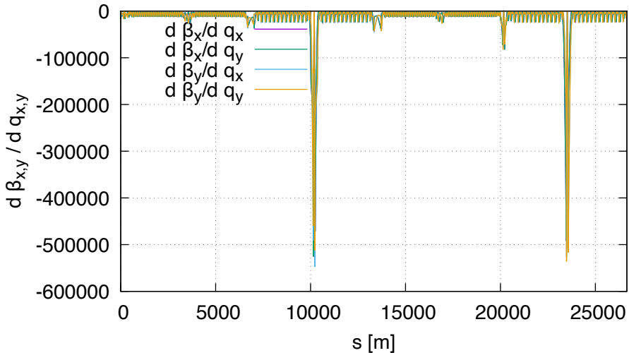
Sensitivity of beta FD (lhcb1, order 2)
