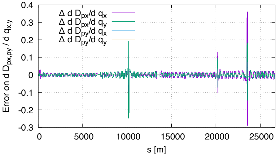
Sensitivity error of dispp FD vs DA (lhcb1, order 2)
