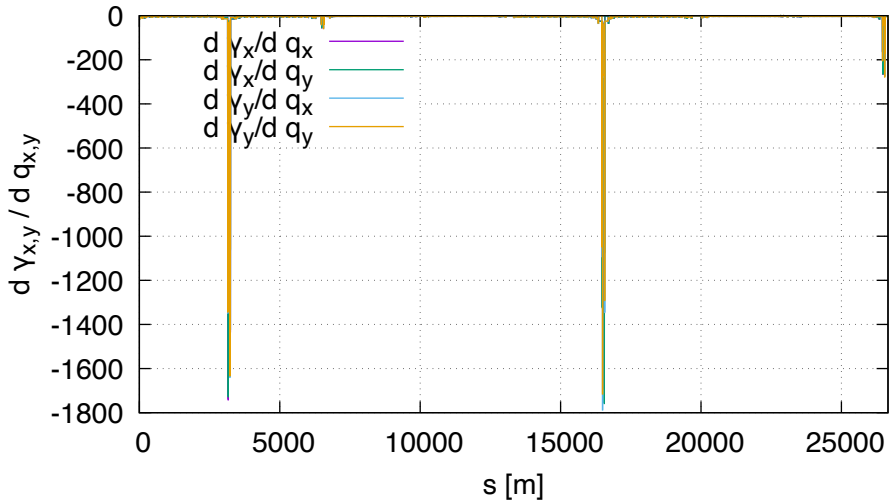
Sensitivity of gamma FD (lhcb2, order 2)
