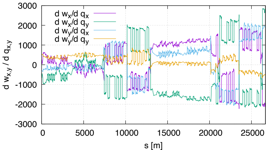
Sensitivity of w FD (lhcb1, order 1)
