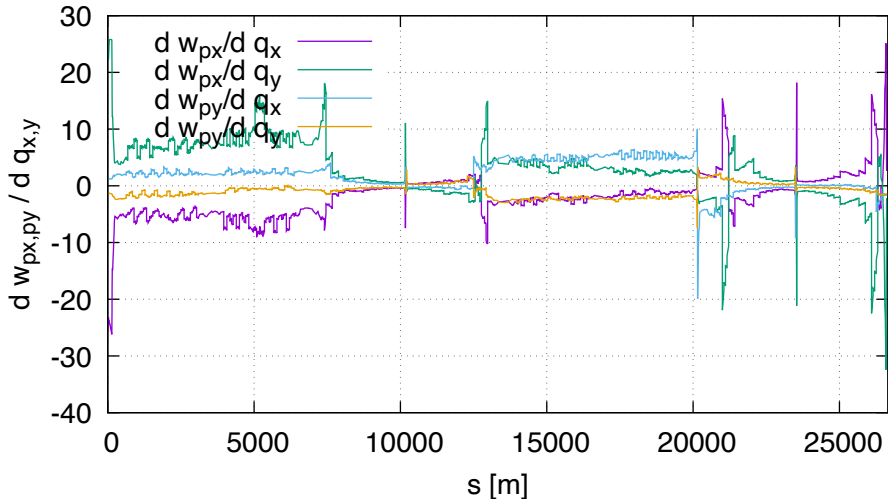
Sensitivity of wp FD (lhcb1, order 1)
