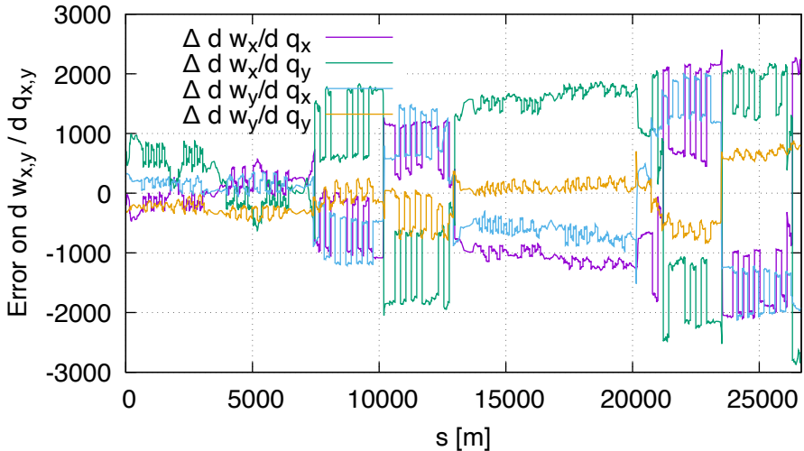
Sensitivity error of w FD vs DA (lhcb1, order 1)
