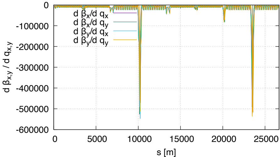
Sensitivity of beta DA (lhcb1, order 2)
