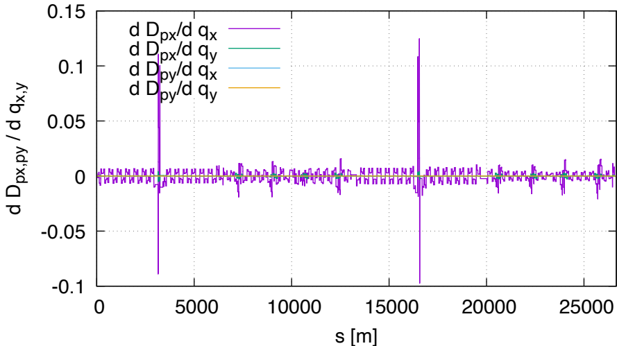
Sensitivity of dispp DA (lhcb2, order 1)
