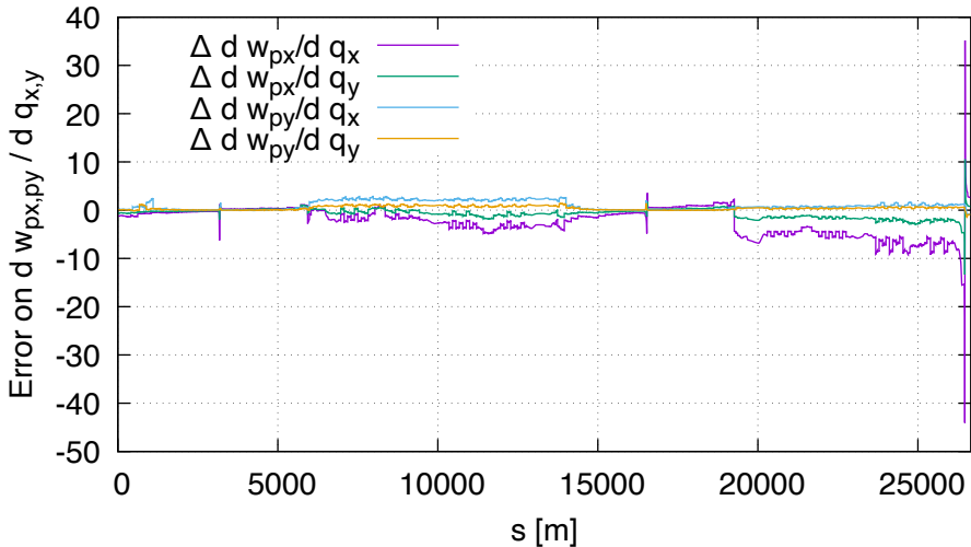
Sensitivity error of wp FD vs DA (lhcb2, order 1)
