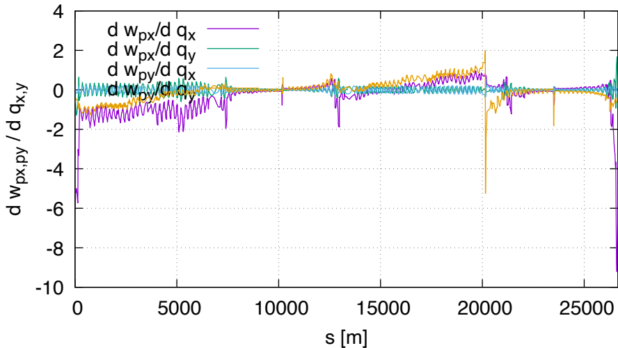
Sensitivity of wp DA (lhcb1, order 1)
