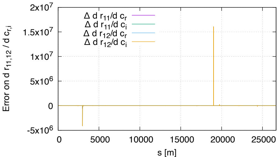
Sensitivity error of R11,R12 FD vs DA (lhcb1, order 2)
