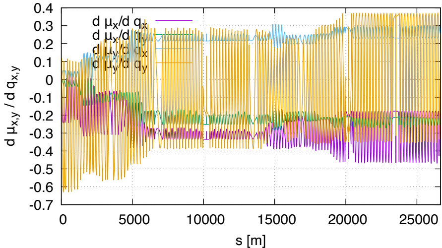
Sensitivity of mu FD (lhcb1, order 2)
