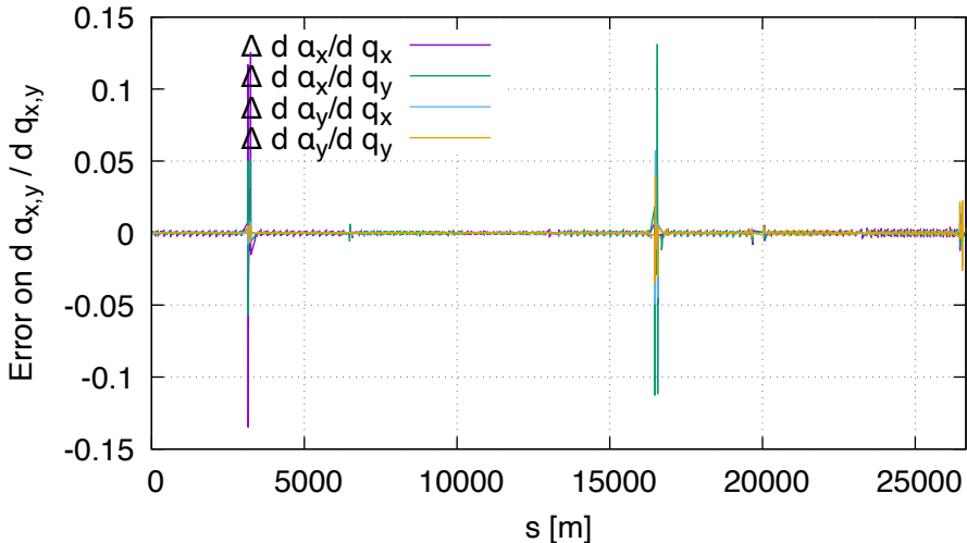
Sensitivity error of alf FD vs DA (lhcb2, order 1)
