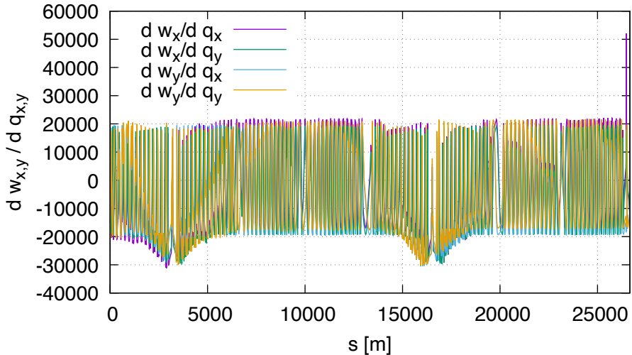
Sensitivity of w DA (lhcb2, order 2)
