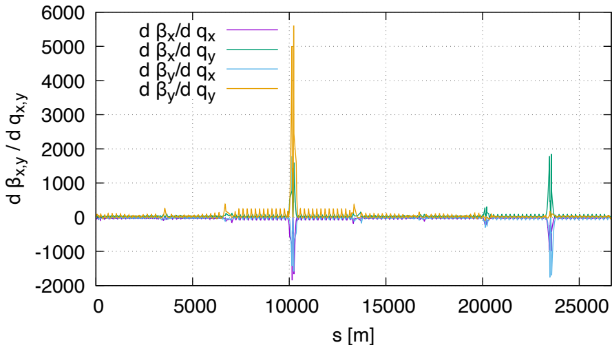
Sensitivity of beta FD (lhcb1, order 1)
