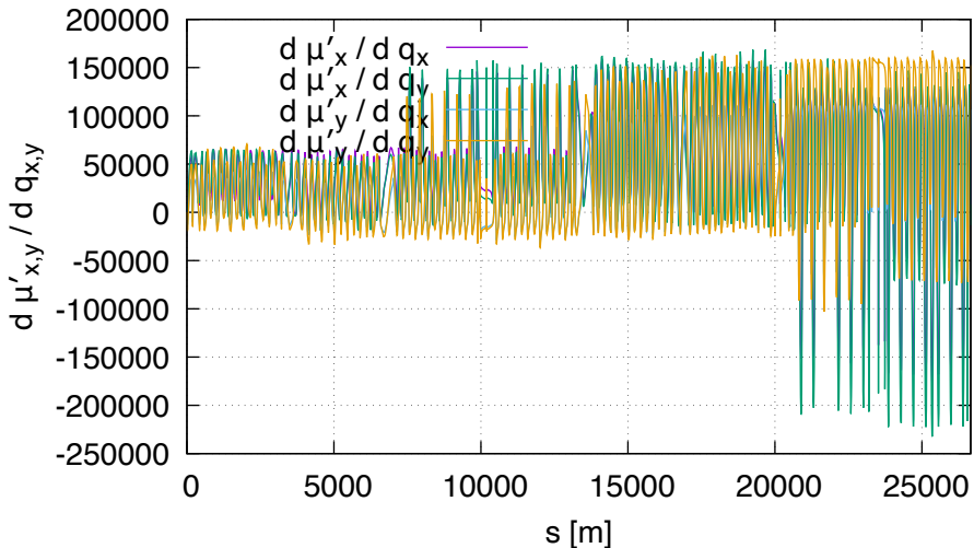
Sensitivity of dmu FD (lhcb1, order 2)
