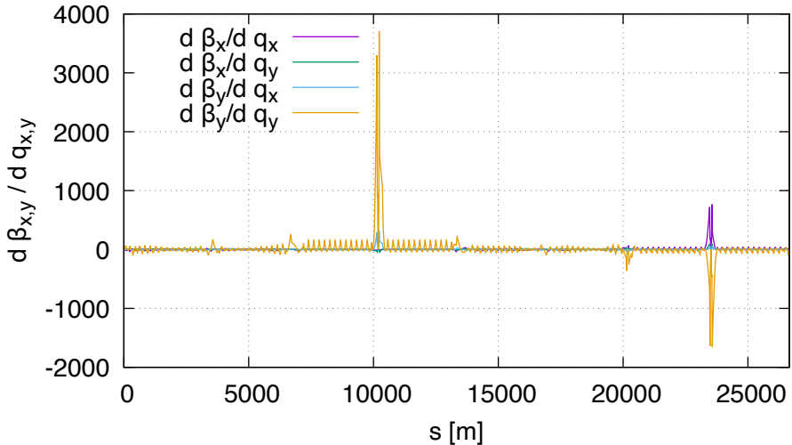
Sensitivity of bet FD (lhcb1, order 1)
