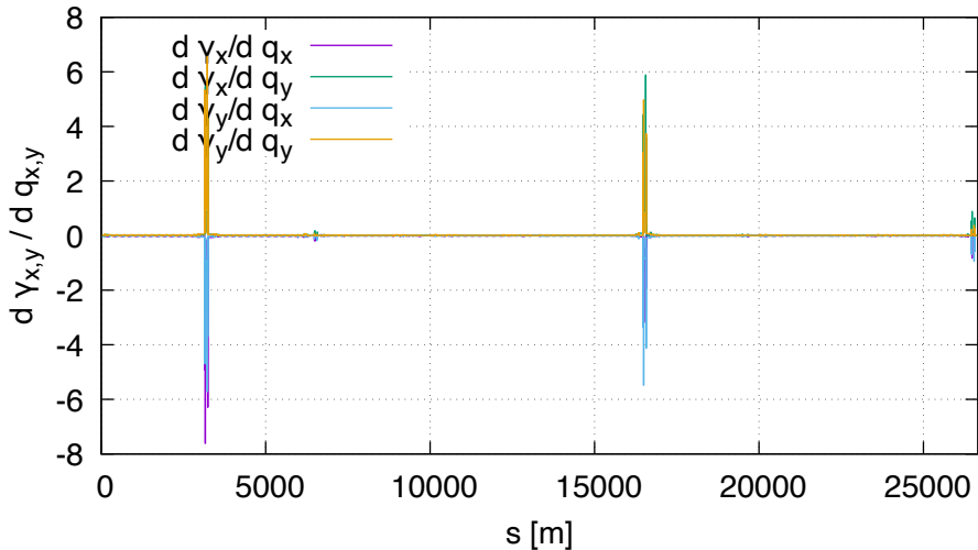
Sensitivity of gamma DA (lhcb2, order 1)
