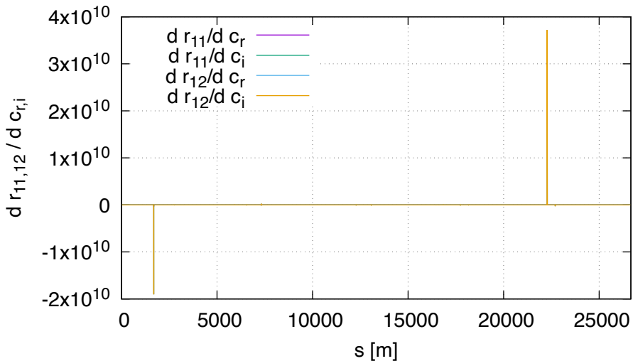
Sensitivity of R11,R12 DA (lhcb2, order 2)
