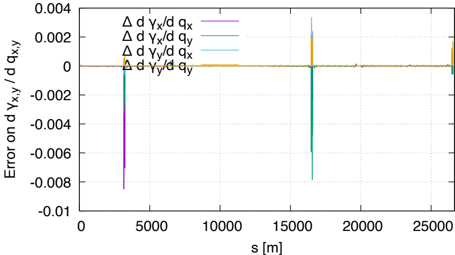
Sensitivity error of gamma FD vs DA (lhcb2, order 1)
