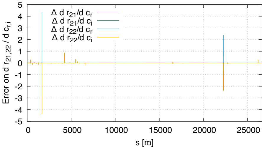
Sensitivity error of R21,R22 FD vs DA (lhcb2, order 1)
