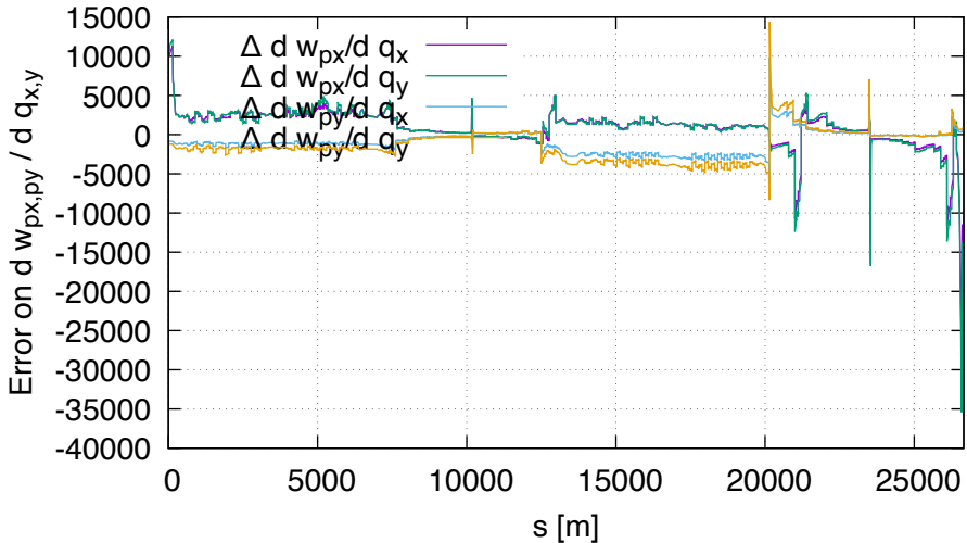
Sensitivity error of wp FD vs DA (lhcb1, order 2)
