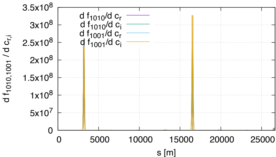
Sensitivity of f1010,f1001 DA (lhcb2, order 1)
