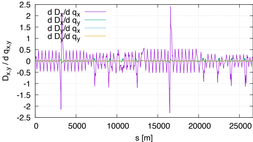
Sensitivity of disp FD (lhcb2, order 1)
