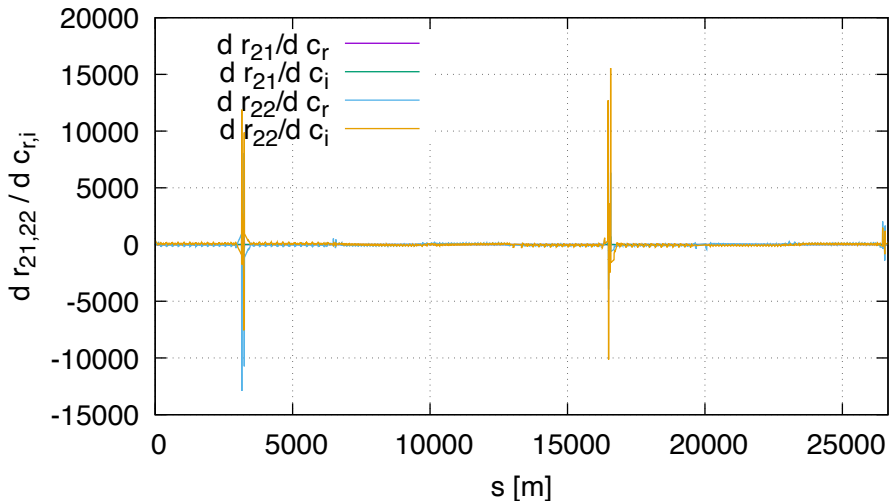
Sensitivity of R21,R22 FD (lhcb2, order 1)
