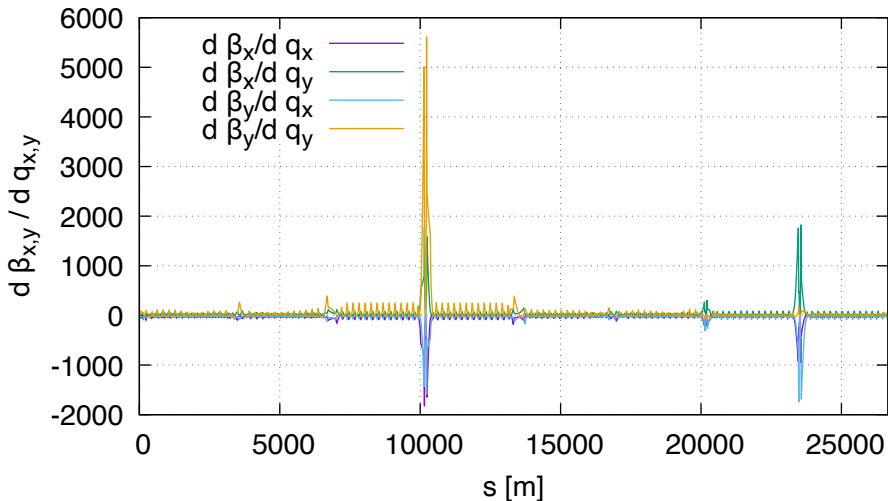
Sensitivity of beta DA (lhcb1, order 1)
