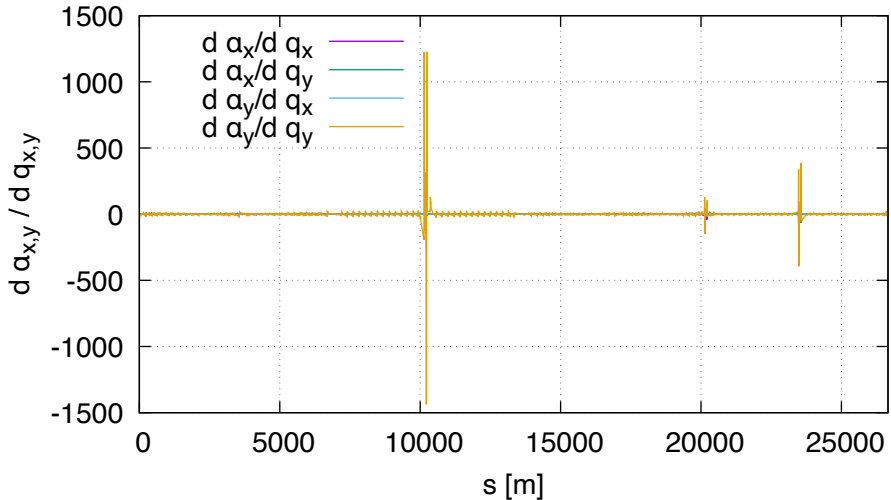
Sensitivity of alf FD (lhcb1, order 2)
