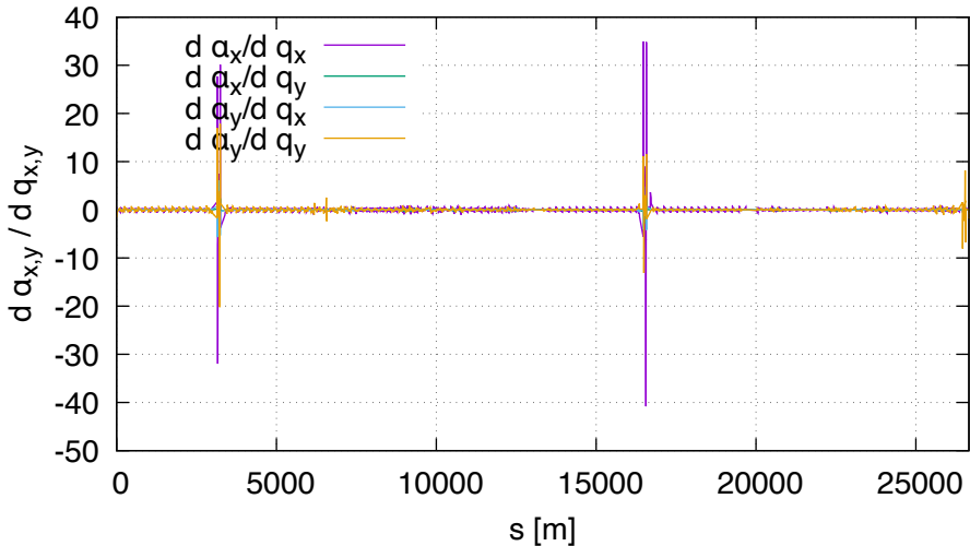
Sensitivity of alf FD (lhcb2, order 1)
