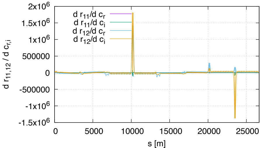
Sensitivity of R11,R12 FD (lhcb1, order 2)
