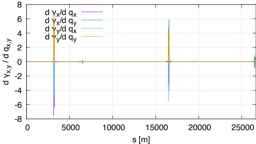
Sensitivity of gamma FD (lhcb2, order 1)
