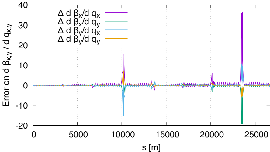
Sensitivity error of bet FD vs DA (lhcb1, order 1)
