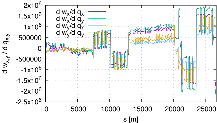
Sensitivity of w FD (lhcb1, order 2)
