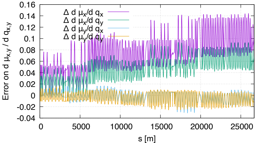
Sensitivity error of mu FD vs DA (lhcb2, order 2)
