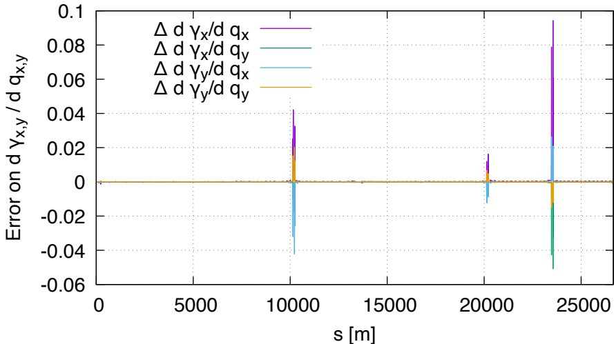
Sensitivity error of gamma FD vs DA (lhcb1, order 1)
