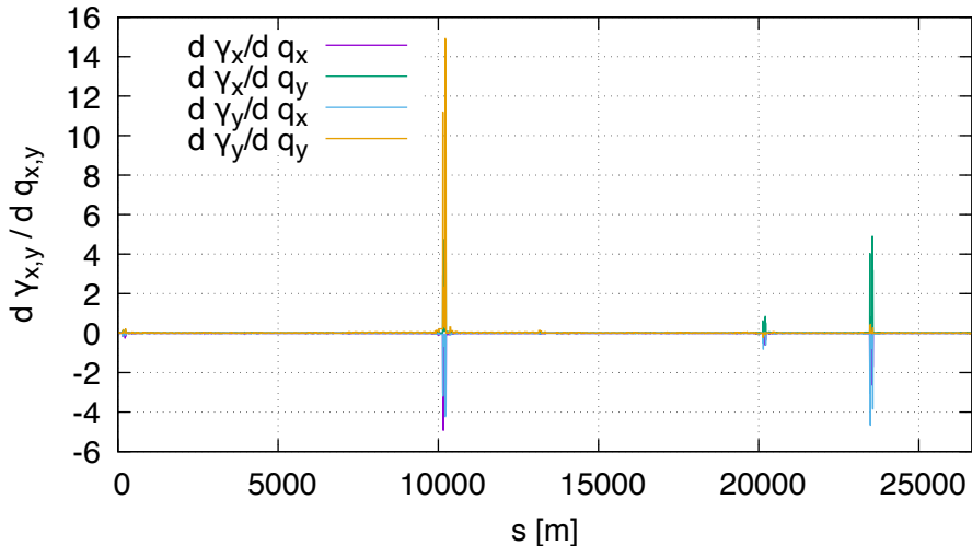
Sensitivity of gamma FD (lhcb1, order 1)
