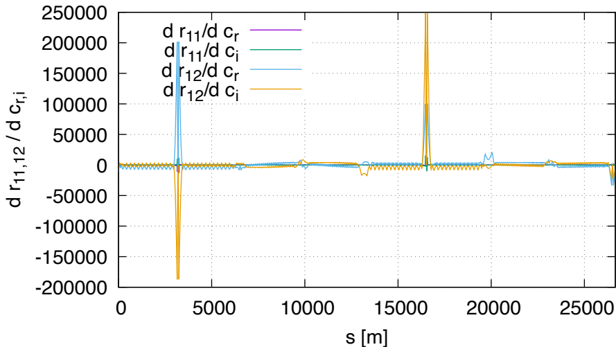
Sensitivity of R11,R12 DA (lhcb2, order 1)
