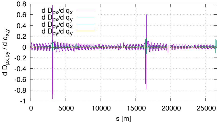
Sensitivity of dispp FD (lhcb2, order 2)
