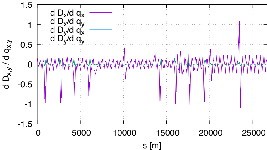
Sensitivity of disp DA (lhcb1, order 1)
