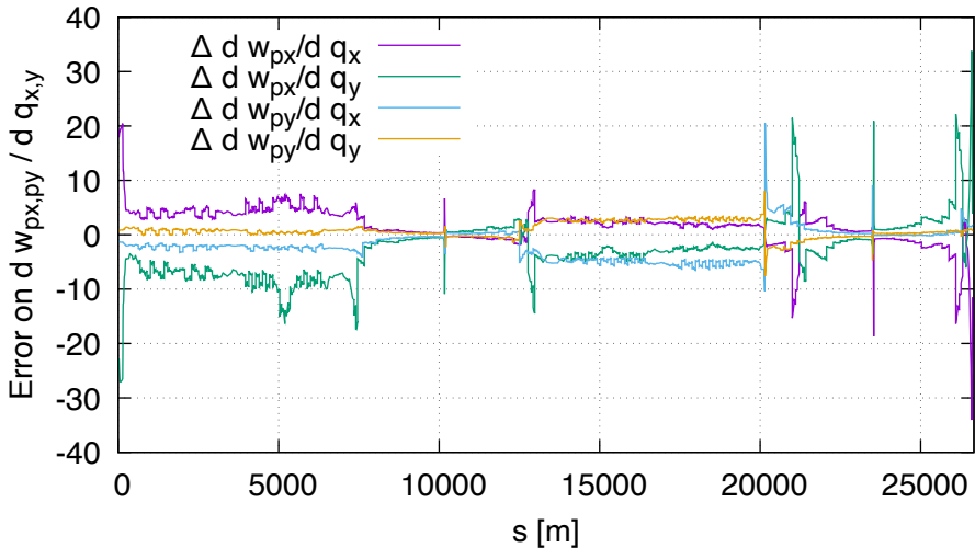
Sensitivity error of wp FD vs DA (lhcb1, order 1)
