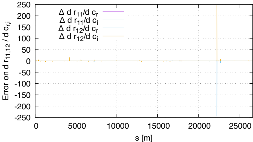
Sensitivity error of R11,R12 FD vs DA (lhcb2, order 1)
