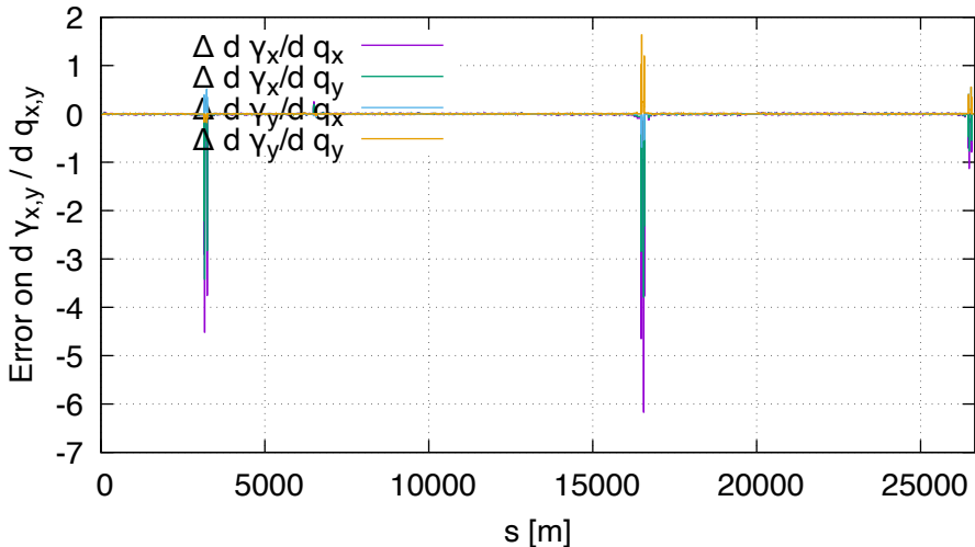
Sensitivity error of gamma FD vs DA (lhcb2, order 2)
