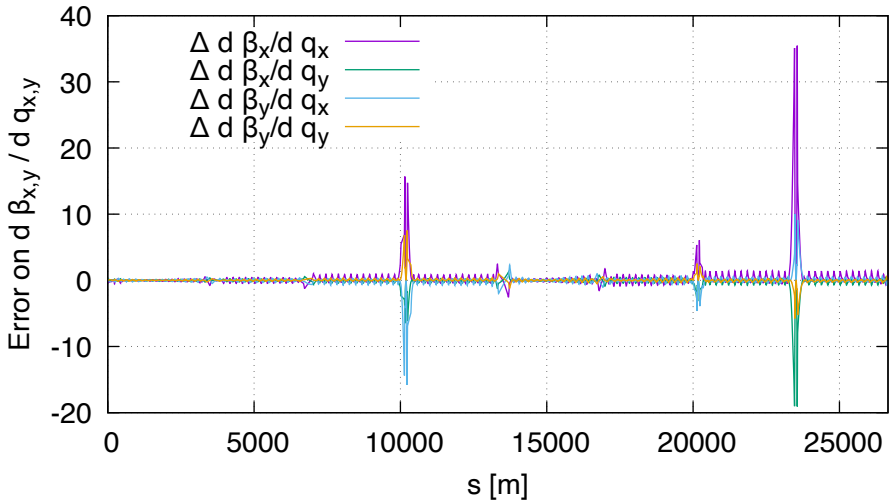
Sensitivity error of beta FD vs DA (lhcb1, order 1)
