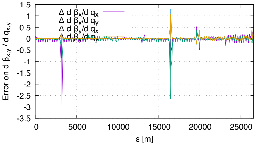
Sensitivity error of beta FD vs DA (lhcb2, order 1)
