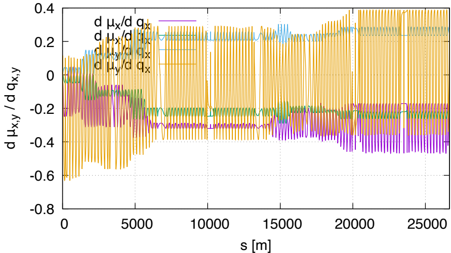
Sensitivity of mu DA (lhcb1, order 2)
