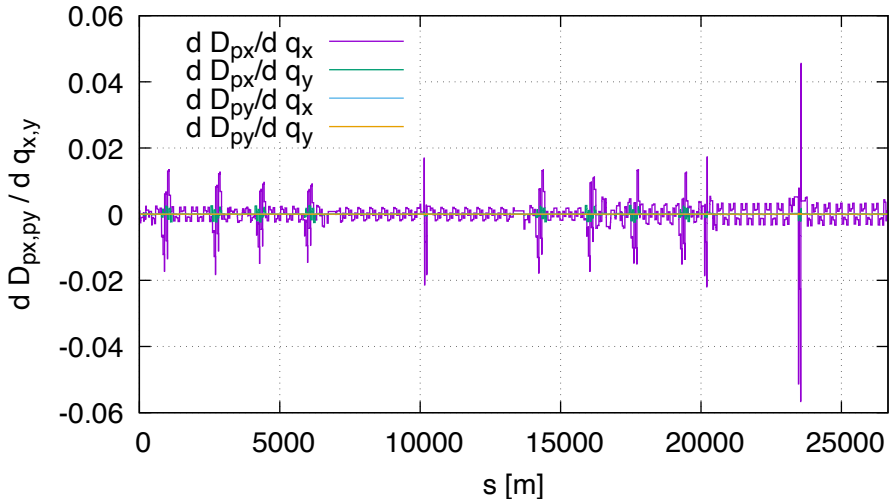
Sensitivity of dispp DA (lhcb1, order 1)
