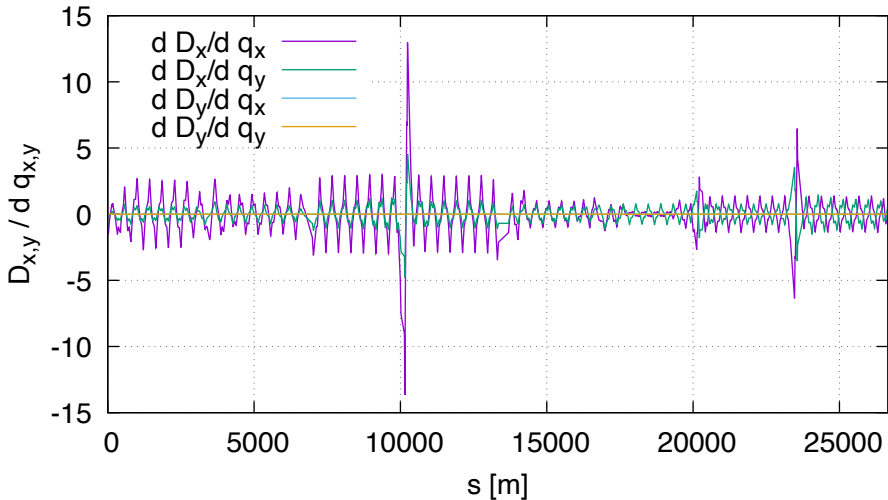
Sensitivity of disp FD (lhcb1, order 2)
