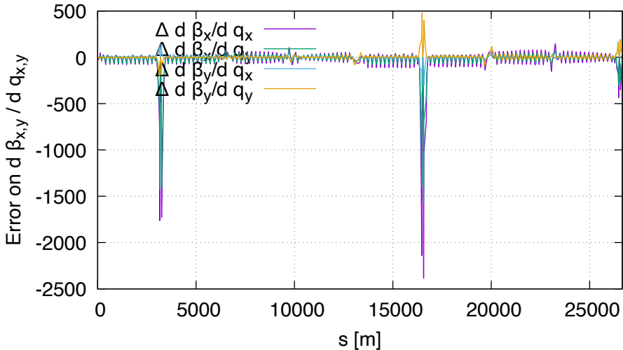
Sensitivity error of bet FD vs DA (lhcb2, order 2)
