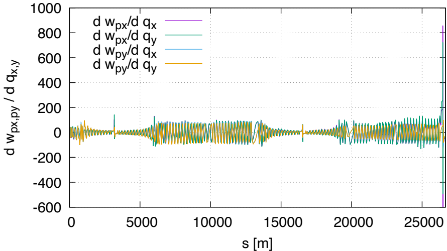
Sensitivity of wp DA (lhcb2, order 2)
