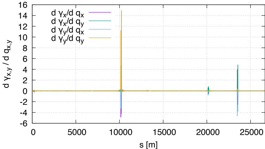
Sensitivity of gamma DA (lhcb1, order 1)
