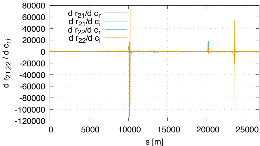
Sensitivity of R21,R22 FD (lhcb1, order 2)
