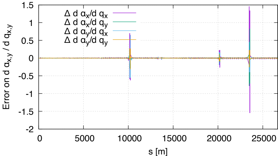
Sensitivity error of alf FD vs DA (lhcb1, order 1)
