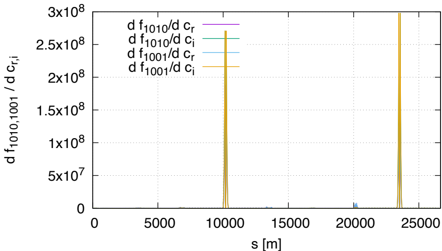
Sensitivity of f1010,f1001 DA (lhcb1, order 1)
