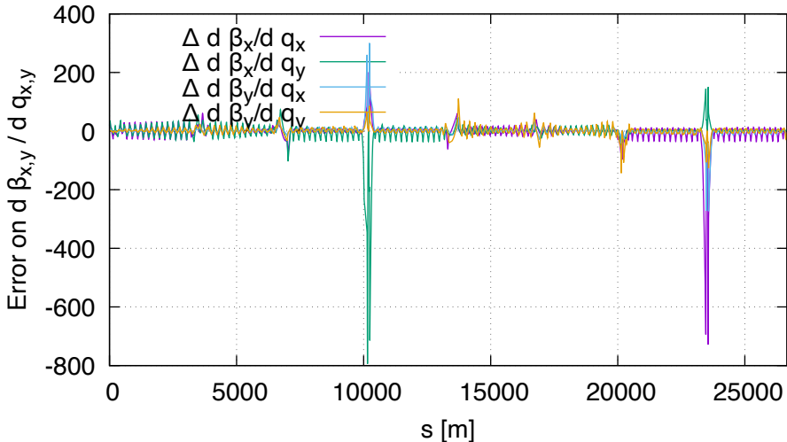
Sensitivity error of beta FD vs DA (lhcb1, order 2)
