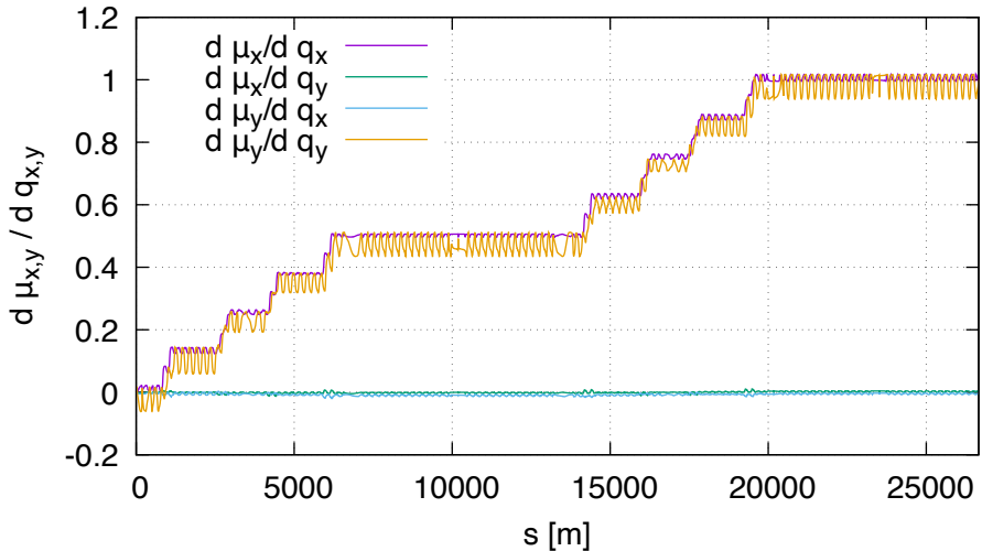
Sensitivity of mu FD (lhcb1, order 1)
