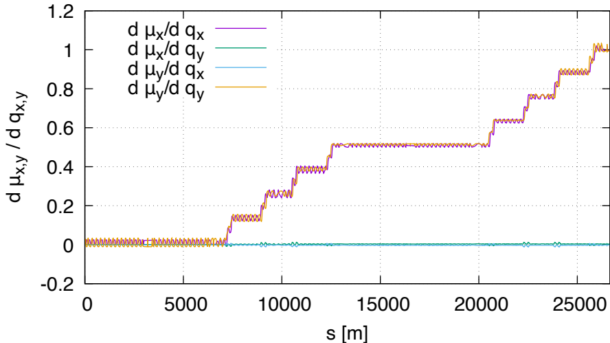
Sensitivity of mu FD (lhcb2, order 1)
