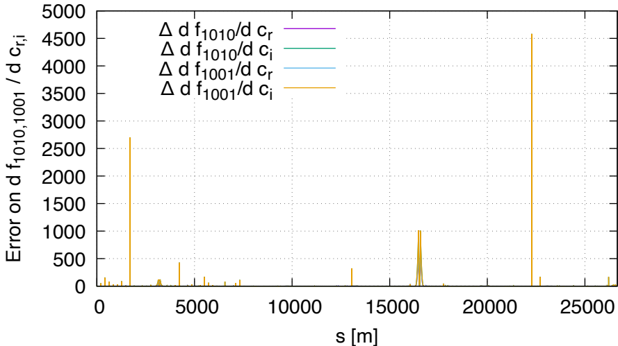
Sensitivity error of f1010,f1001 FD vs DA (lhcb2, order 1)
