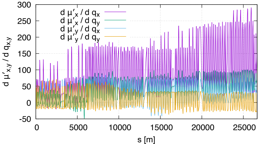
Sensitivity of dm \mu FD (lhcb2, order 1)
