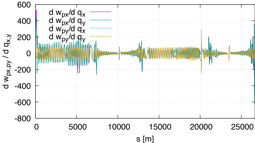
Sensitivity of wp DA (lhcb1, order 2)
