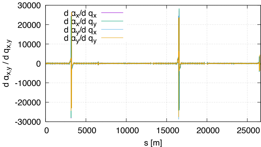
Sensitivity of alpha FD (lhcb2, order 2)
