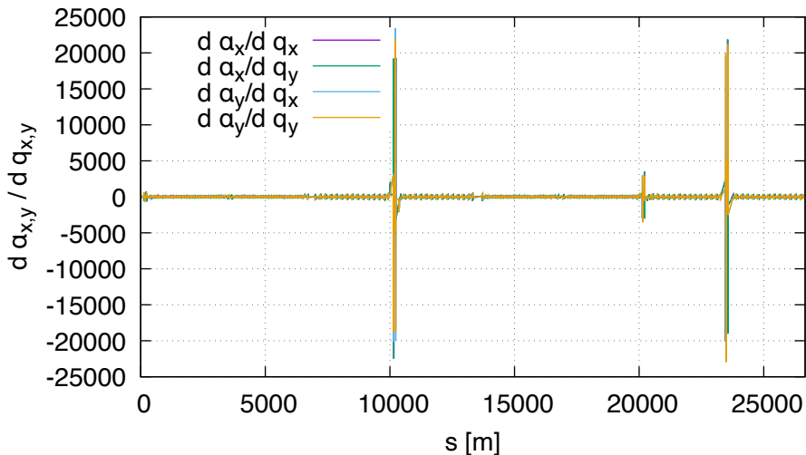
Sensitivity of alpha DA (lhcb1, order 2)
