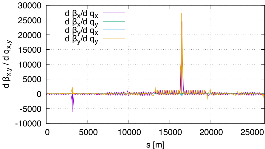
Sensitivity of bet DA (lhcb2, order 2)
