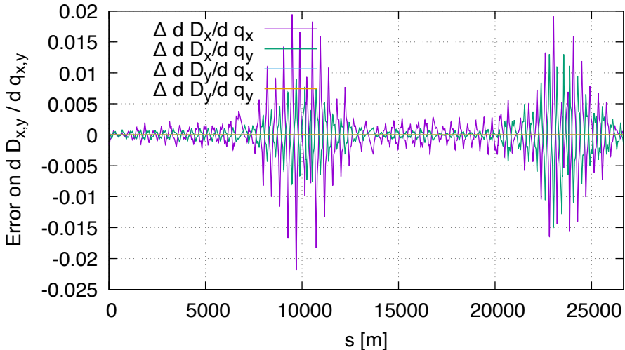
Sensitivity error of disp FD vs DA (lhcb1, order 1)
