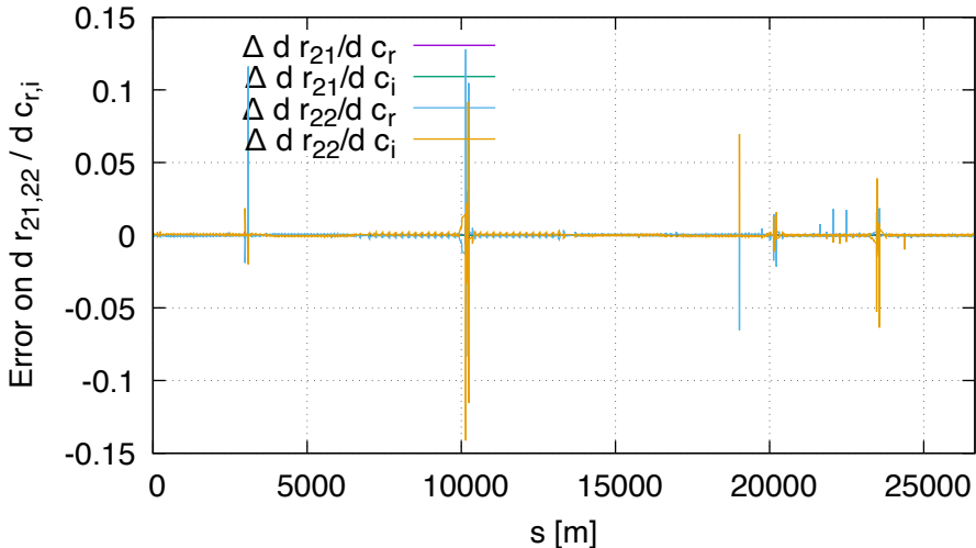
Sensitivity error of R21,R22 FD vs DA (lhcb1, order 1)
