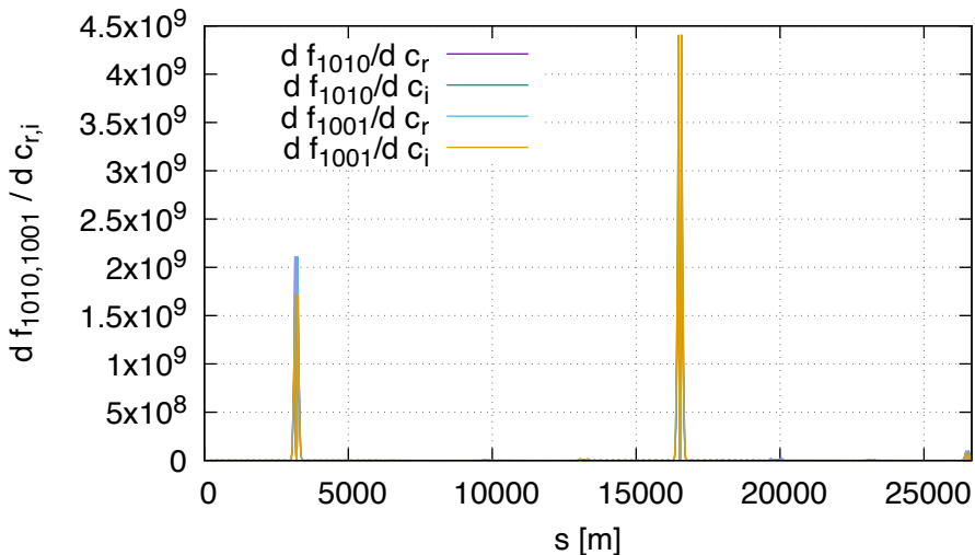
Sensitivity of f1010,f1001 FD (lhcb2, order 2)
