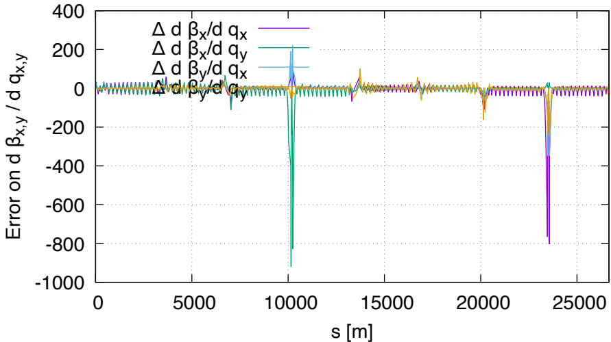
Sensitivity error of bet FD vs DA (lhcb1, order 2)
