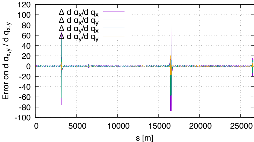
Sensitivity error of alf FD vs DA (lhcb2, order 2)
