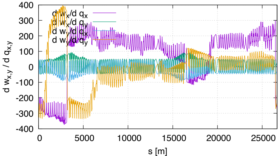
Sensitivity of w DA (lhcb2, order 1)
