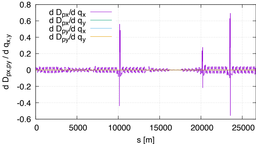
Sensitivity of dispp DA (lhcb1, order 2)
