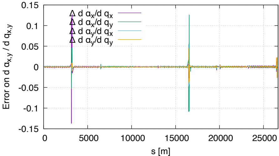
Sensitivity error of alpha FD vs DA (lhcb2, order 1)
