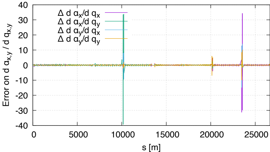
Sensitivity error of alf FD vs DA (lhcb1, order 2)
