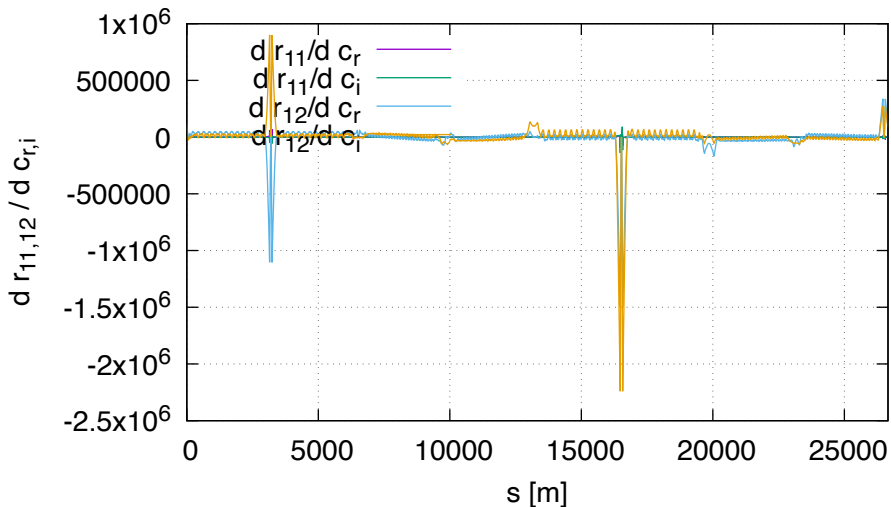
Sensitivity of R11,R12 FD (lhcb2, order 2)
