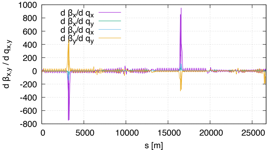
Sensitivity of bet DA (lhcb2, order 1)
