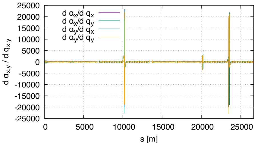
Sensitivity of alpha FD (lhcb1, order 2)
