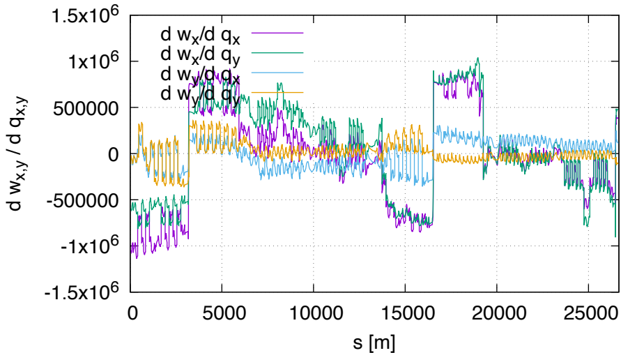
Sensitivity of w FD (lhcb2, order 2)
