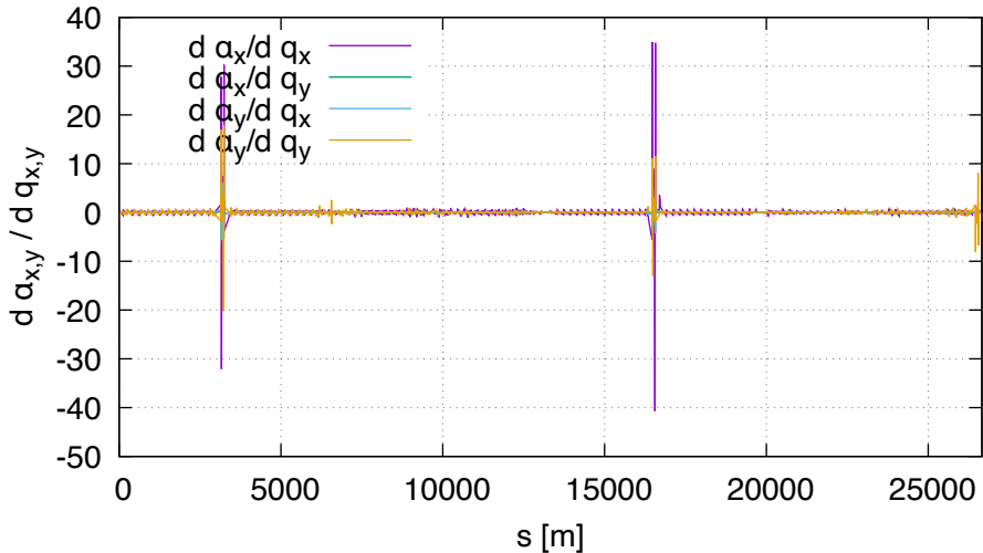
Sensitivity of alf DA (lhcb2, order 1)
