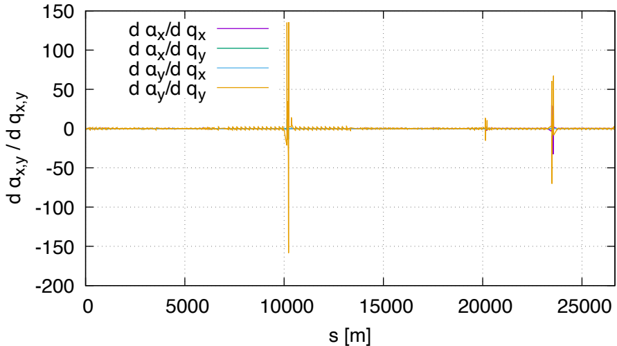
Sensitivity of alf FD (lhcb1, order 1)
