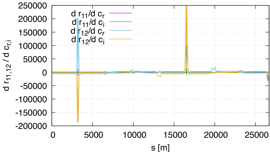
Sensitivity of R11,R12 FD (lhcb2, order 1)
