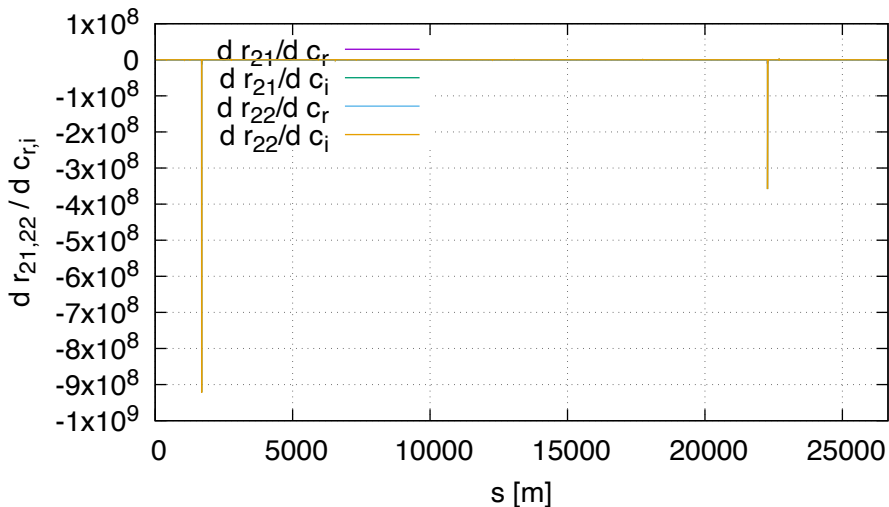
Sensitivity of R21,R22 DA (lhcb2, order 2)
