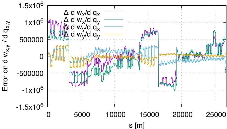
Sensitivity error of w FD vs DA (lhcb2, order 2)
