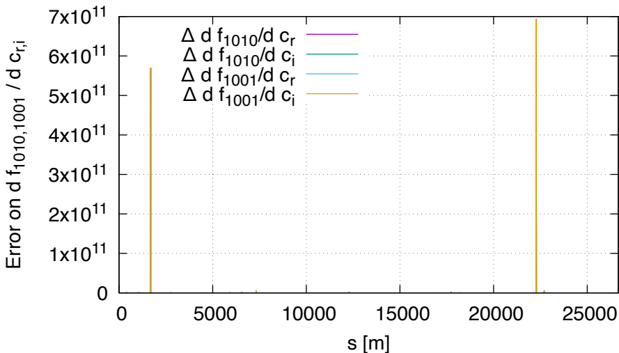
Sensitivity error of f1010,f1001 FD vs DA (lhcb2, order 2)
