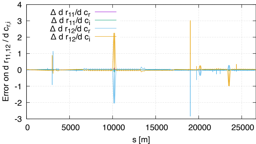
Sensitivity error of R11,R12 FD vs DA (lhcb1, order 1)
