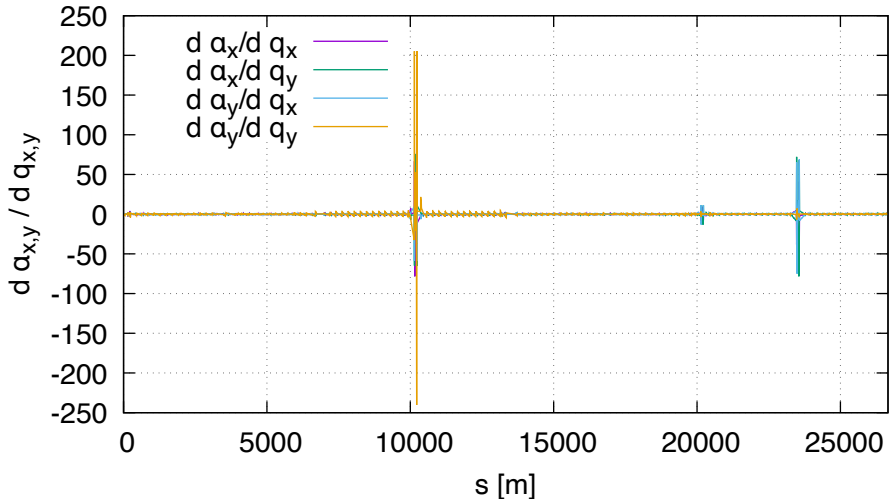
Sensitivity of alpha DA (lhcb1, order 1)
