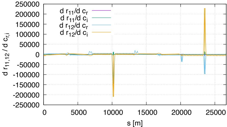
Sensitivity of R11,R12 FD (lhcb1, order 1)
