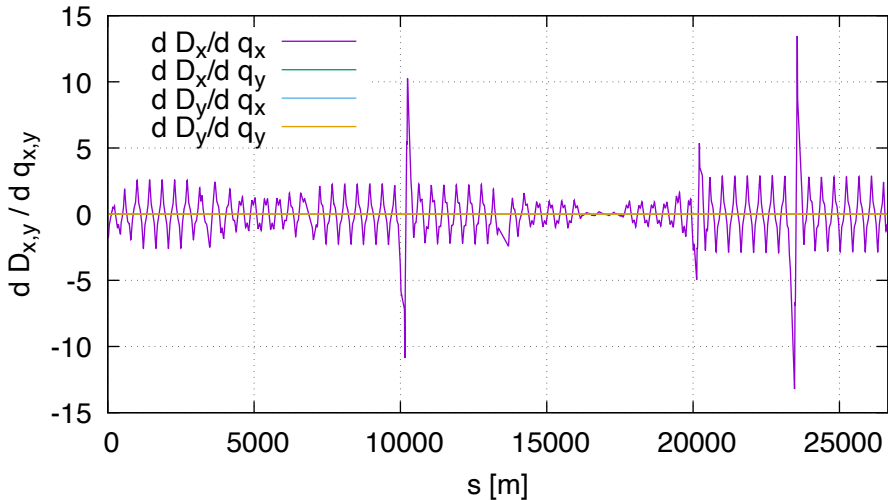
Sensitivity of disp DA (lhcb1, order 2)
