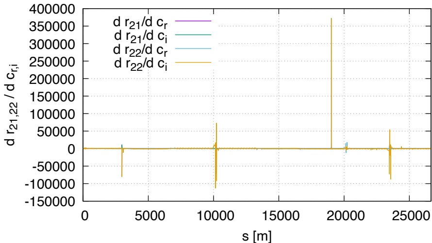
Sensitivity of R21,R22 DA (lhcb1, order 2)
