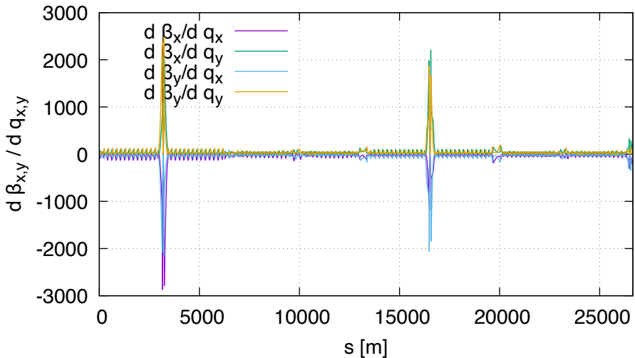
Sensitivity of beta DA (lhcb2, order 1)
