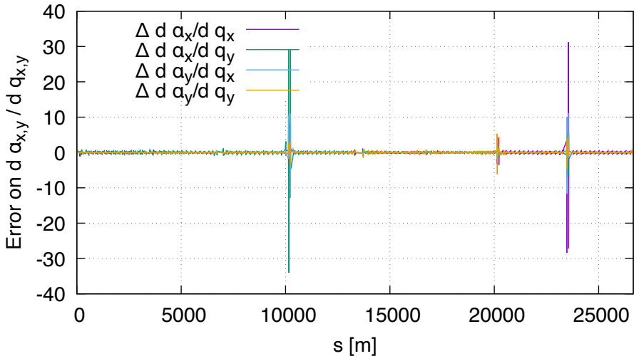
Sensitivity error of alpha FD vs DA (lhcb1, order 2)
