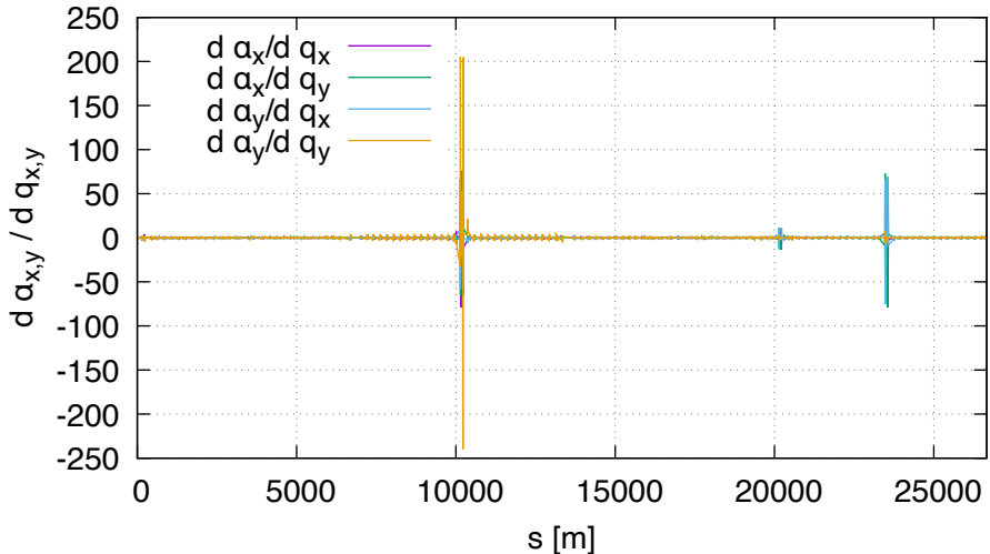
Sensitivity of alpha FD (lhcb1, order 1)
