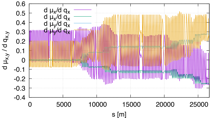
Sensitivity of mu DA (lhcb2, order 2)
