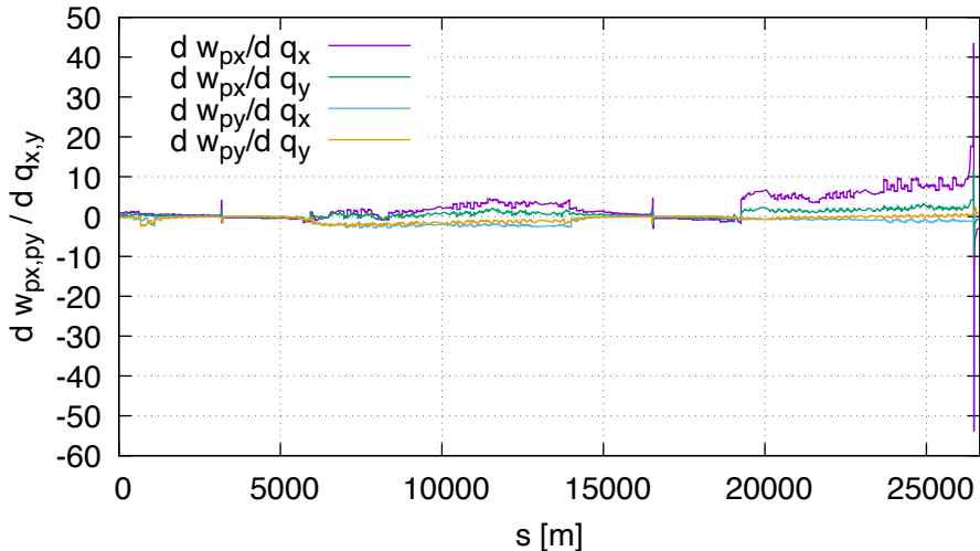
Sensitivity of wp FD (lhcb2, order 1)
