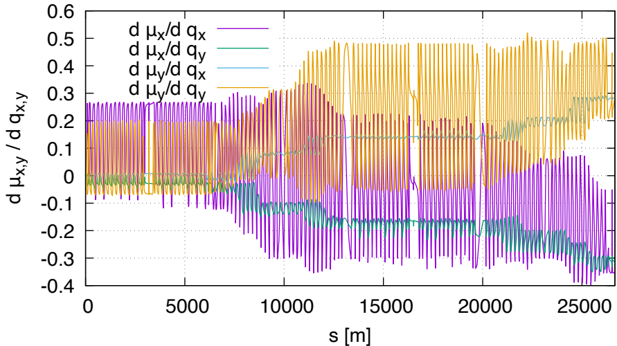
Sensitivity of mu FD (lhcb2, order 2)
