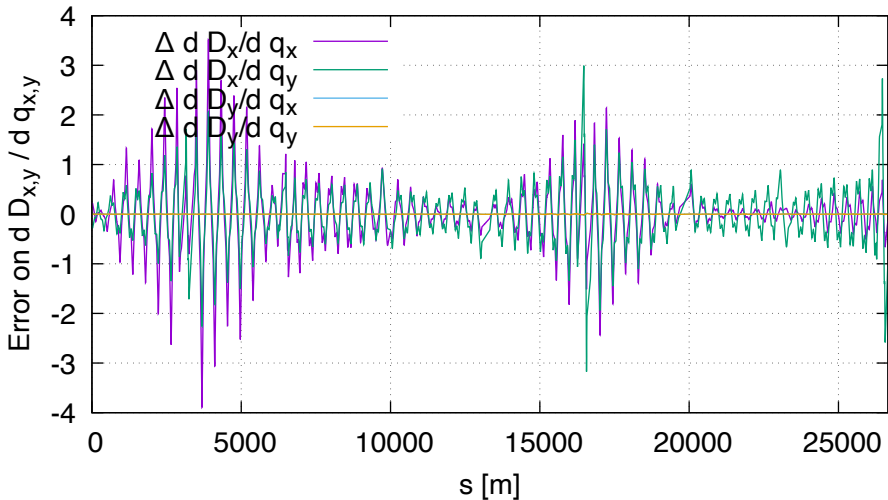
Sensitivity error of disp FD vs DA (lhcb2, order 2)
