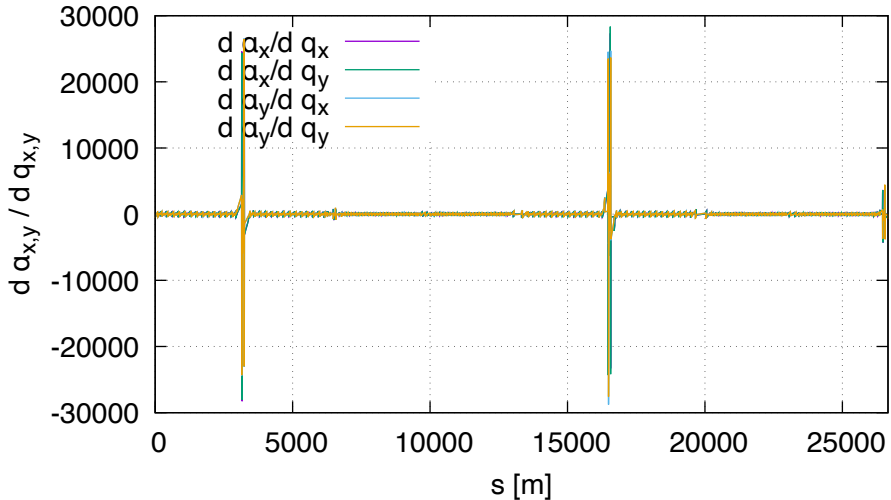
Sensitivity of alpha DA (lhcb2, order 2)
