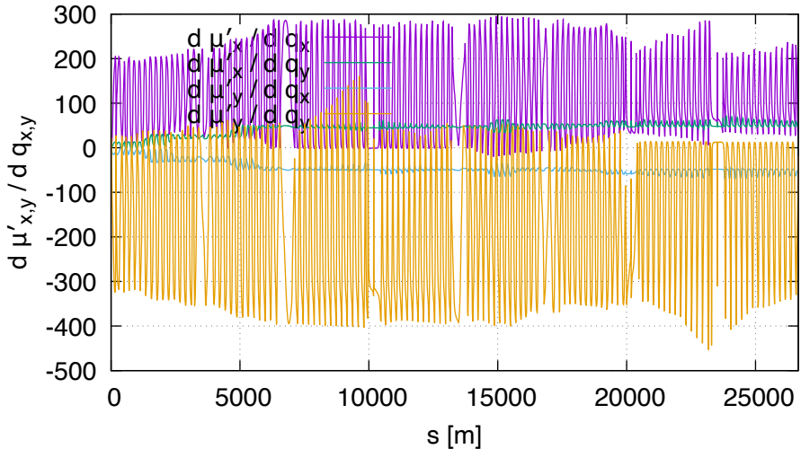
Sensitivity of dm \mu DA (lhcb1, order 2)
