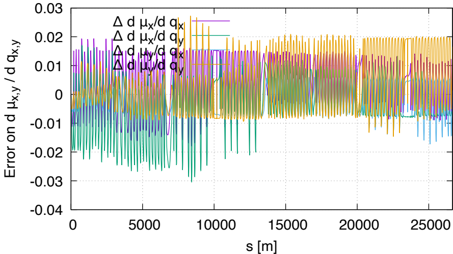
Sensitivity error of mu FD vs DA (lhcb1, order 2)
