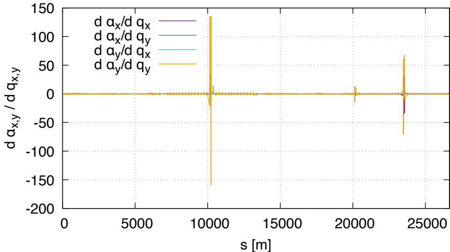
Sensitivity of alf DA (lhcb1, order 1)
