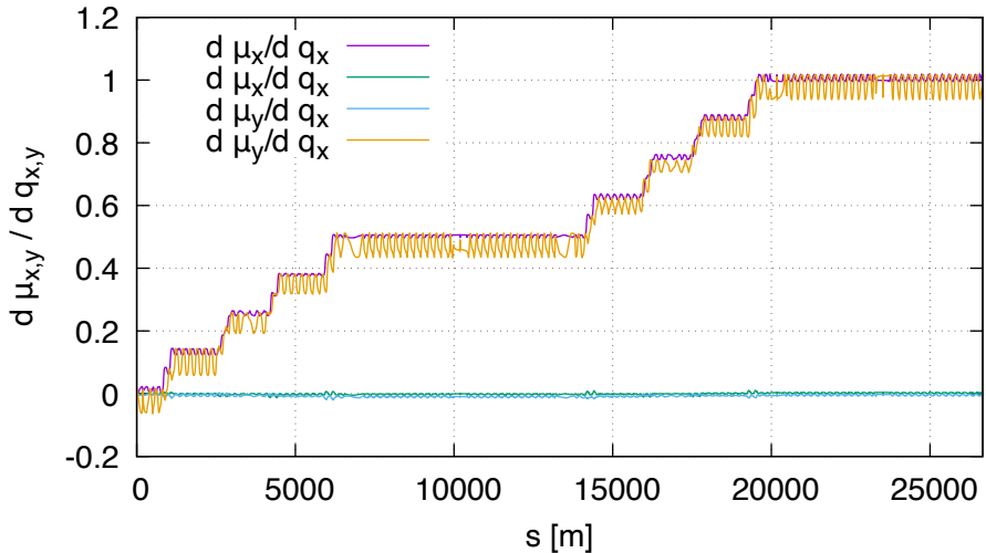
Sensitivity of mu DA (lhcb1, order 1)
