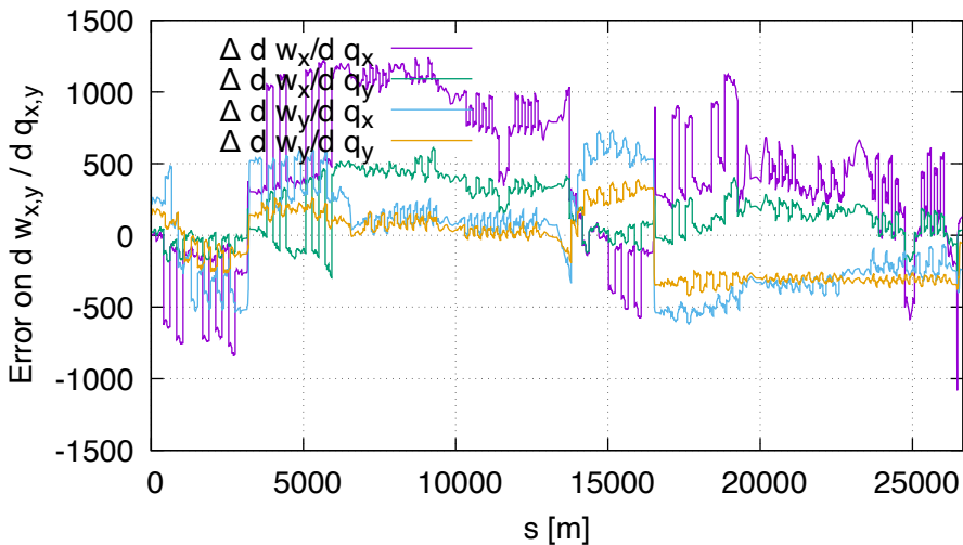
Sensitivity error of w FD vs DA (lhcb2, order 1)
