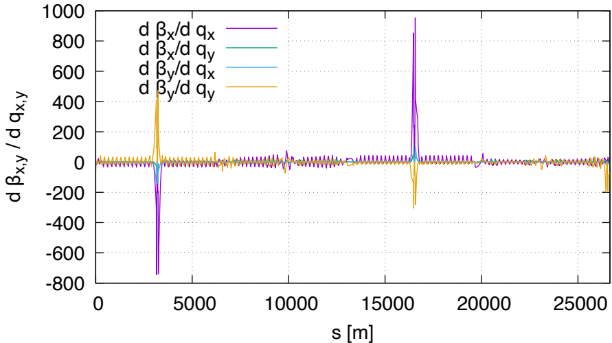
Sensitivity of bet FD (lhcb2, order 1)
