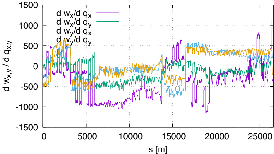
Sensitivity of w FD (lhcb2, order 1)
