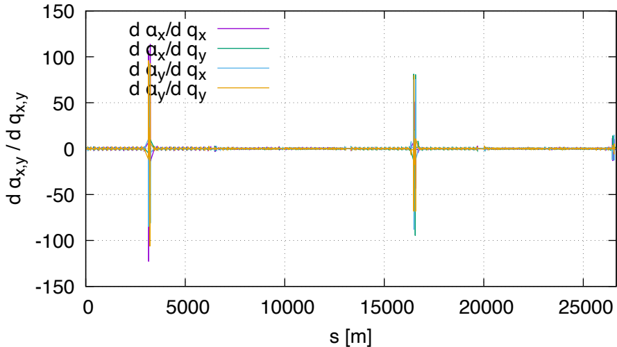
Sensitivity of alpha FD (lhcb2, order 1)
