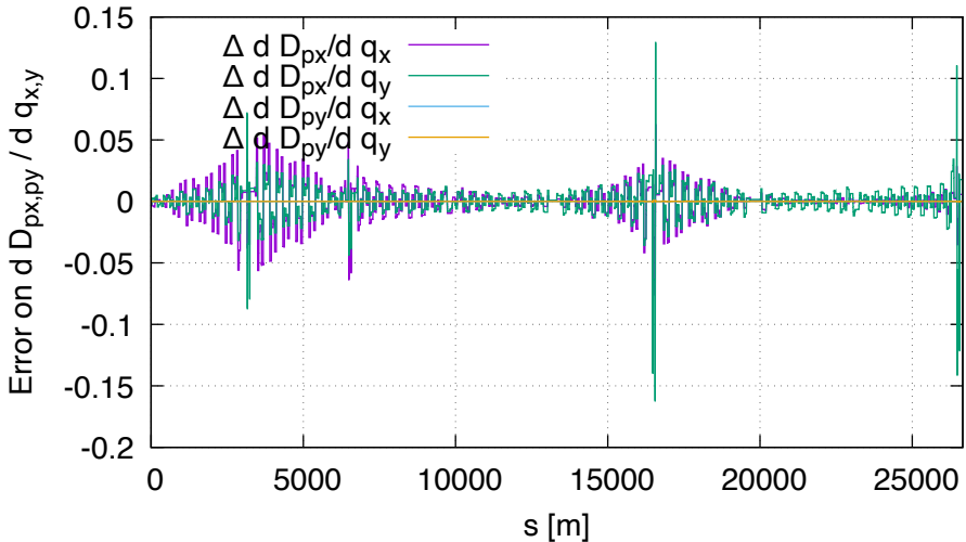
Sensitivity error of dispp FD vs DA (lhcb2, order 2)
