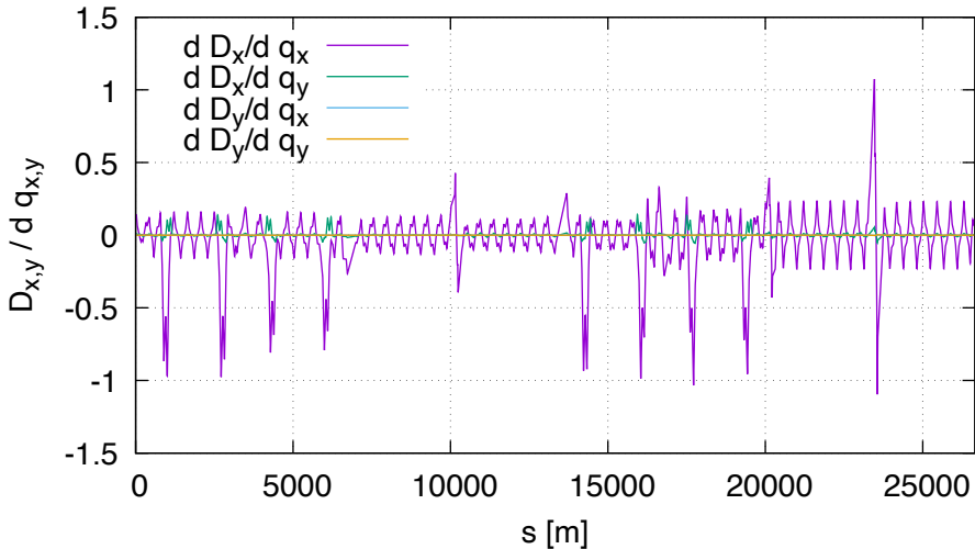
Sensitivity of disp FD (lhcb1, order 1)
