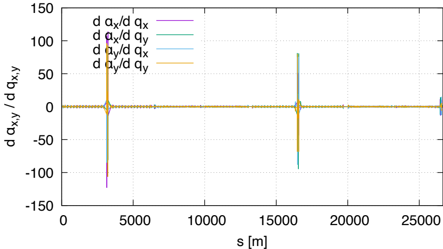
Sensitivity of alpha DA (lhcb2, order 1)
