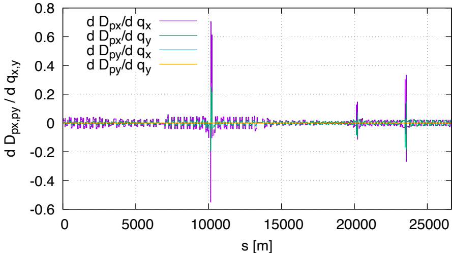
Sensitivity of dispp FD (lhcb1, order 2)
