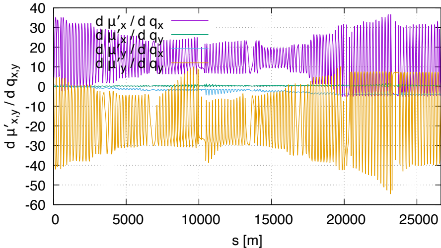
Sensitivity of dm \mu DA (lhcb1, order 1)
