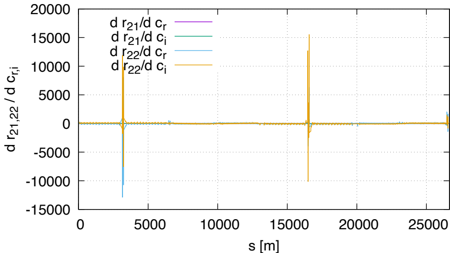
Sensitivity of R21,R22 DA (lhcb2, order 1)
