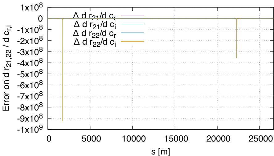
Sensitivity error of R21,R22 FD vs DA (lhcb2, order 2)
