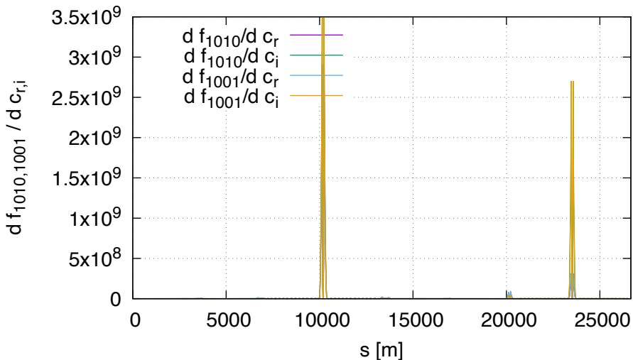
Sensitivity of f1010,f1001 FD (lhcb1, order 2)
