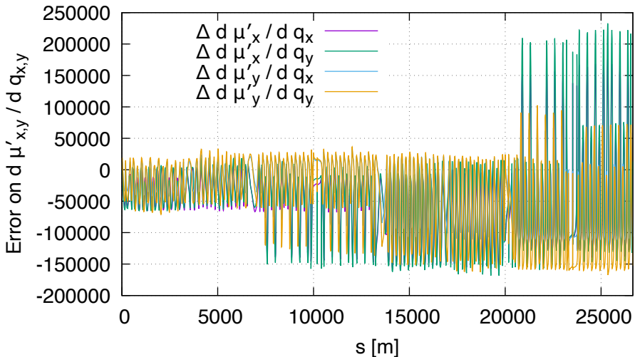
Sensitivity error of dm u FD vs DA (lhcb1, order 2)
