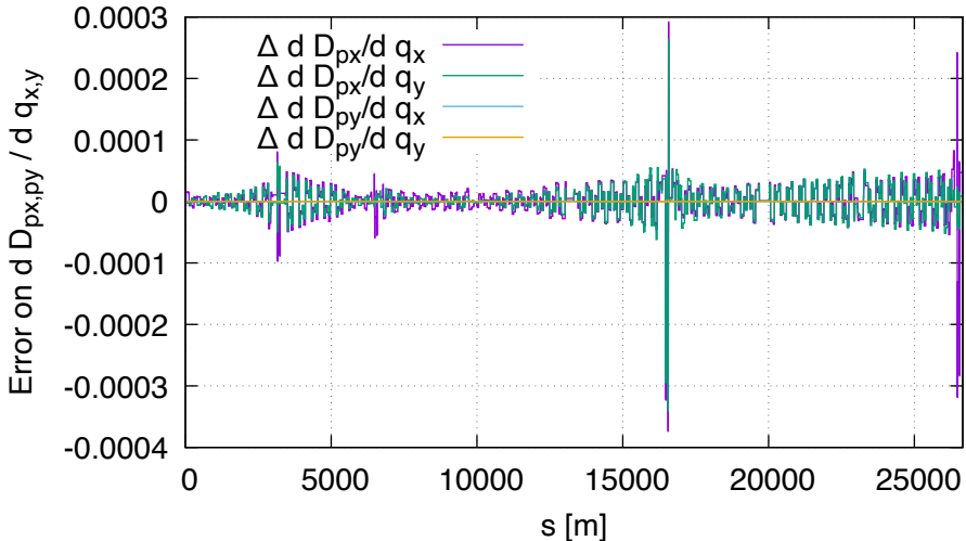
Sensitivity error of dispp FD vs DA (lhcb2, order 1)
