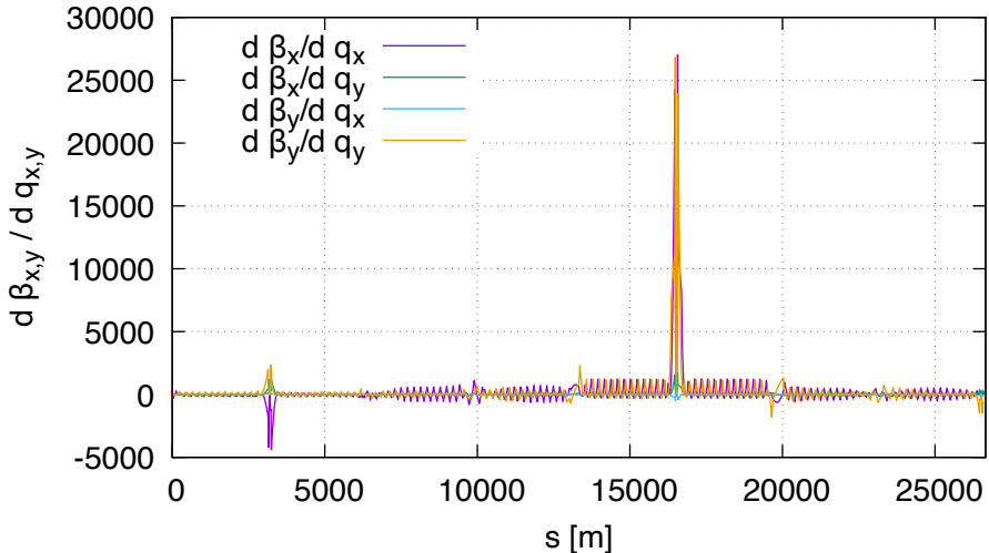
Sensitivity of bet FD (lhcb2, order 2)
