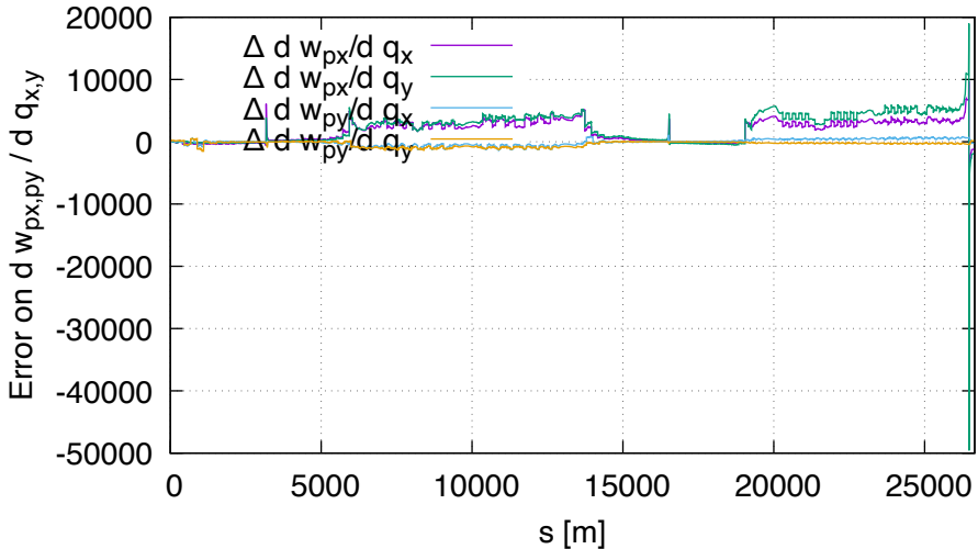
Sensitivity error of wp FD vs DA (lhcb2, order 2)
