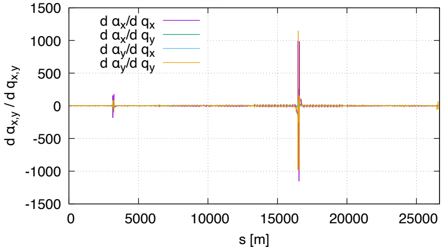
Sensitivity of alf FD (lhcb2, order 2)
