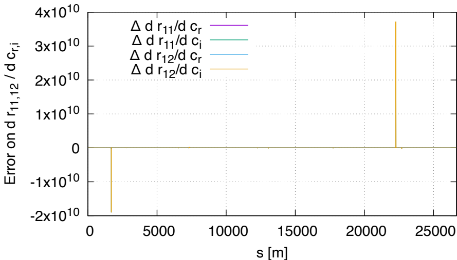
Sensitivity error of R11,R12 FD vs DA (lhcb2, order 2)
