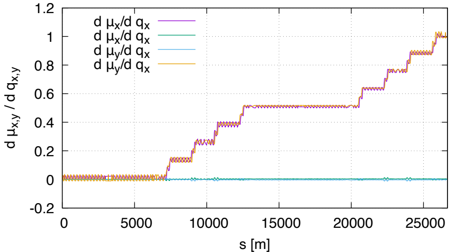
Sensitivity of mu DA (lhcb2, order 1)
