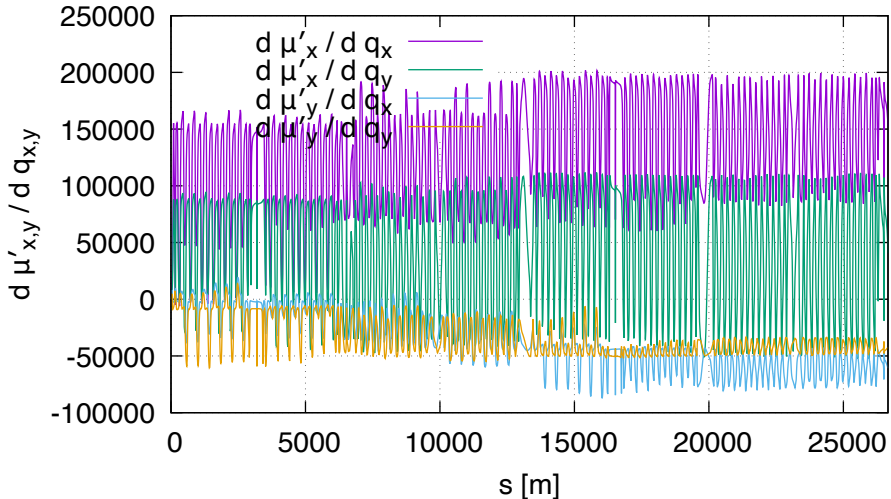
Sensitivity of dm \mu FD (lhcb2, order 2)
