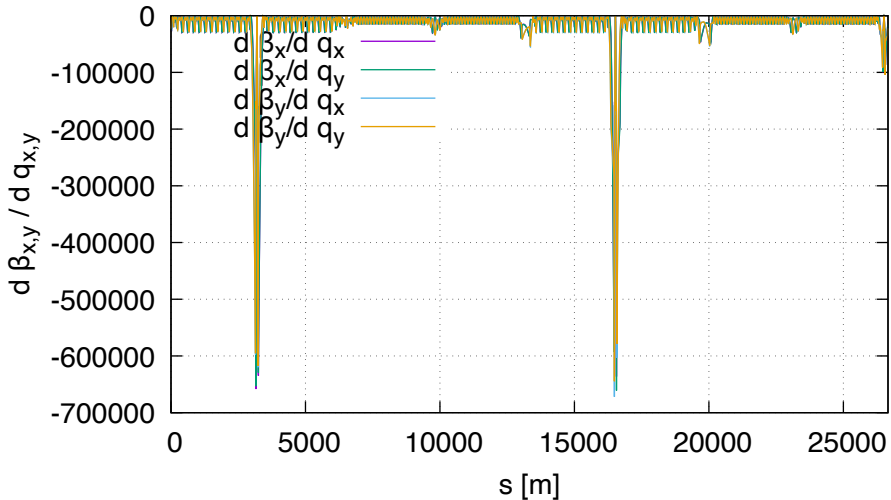
Sensitivity of beta FD (lhcb2, order 2)
