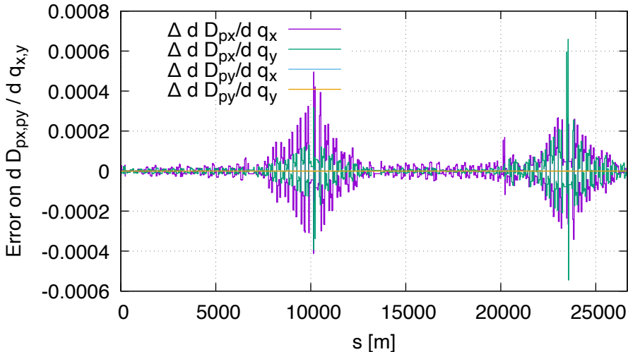
Sensitivity error of dispp FD vs DA (lhcb1, order 1)
