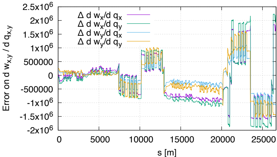
Sensitivity error of w FD vs DA (lhcb1, order 2)
