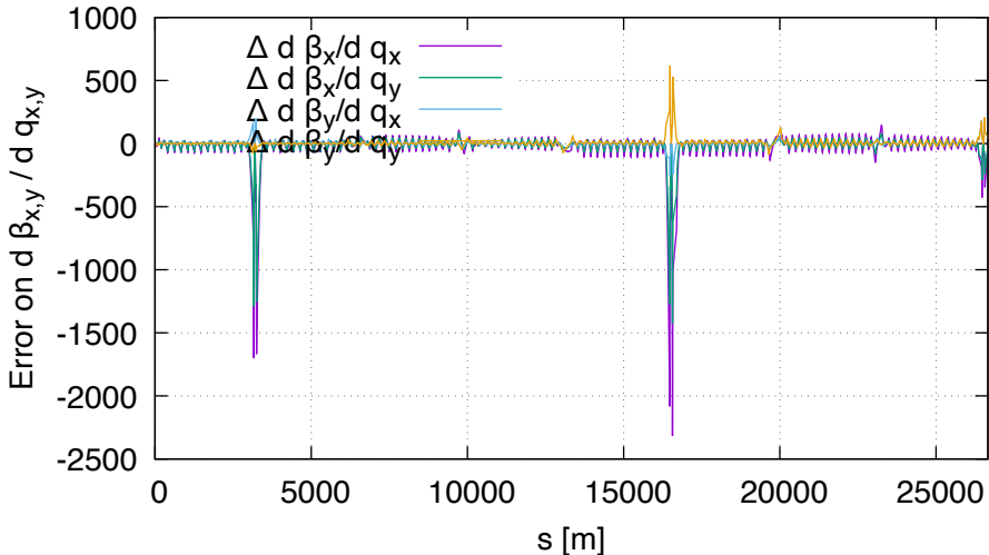
Sensitivity error of beta FD vs DA (lhcb2, order 2)
