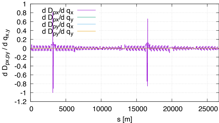
Sensitivity of dispp DA (lhcb2, order 2)
