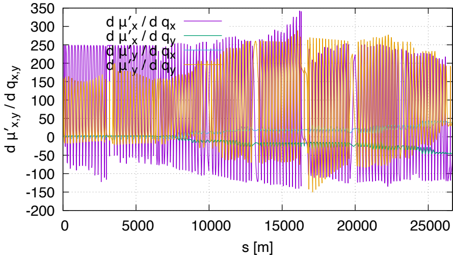
Sensitivity of dm \mu DA (lhcb2, order 2)
