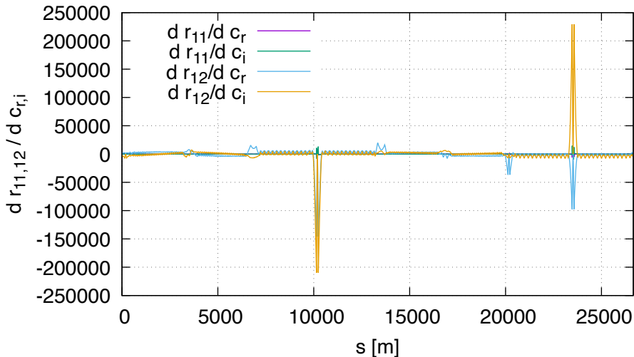
Sensitivity of R11,R12 DA (lhcb1, order 1)
