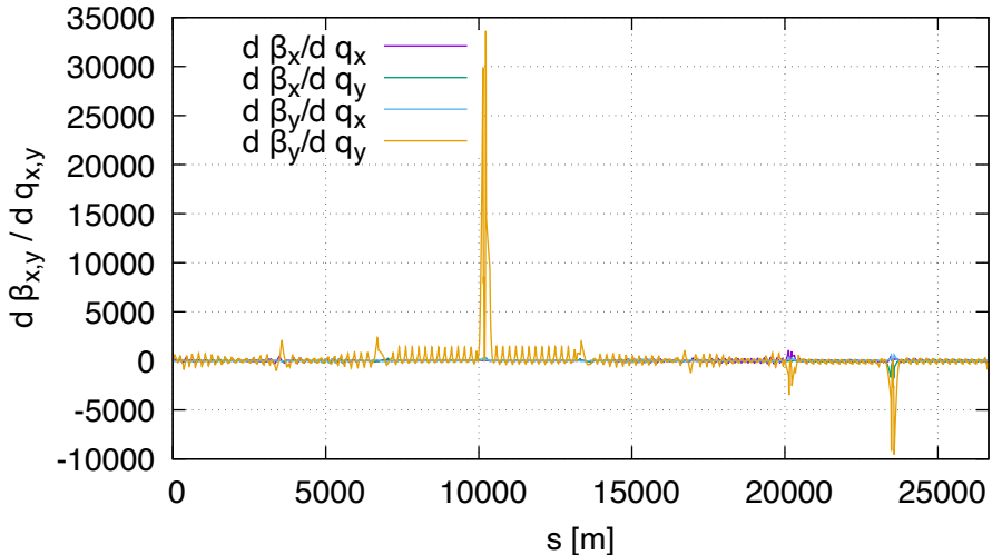
Sensitivity of bet FD (lhcb1, order 2)
