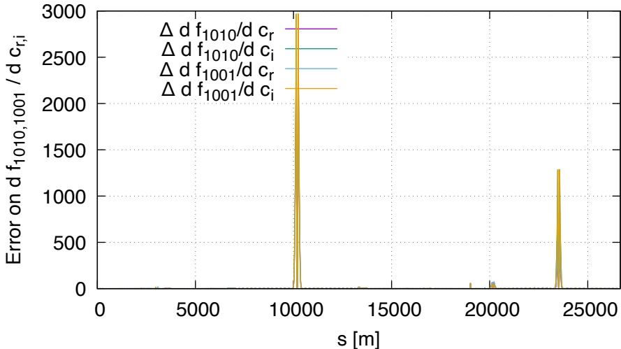
Sensitivity error of f1010,f1001 FD vs DA (lhcb1, order 1)
