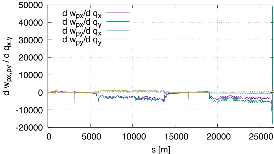
Sensitivity of wp FD (lhcb2, order 2)
