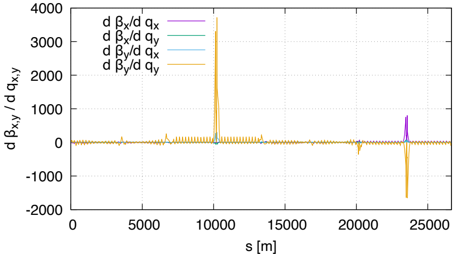
Sensitivity of bet DA (lhcb1, order 1)
