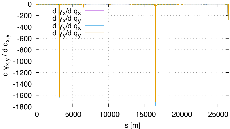
Sensitivity of gamma DA (lhcb2, order 2)
