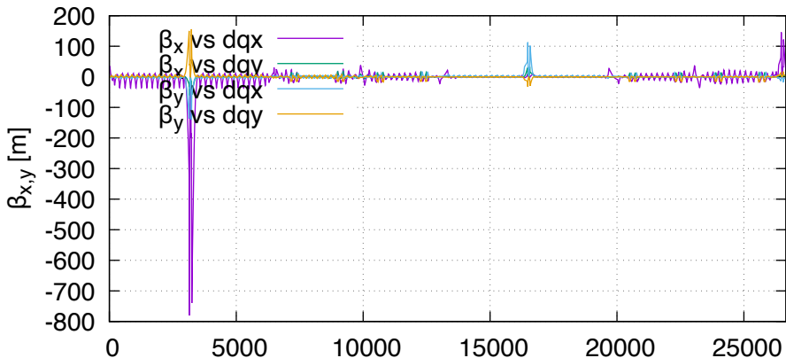
beta (lhcb2, order 1)
