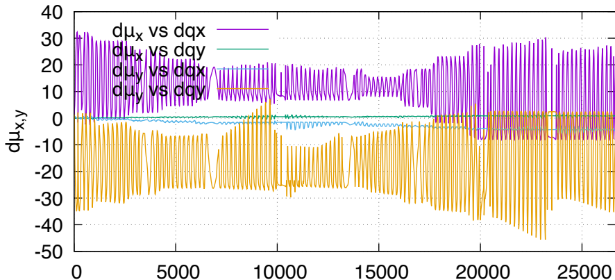
dmu (lhcb1, order 1)
