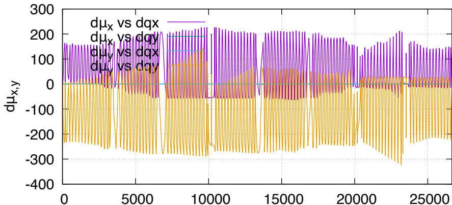
dmu (lhcb1, order 2)
