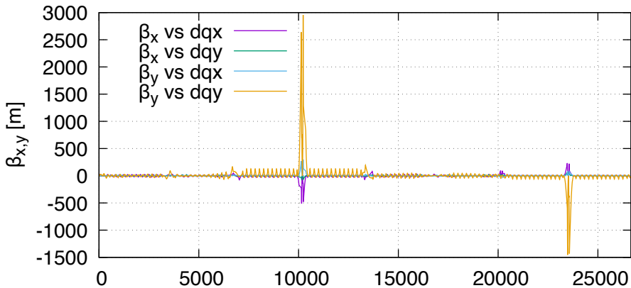
beta (lhcb1, order 1)
