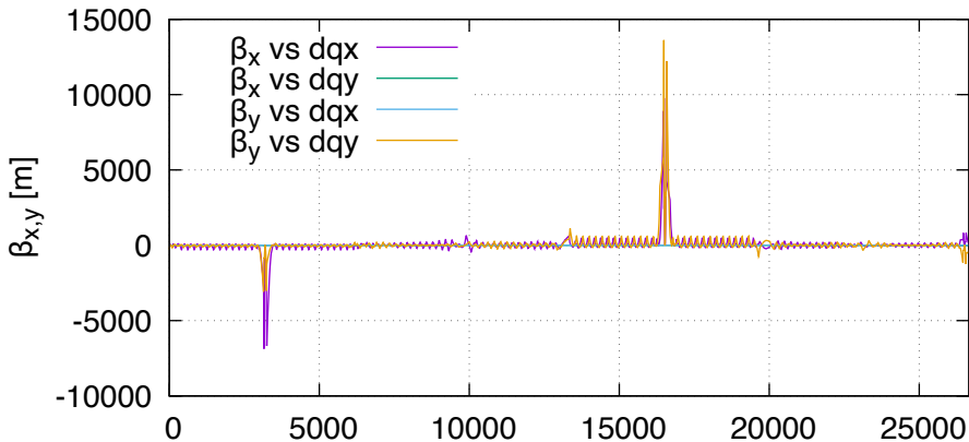
beta (lhcb2, order 2)
