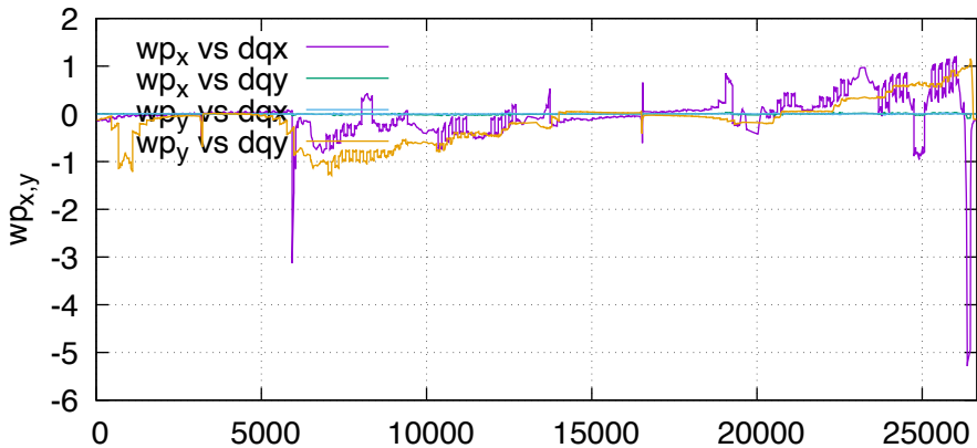
wp (lhcb2, order 1)
