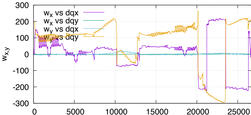
w (lhcb1, order 1)
