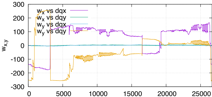
w (lhcb2, order 1)
