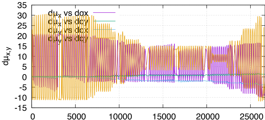
dmu (lhcb2, order 1)
