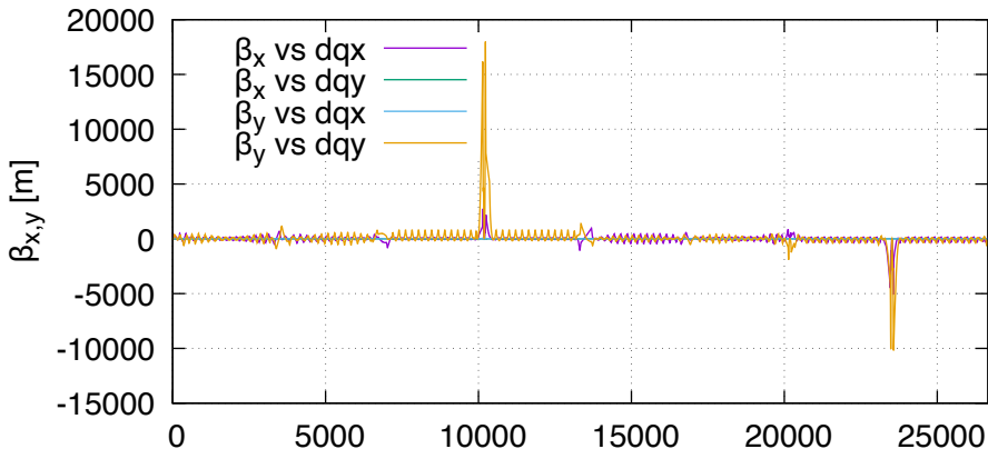
beta (lhcb1, order 2)
