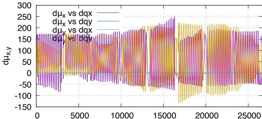
dmu (lhcb2, order 2)
