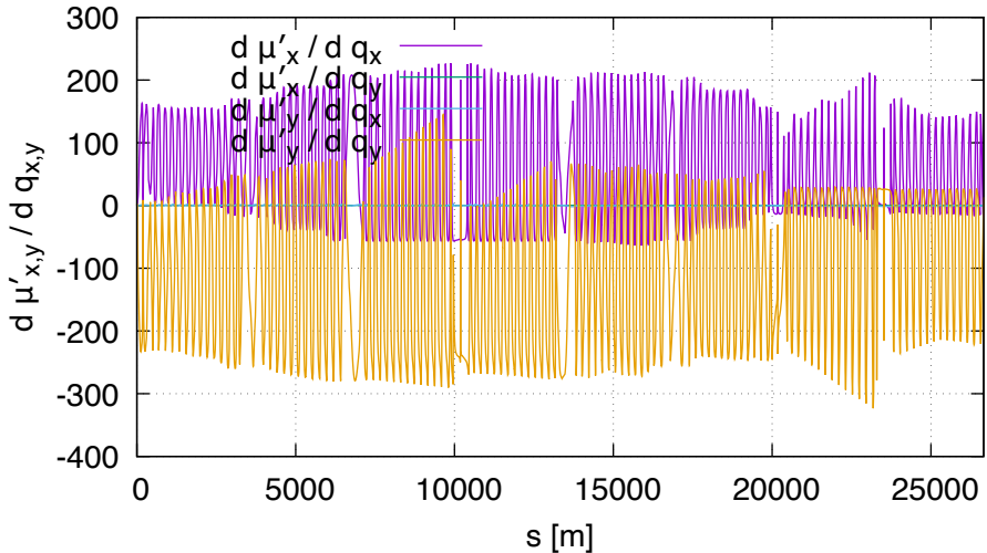
Sensitivity of d\mu (lhcb1, order 2)
