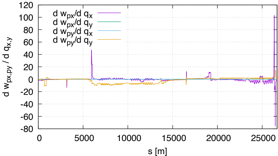
Sensitivity of wp (lhcb2, order 2)
