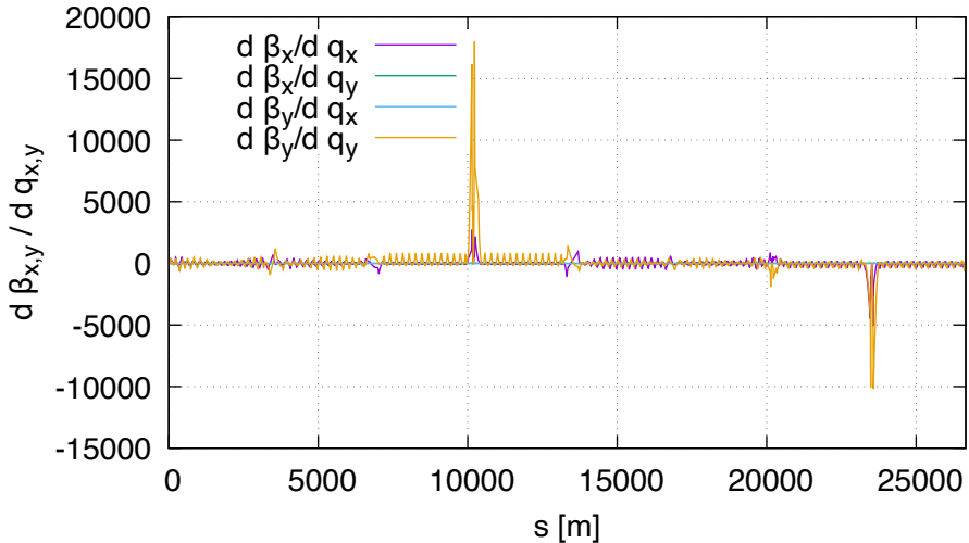
Sensitivity of beta (lhcb1, order 2)
