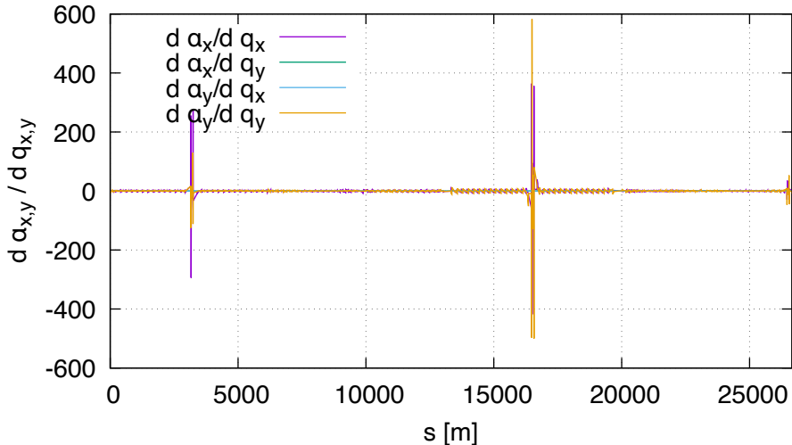
Sensitivity of alpha (lhcb2, order 2)
