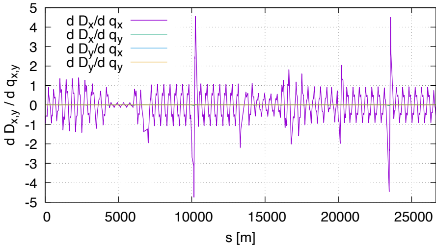
Sensitivity of disp (lhcb1, order 2)
