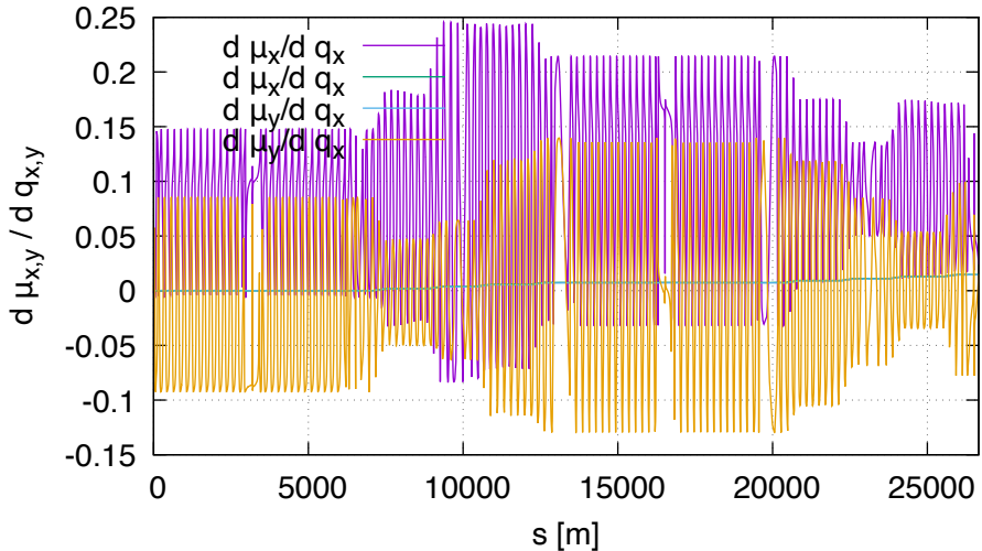
Sensitivity of mu (lhcb2, order 2)
