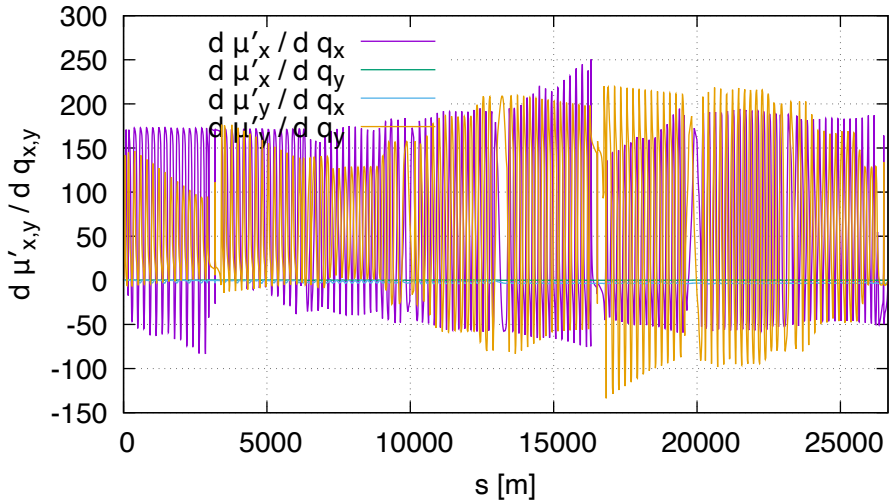
Sensitivity of d\mu (lhcb2, order 2)
