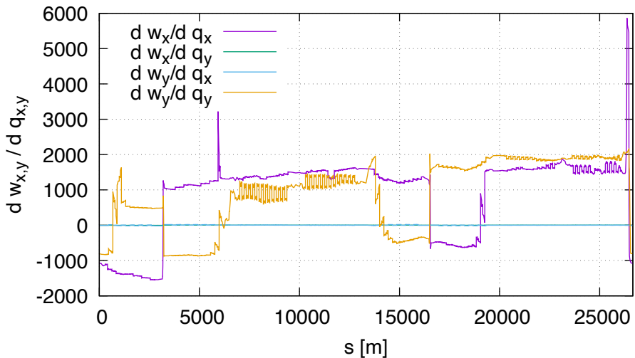
Sensitivity of w (lhcb2, order 2)
