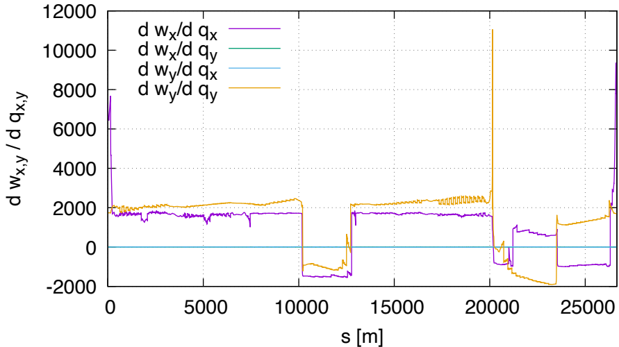
Sensitivity of w (lhcb1, order 2)
