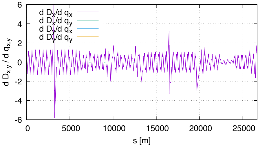
Sensitivity of disp (lhcb2, order 2)
