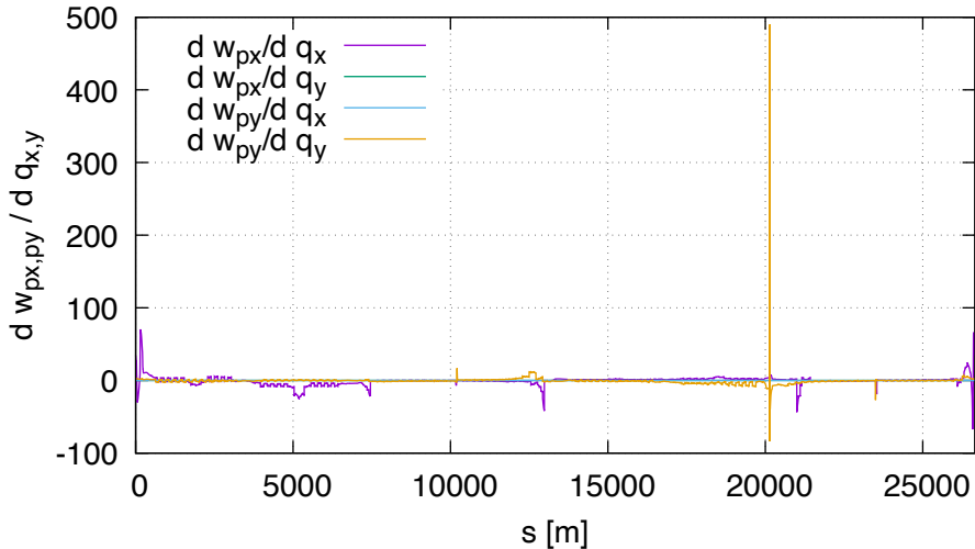
Sensitivity of wp (lhcb1, order 2)
