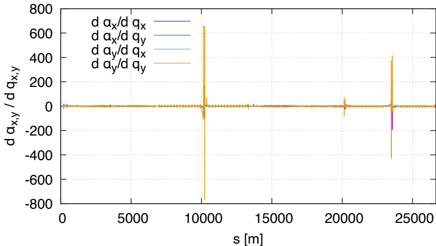
Sensitivity of alpha (lhcb1, order 2)
