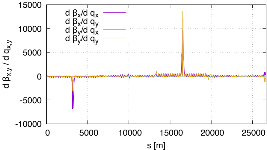
Sensitivity of beta (lhcb2, order 2)
