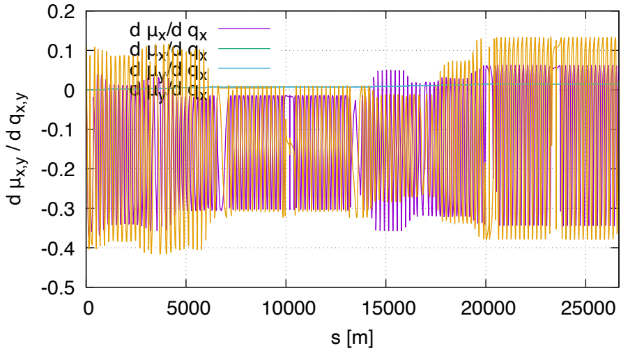
Sensitivity of mu (lhcb1, order 2)
