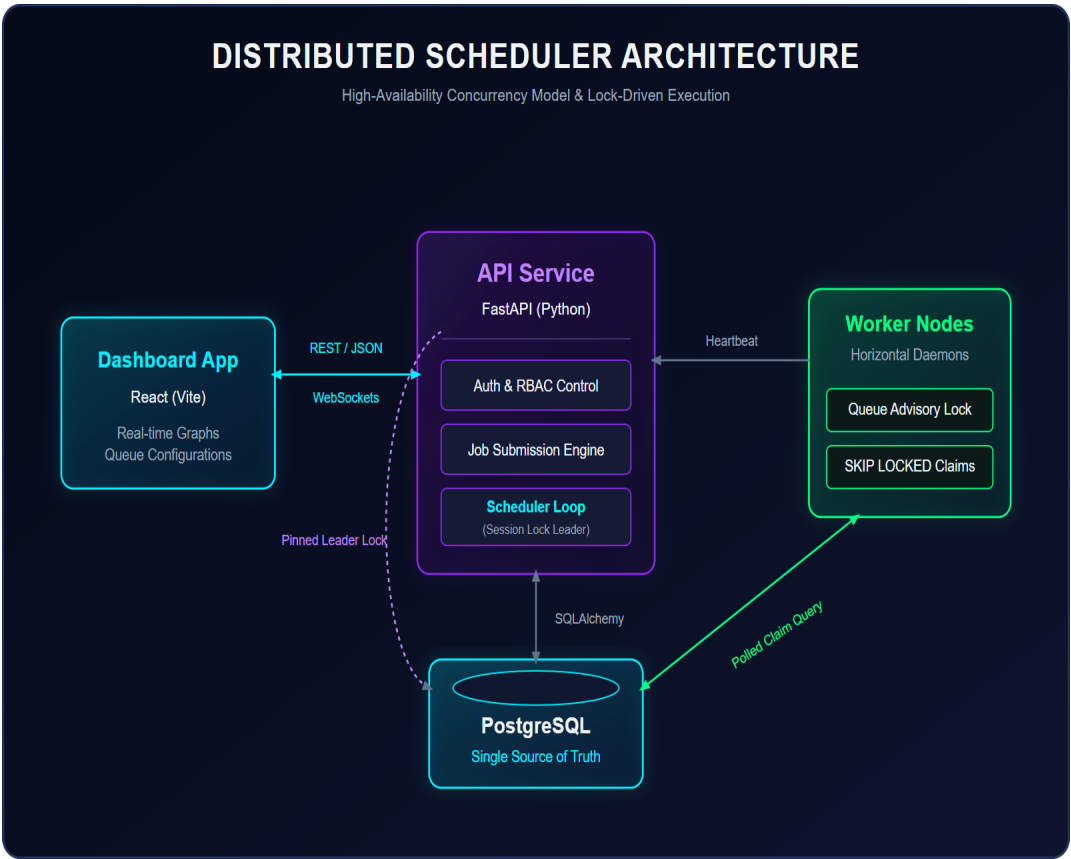
Figure 1: Full System Component Architecture & Locking Channels
