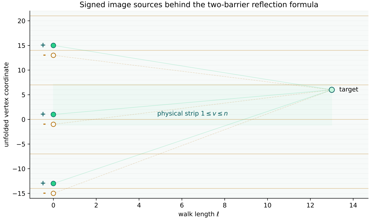
Figure 2: Schematic signed image sources for a strip with two absorbing barriers. Positive and negative unrestricted kernels cancel at the boundaries, leaving exactly the walks that remain inside the physical path.
