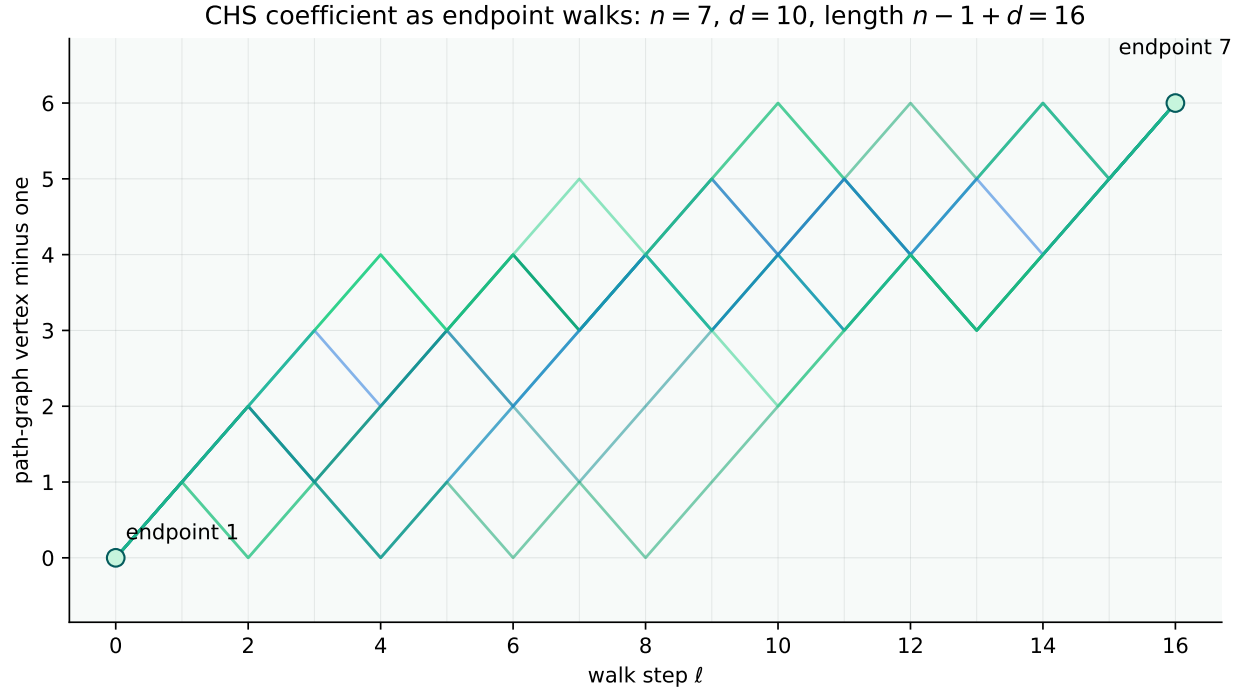
Figure 1: Sample length-16 endpoint walks in P_7 , shown after shifting the vertex coordinate down by one. The exact CHS power \|P_7\|_{X,10}^{10} counts all such walks, not only the displayed sample.
