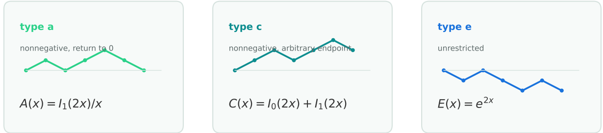
Figure 1: The coordinate constraints separate under exponential generating functions. The factors count type-a, type-c, and type-e coordinate words; their labelled interleaving reconstructs the three-dimensional walk.
