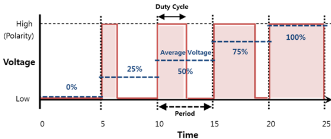
Figure 17: PWM Waveforms[12]
