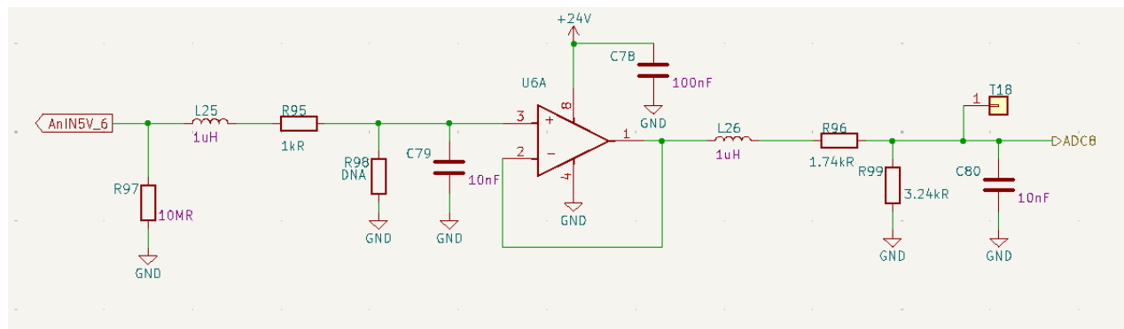
Figure 22: Filtering System for 5V amplitude signal
