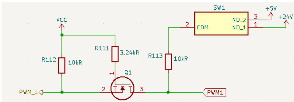
Figure 18: PWM Level-Shifter
