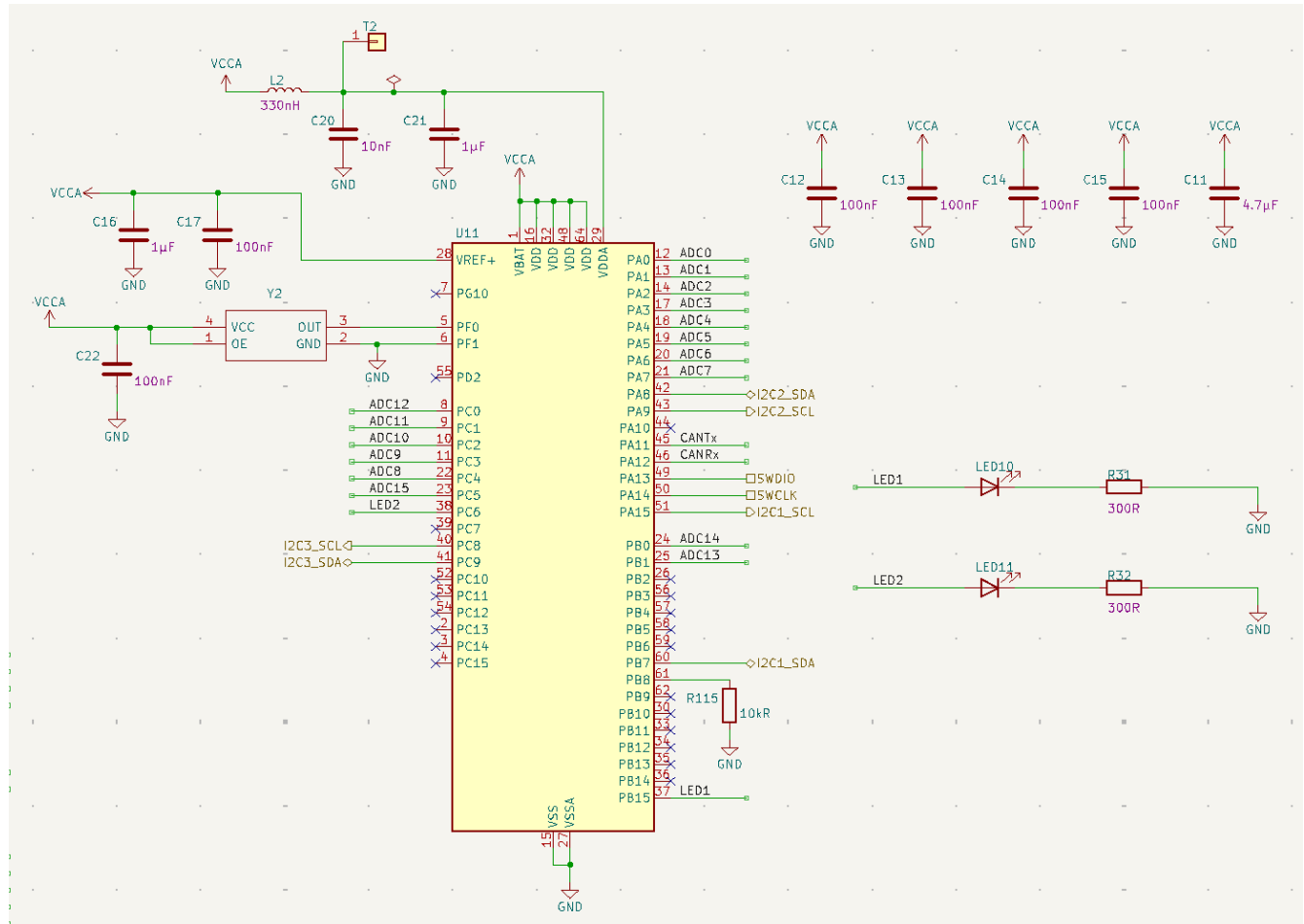
Figure 20: Analog Node schematic v2.2
