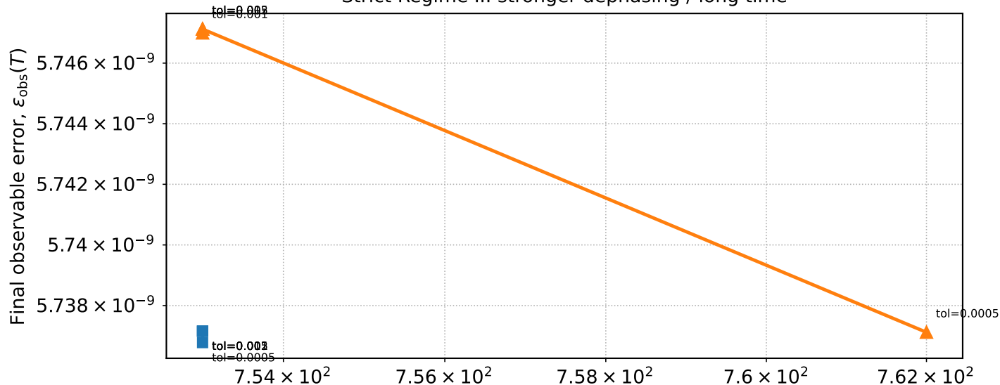
Strict Regime II: stronger dephasing / long time
