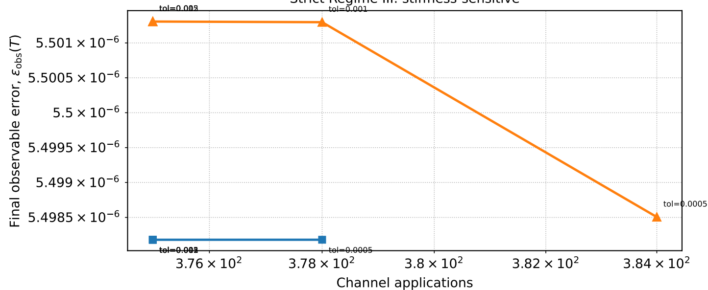
Strict Regime III: stiffness-sensitive
