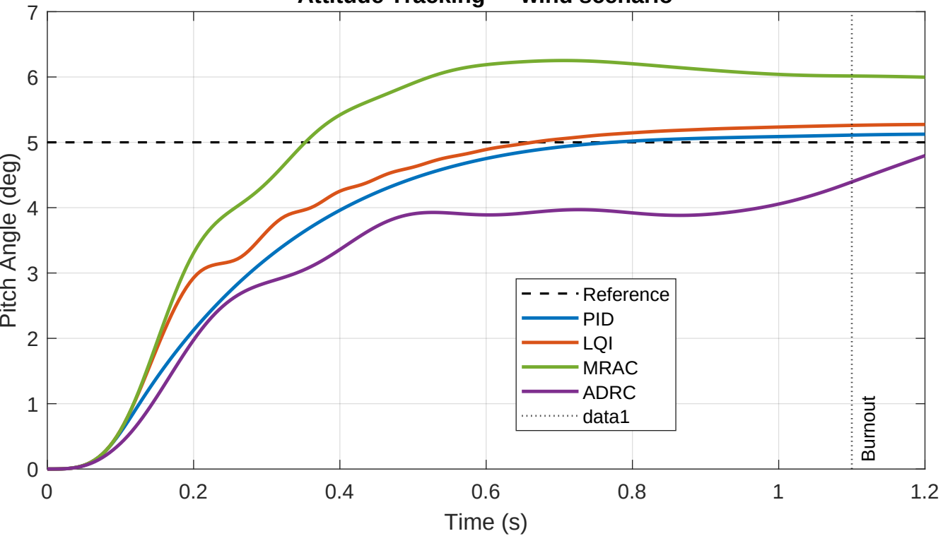
Attitude Tracking — wind scenario
