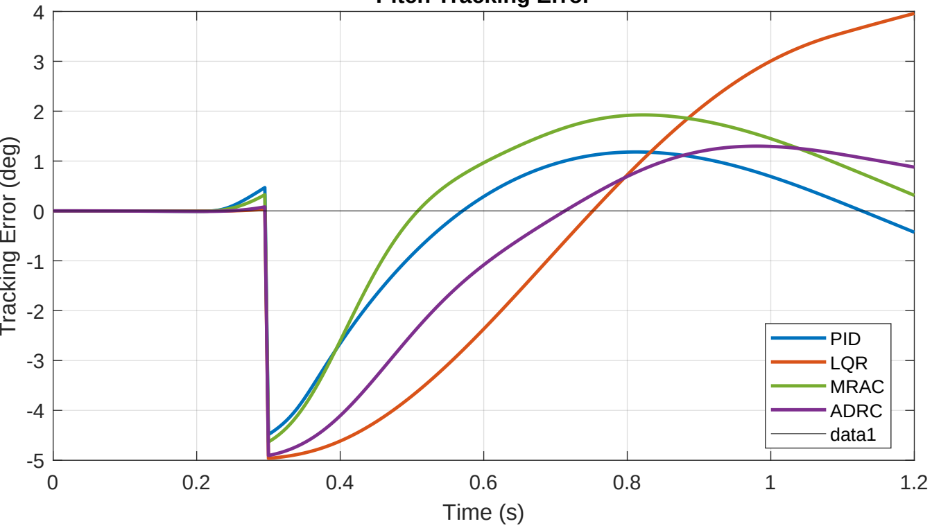
Pitch Tracking Error
