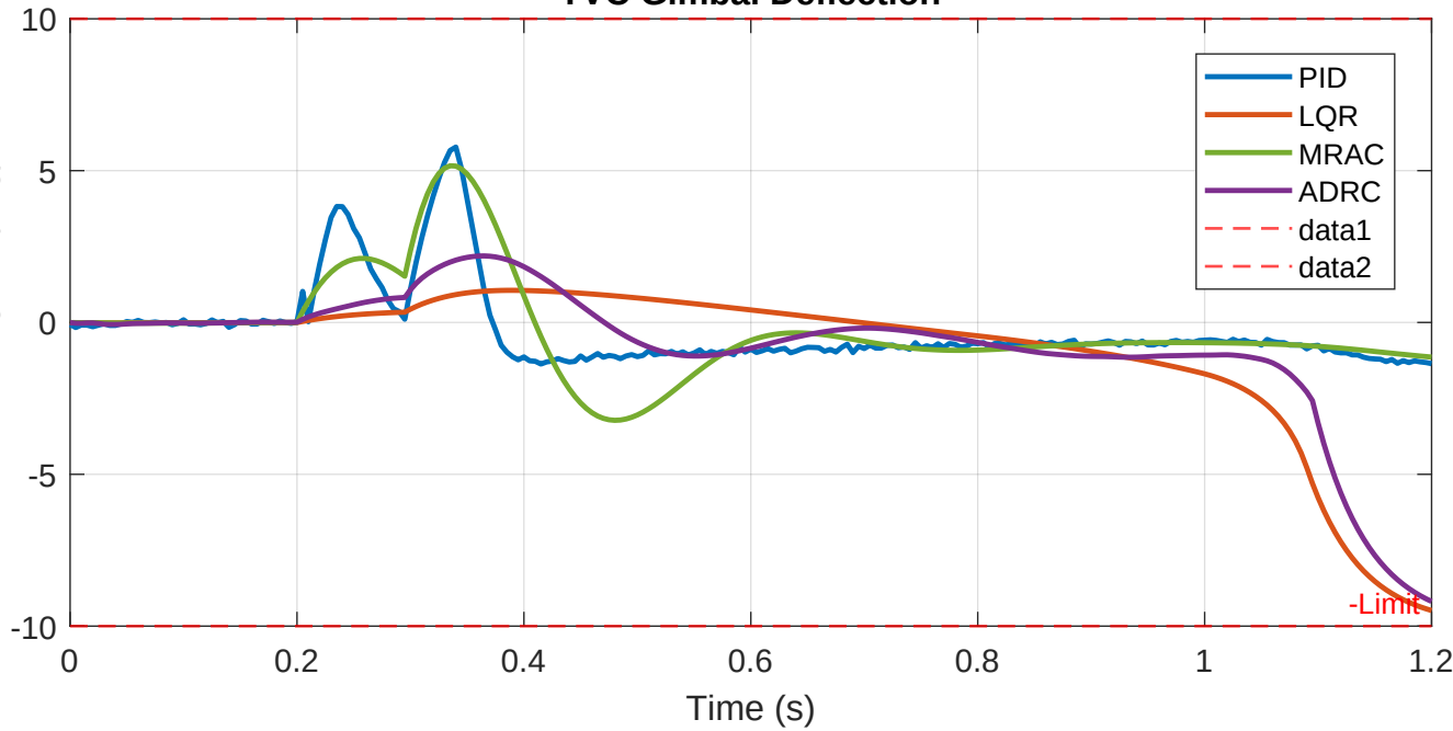
TVC Gimbal Deflection
