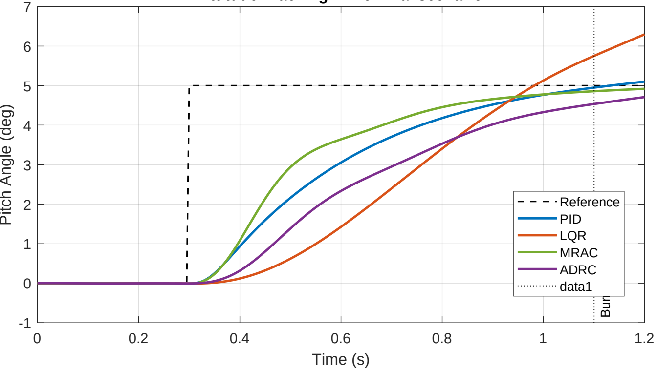
Attitude Tracking — nominal scenario
