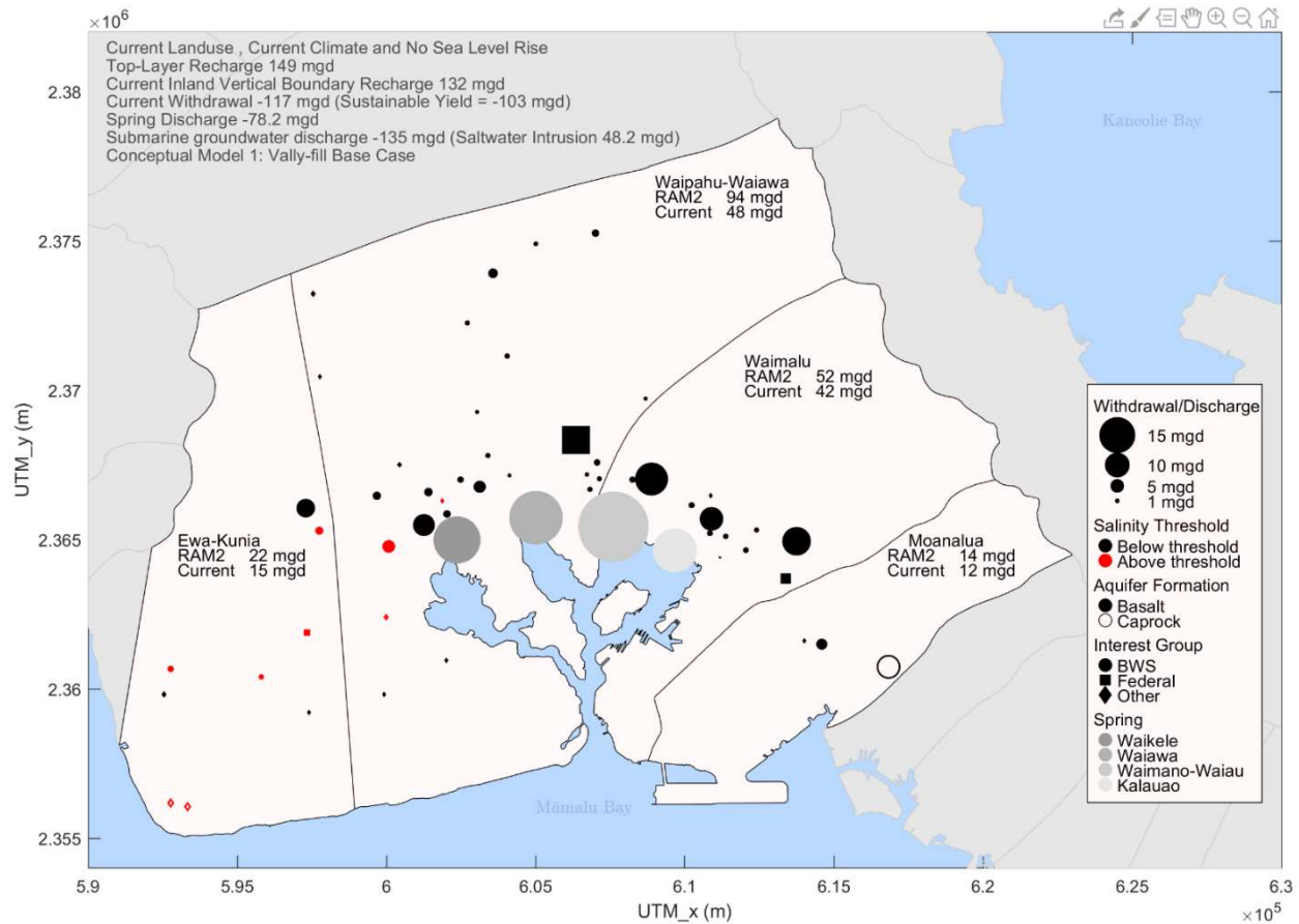
Fig. 6. Future projection of current withdrawal rates under current climate of both recharge and sea-level rise with current land-use management.
