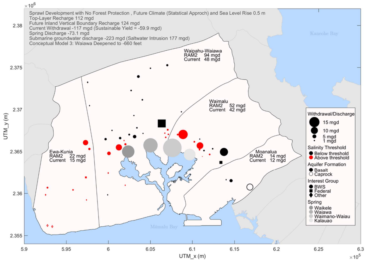
Fig. 7. Future projection of current withdrawal rates under future climate projections of both recharge and sea-level rise with suboptimal land-use management.
