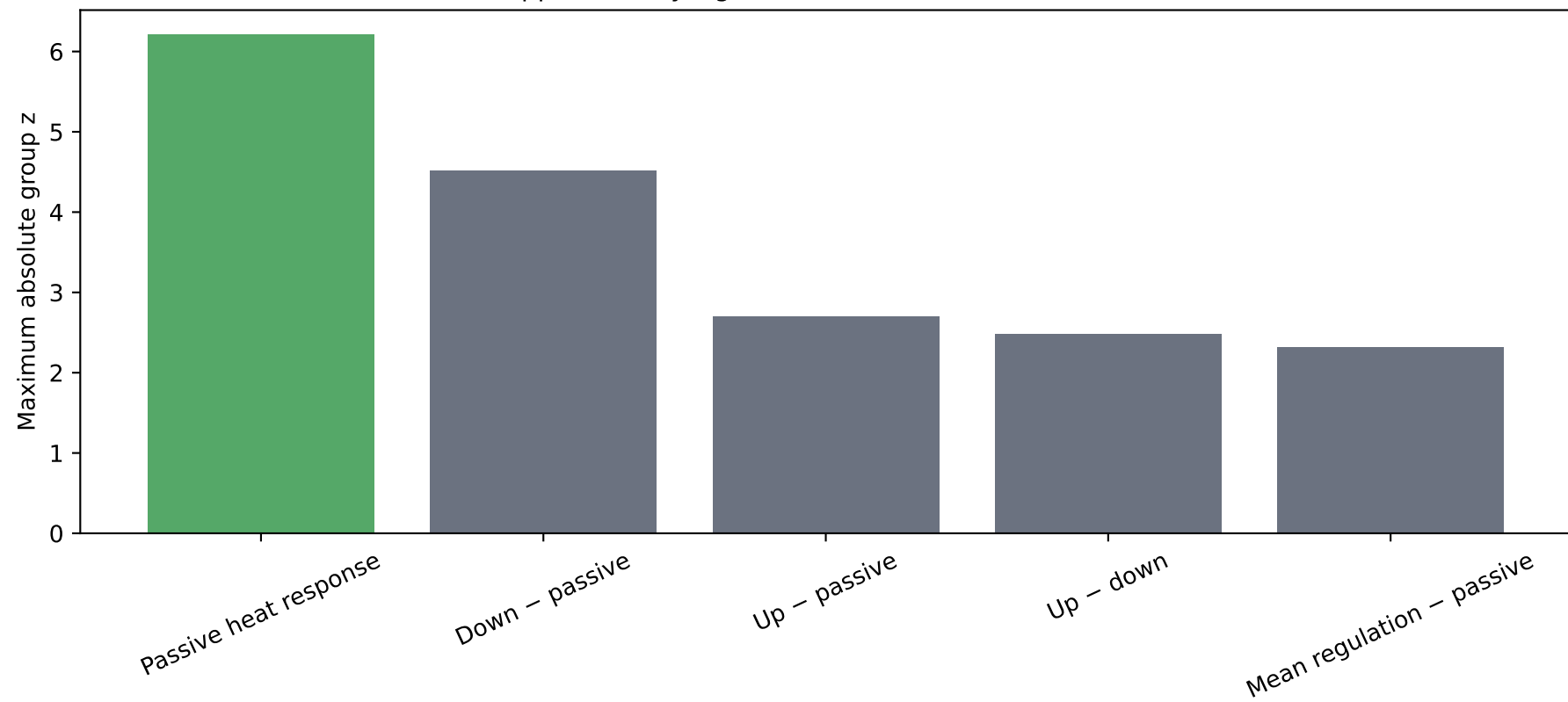
Supplementary Figure 2. Whole-brain GLM contrasts
