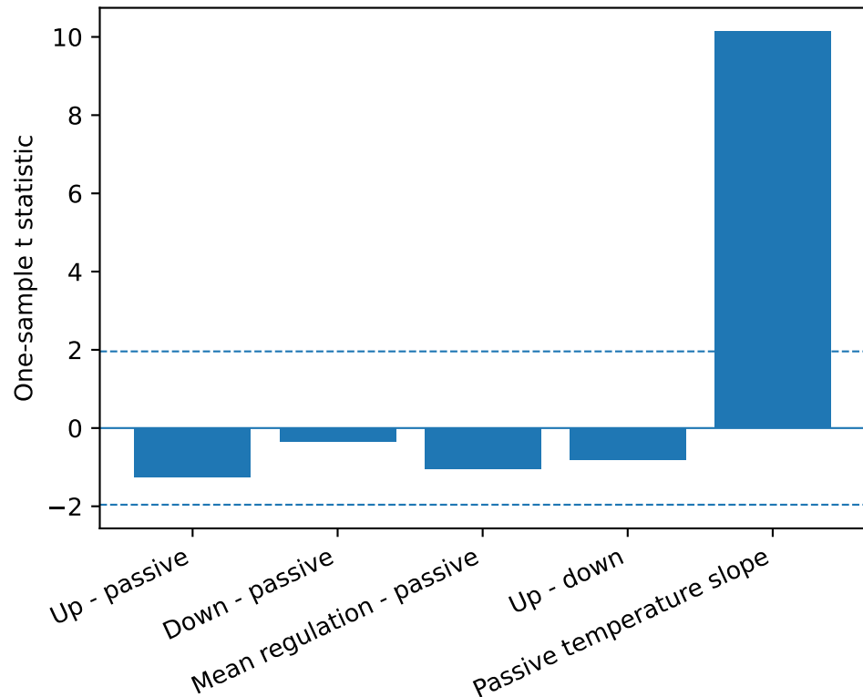
B. Rating-adjusted FWL-LSS NPS
