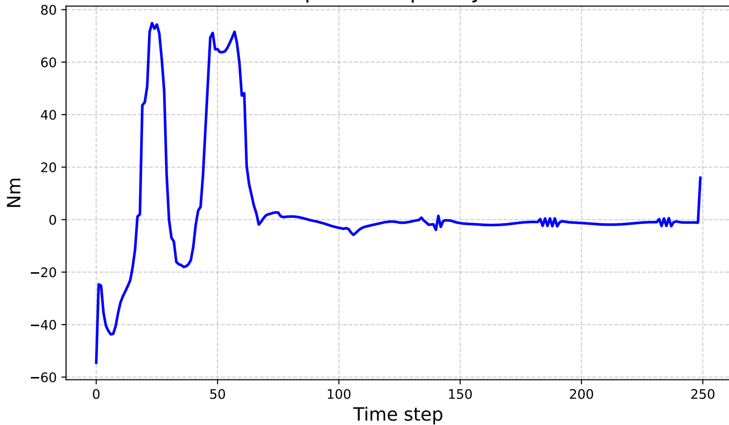
Computed Torques - Joint 5
