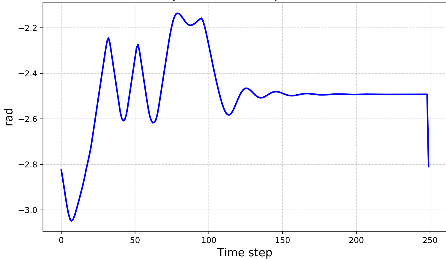
Joint Positions - Joint 4
