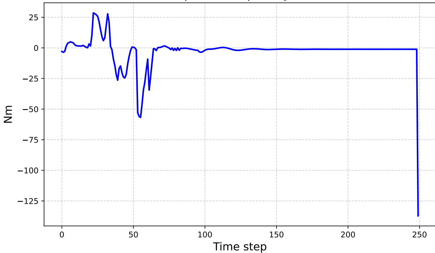
Computed Torques - Joint 6
