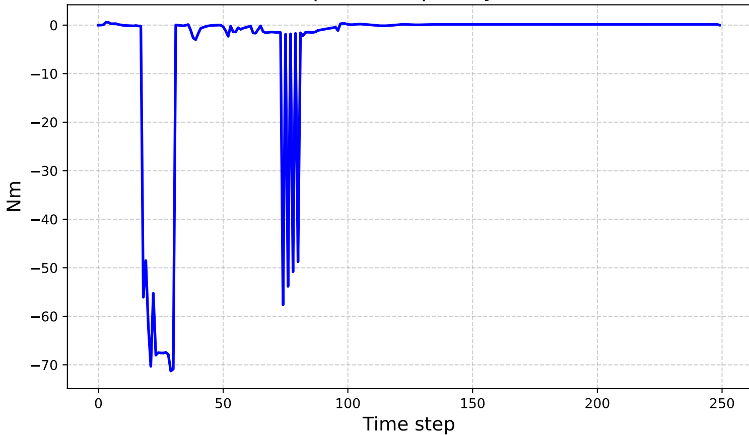
Computed Torques - Joint 9
