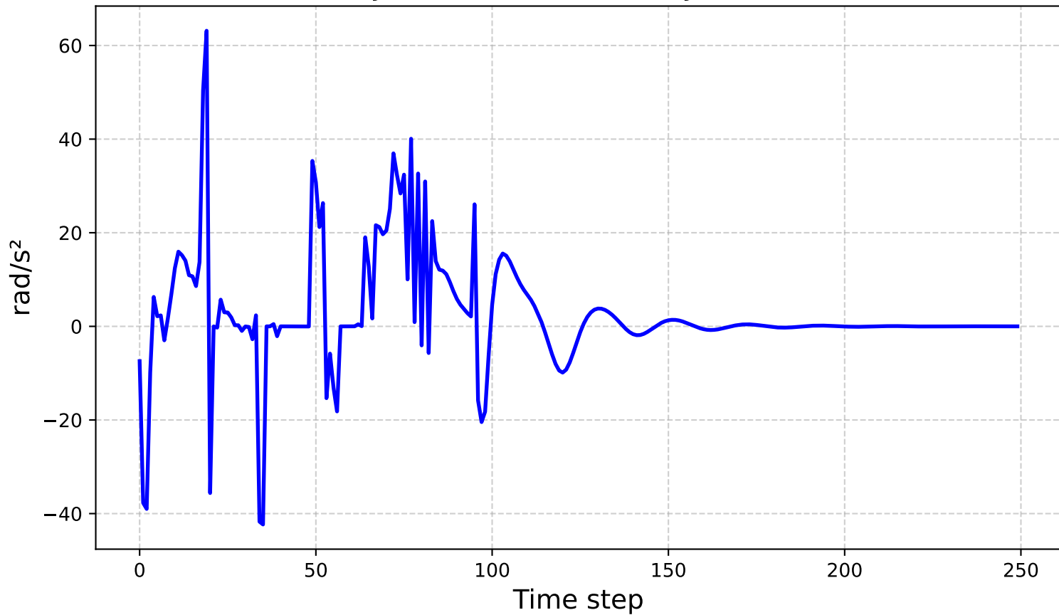
Joint Accelerations - Joint 6
