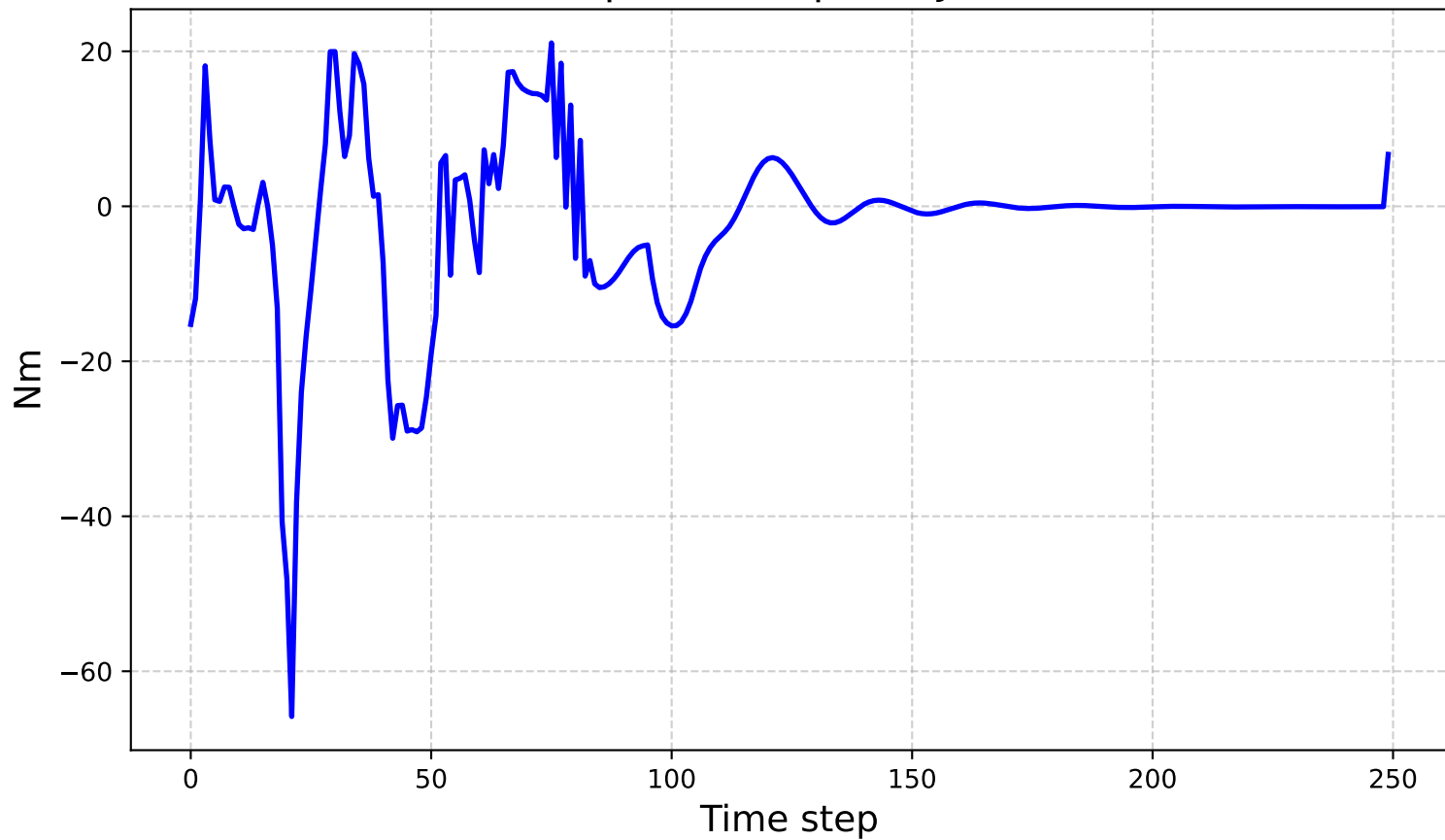
Computed Torques - Joint 1
