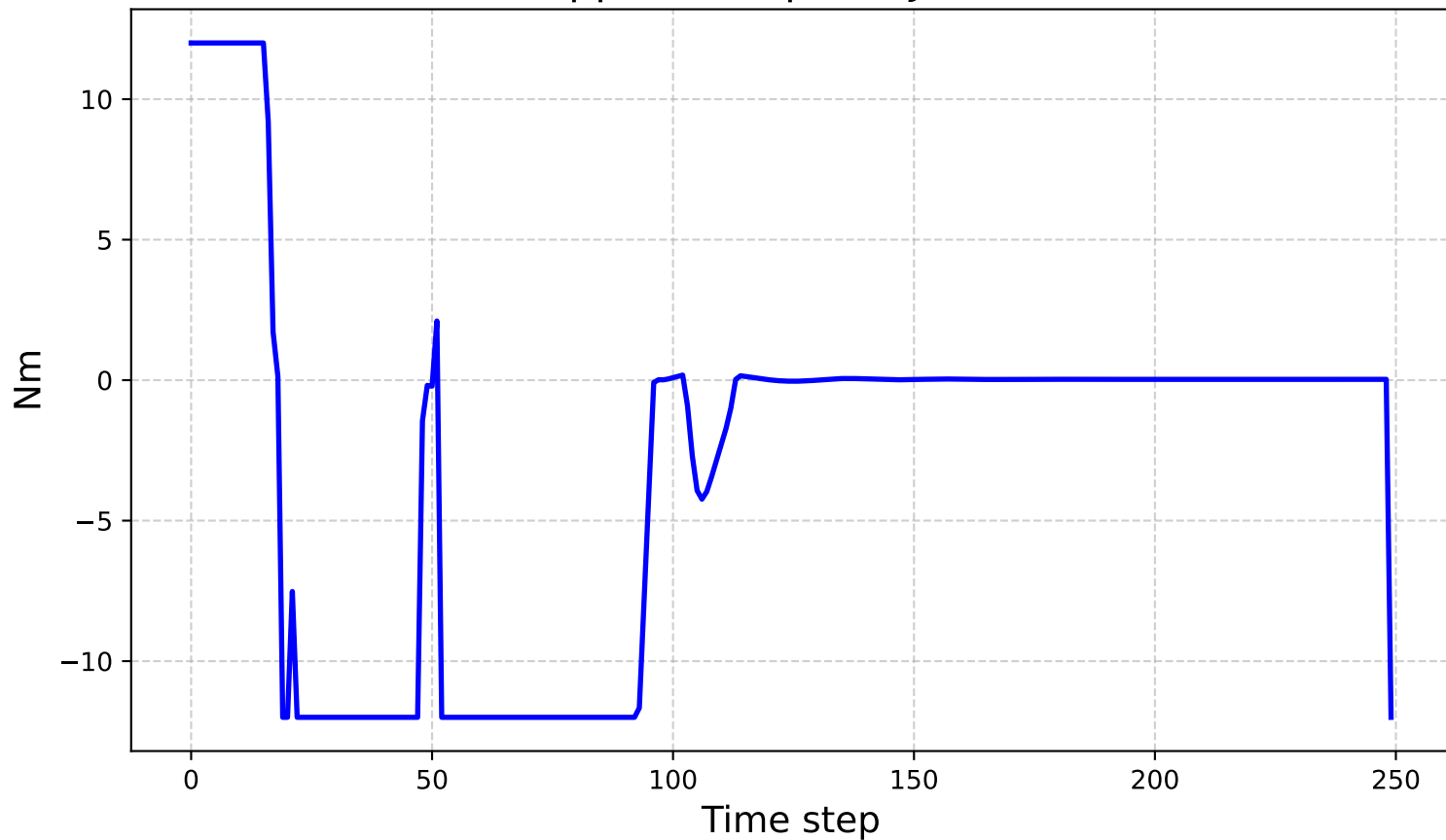
Applied Torques - Joint 7
