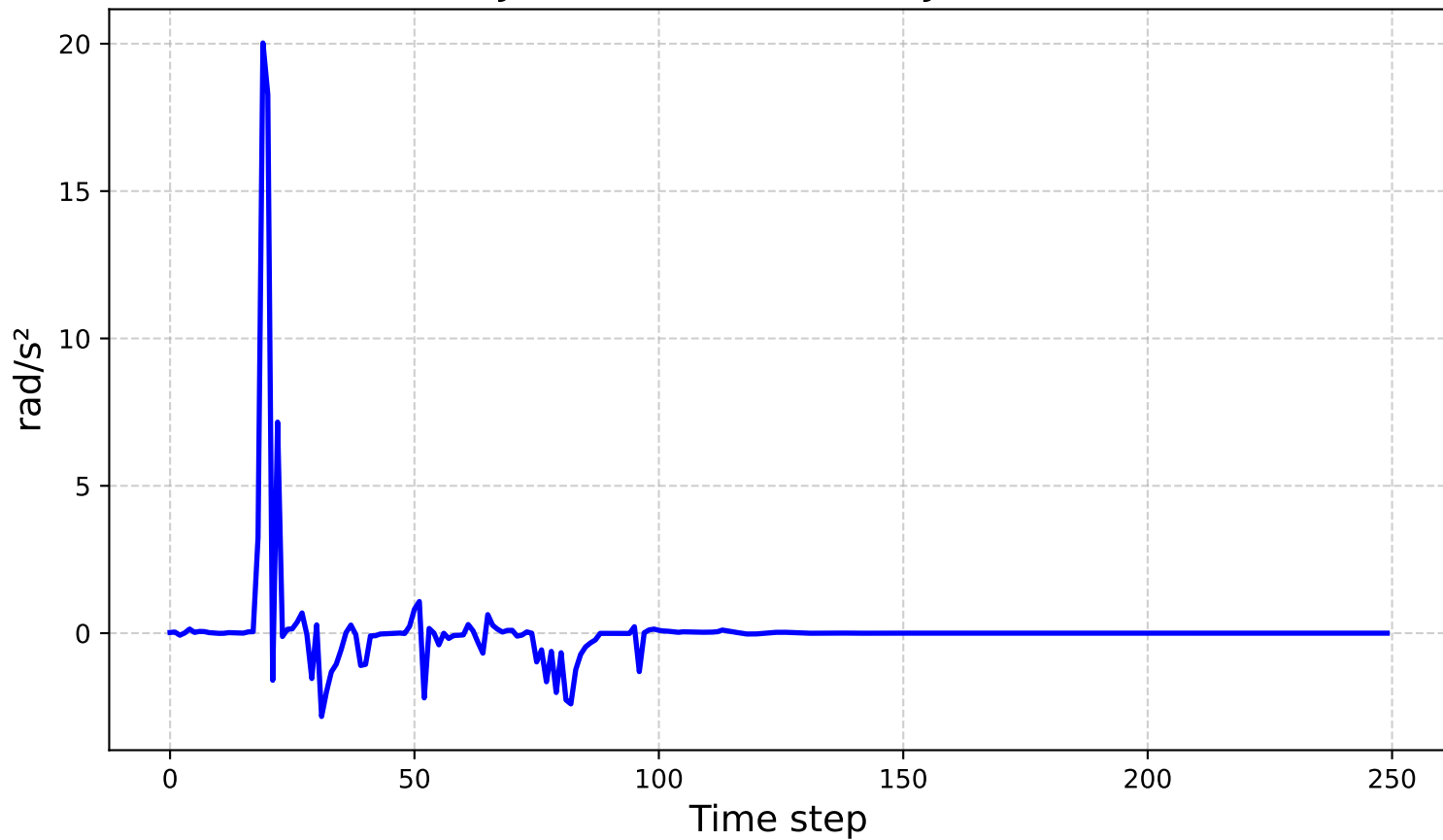
Joint Accelerations - Joint 9
