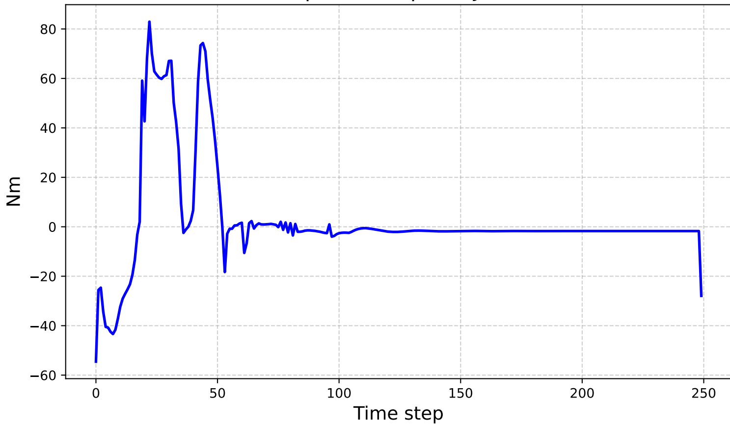
Computed Torques - Joint 5
