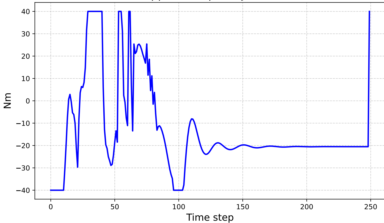
Applied Torques - Joint 3
