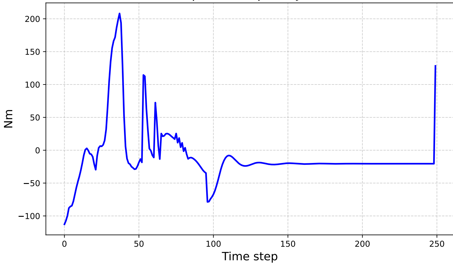
Computed Torques - Joint 3
