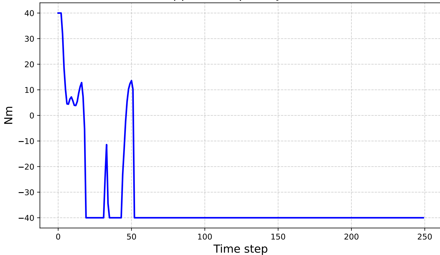
Applied Torques - Joint 2
