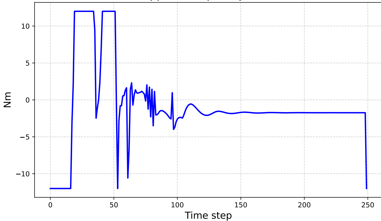
Applied Torques - Joint 5
