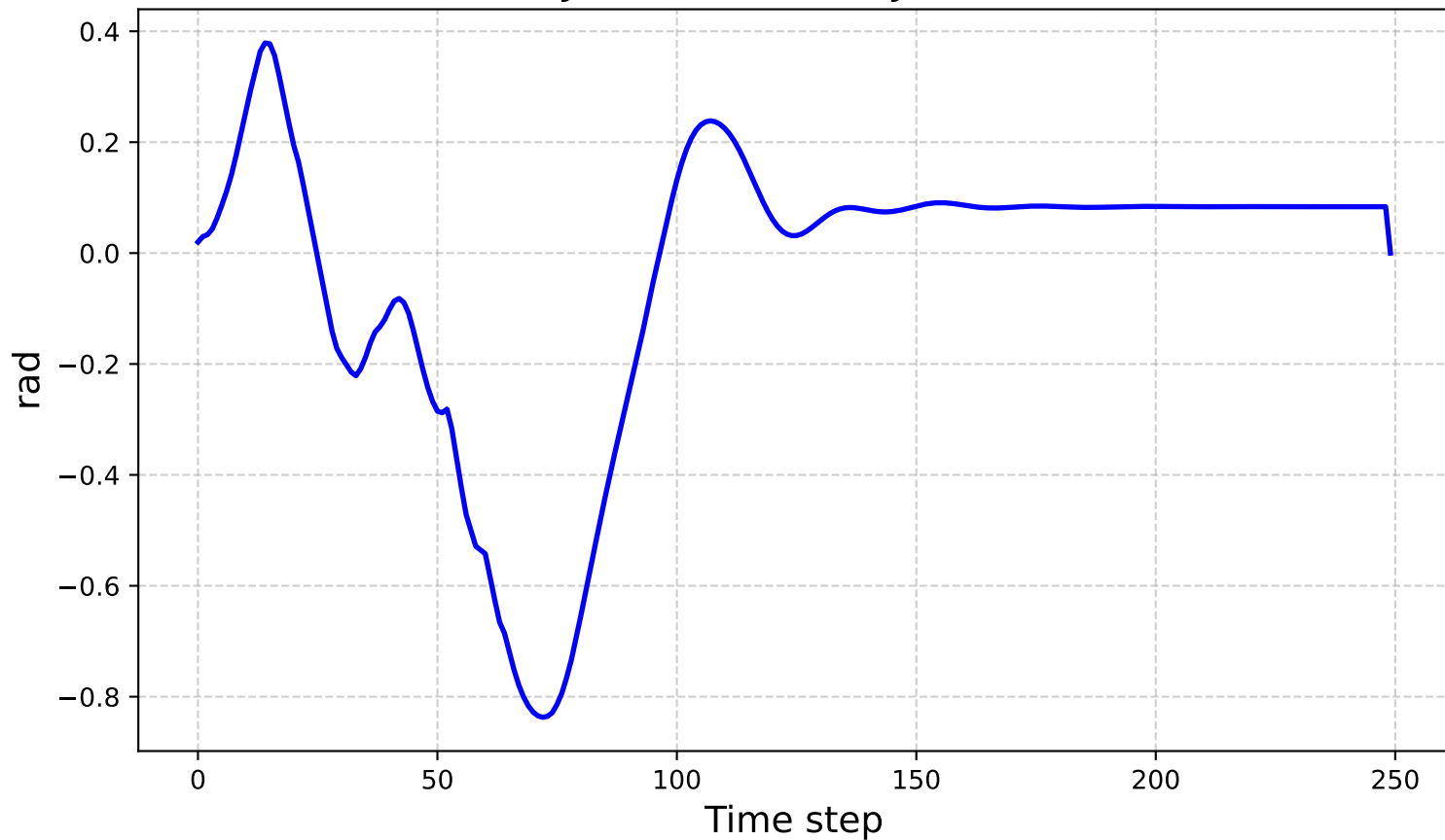
Joint Positions - Joint 1
