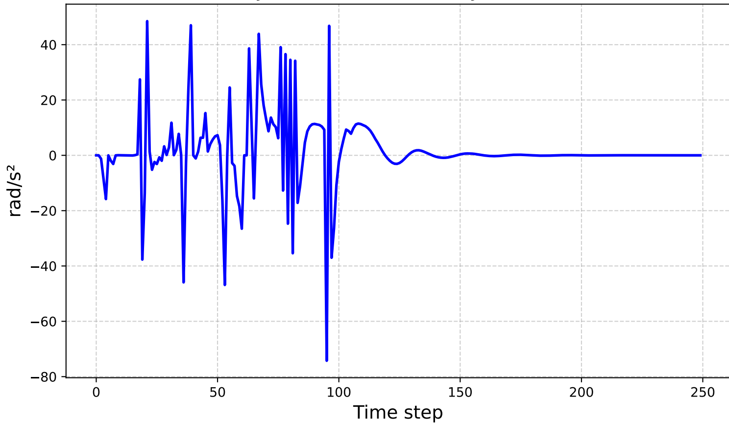
Joint Accelerations - Joint 5
