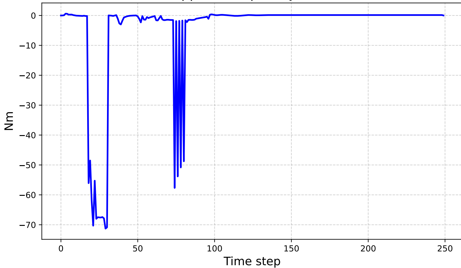
Applied Torques - Joint 9
