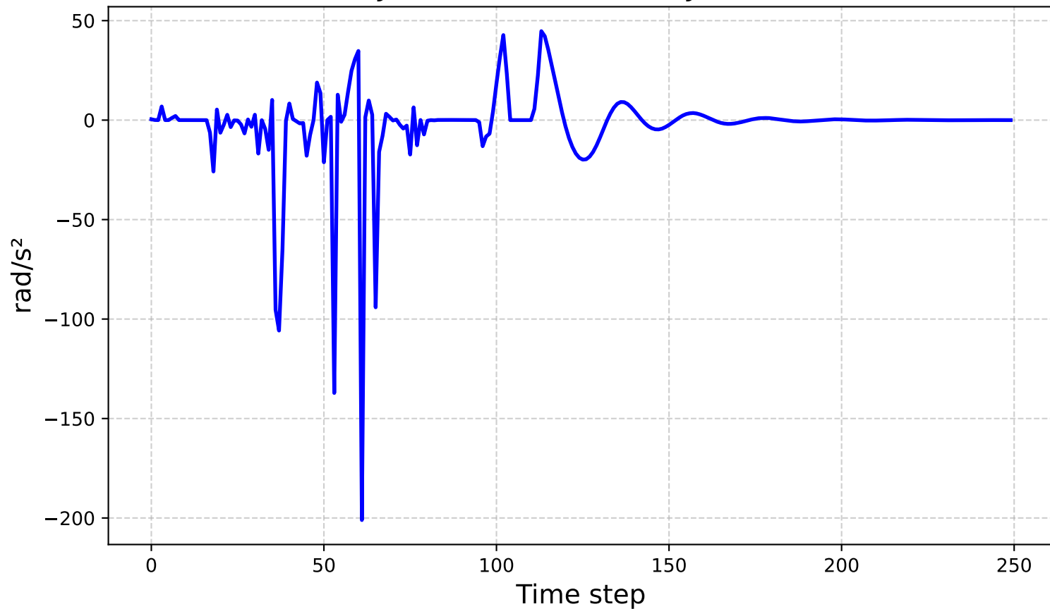
Joint Accelerations - Joint 7
