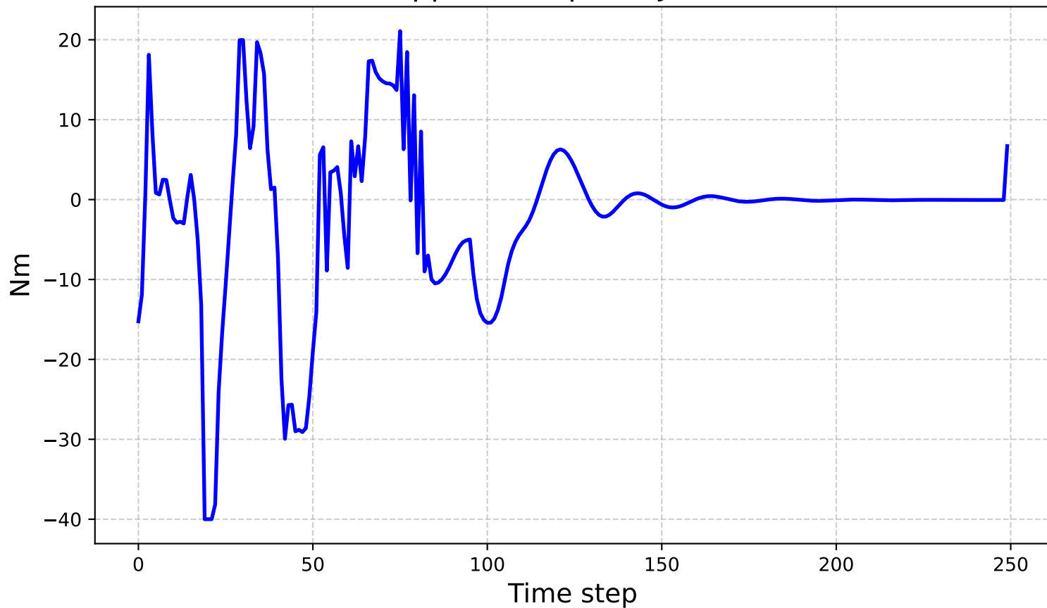
Applied Torques - Joint 1
