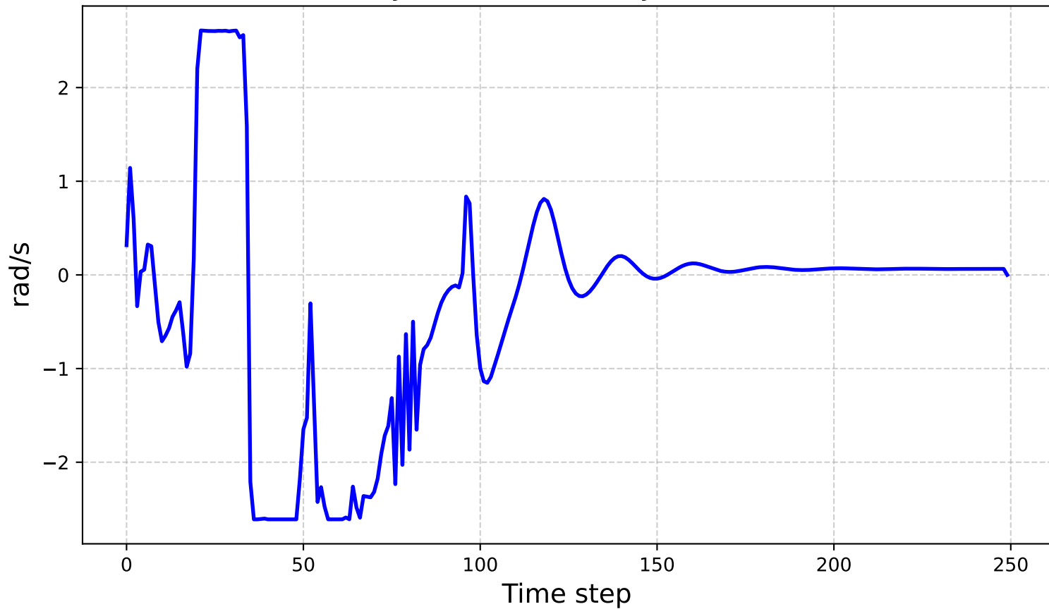
Joint Velocities - Joint 6
