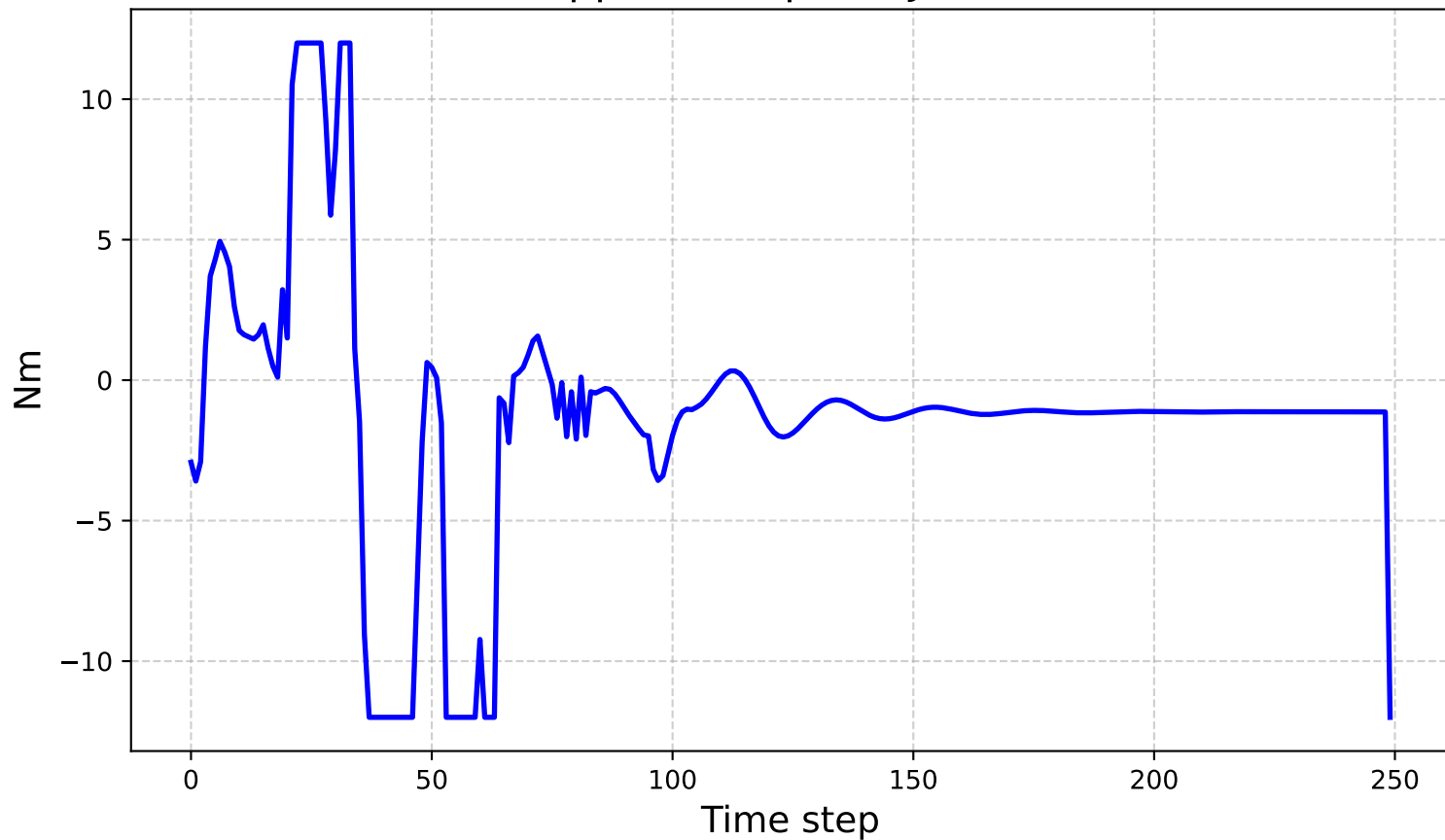
Applied Torques - Joint 6
