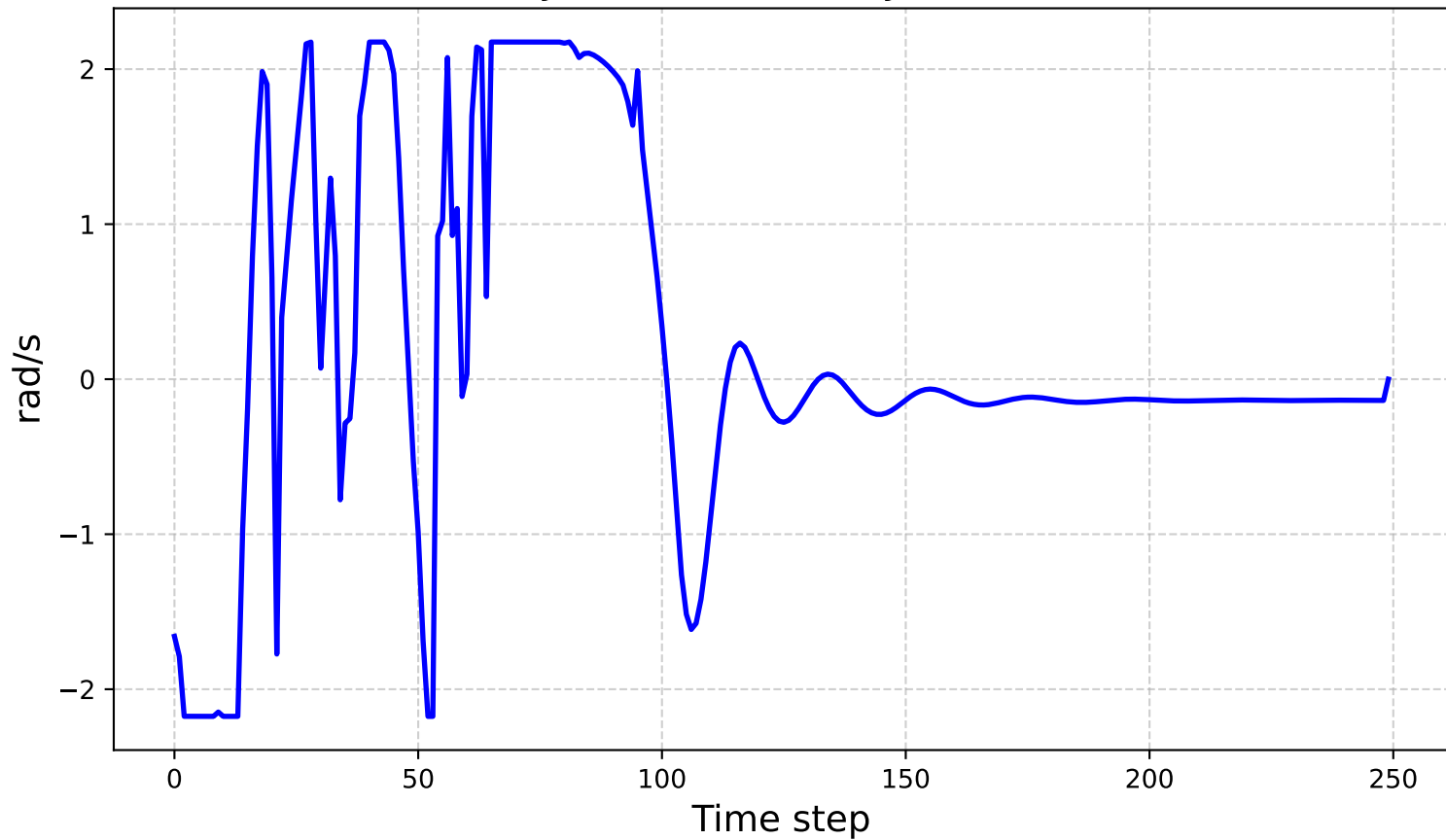
Joint Velocities - Joint 3
