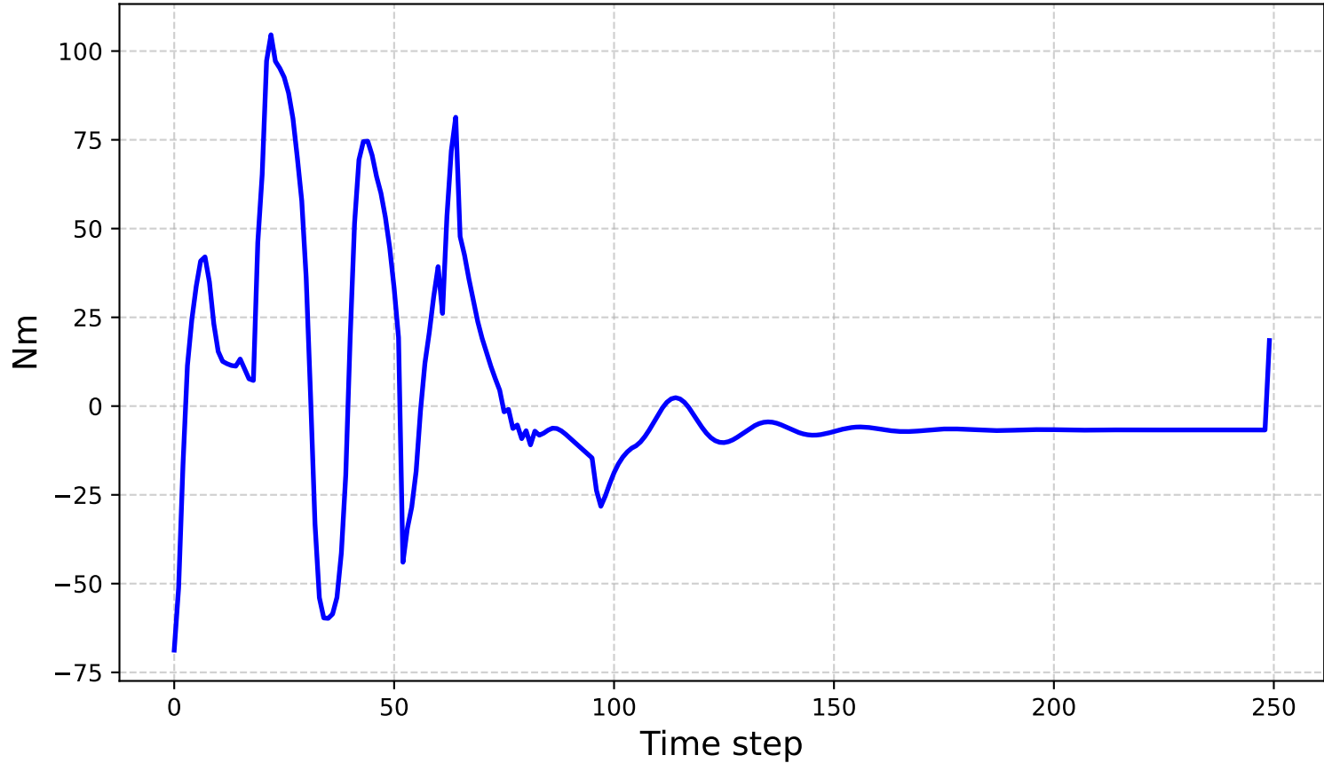
Computed Torques - Joint 4
