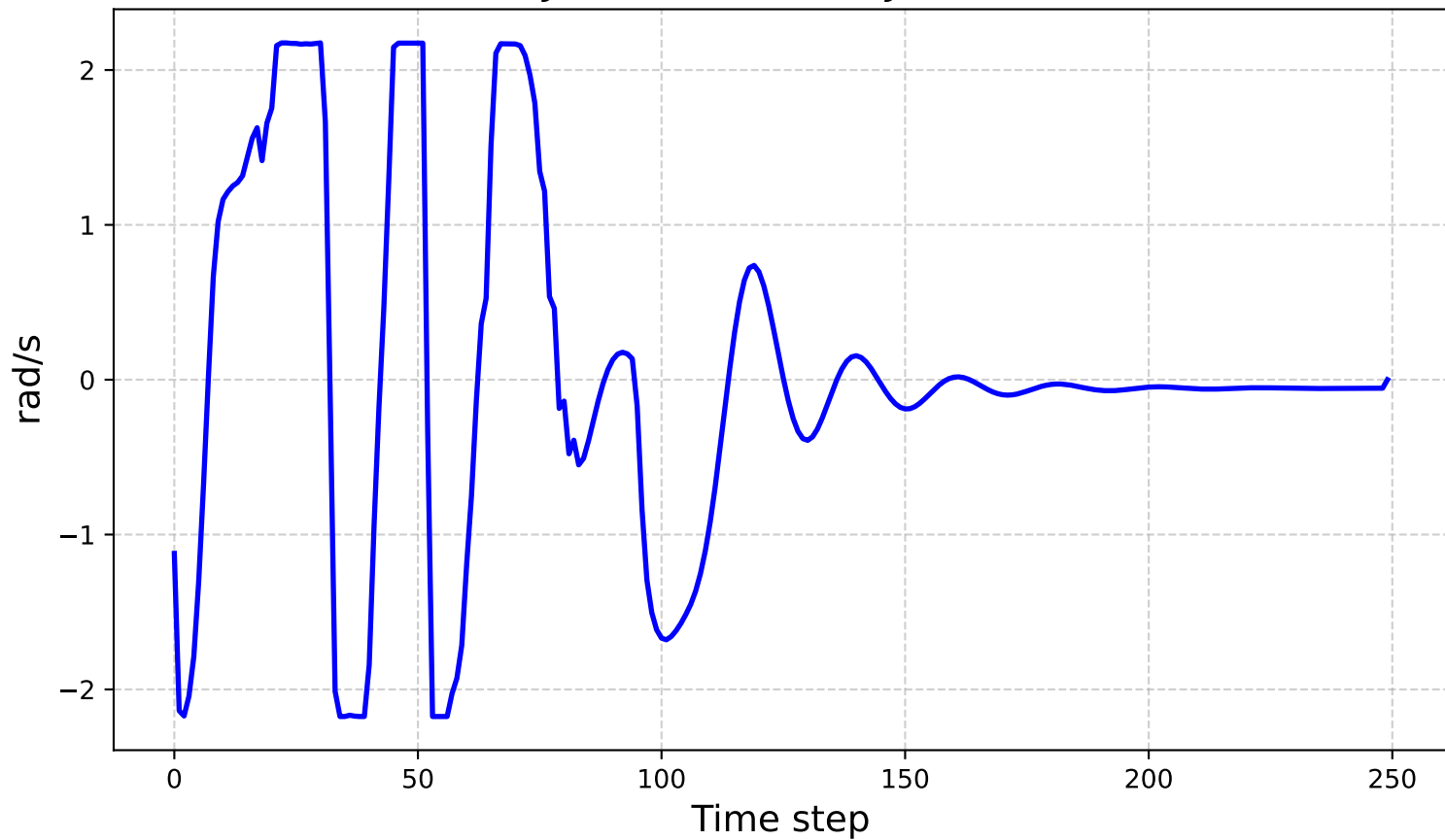
Joint Velocities - Joint 4
