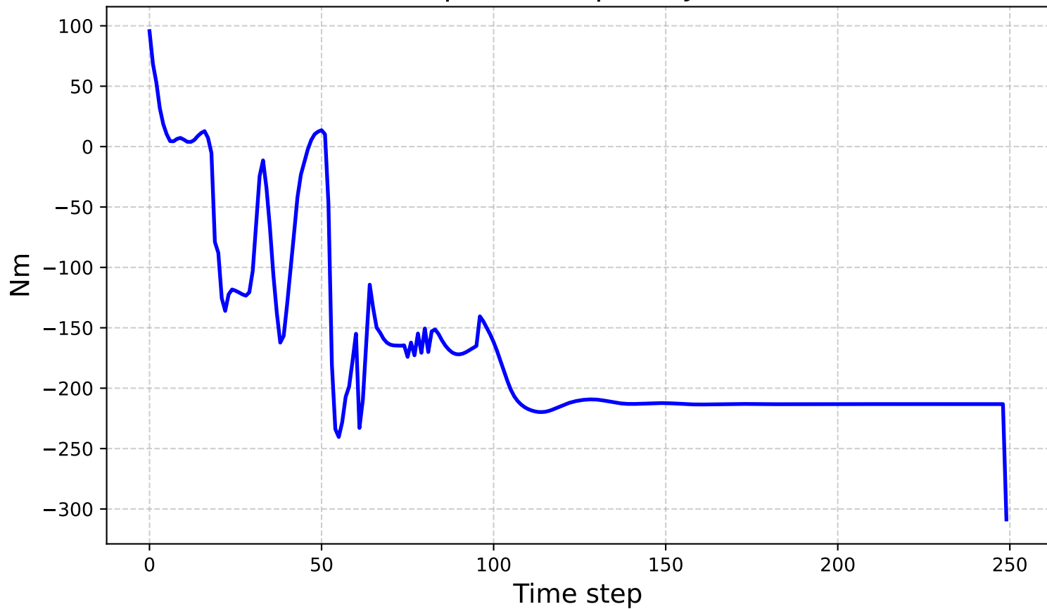
Computed Torques - Joint 2
