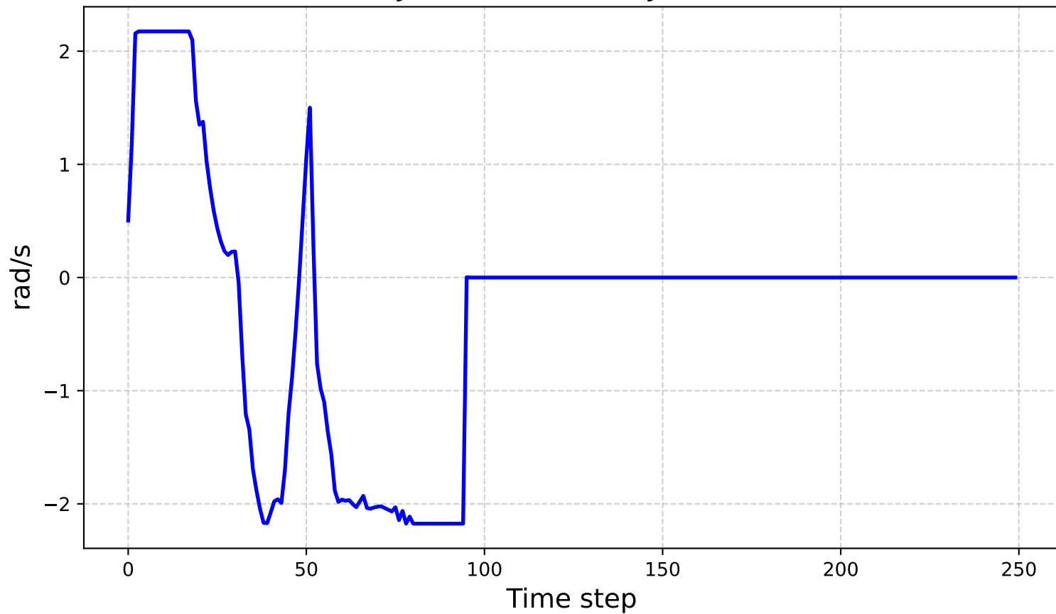
Joint Velocities - Joint 2
