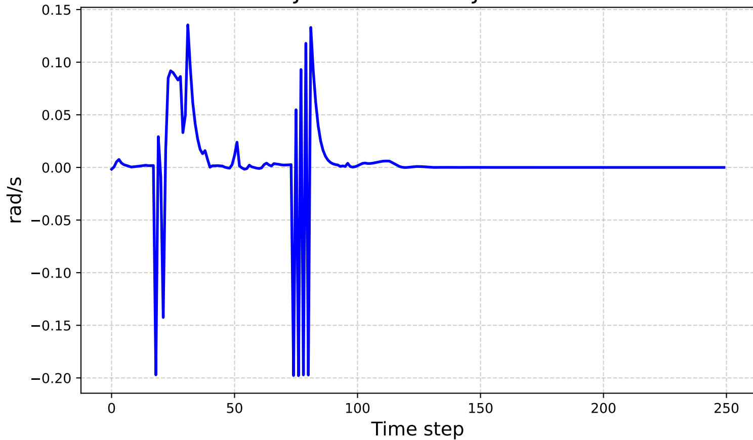
Joint Velocities - Joint 8
