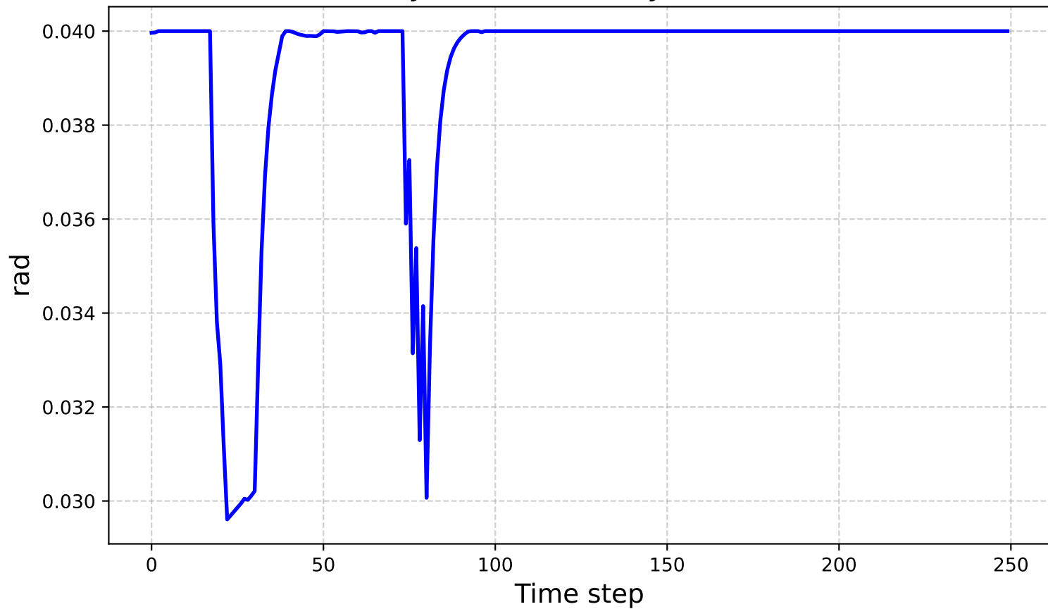
Joint Positions - Joint 8
