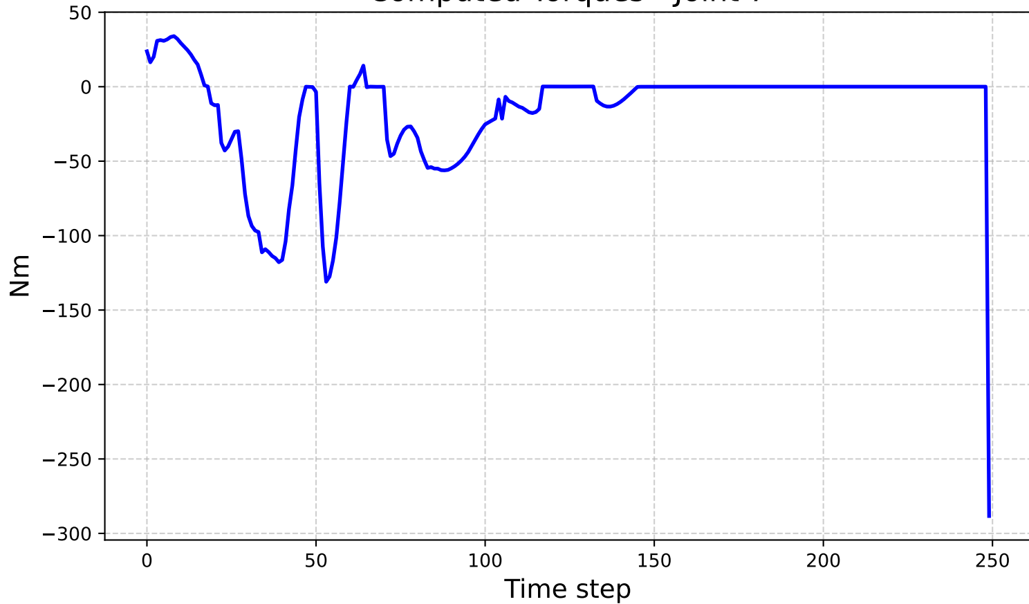
Computed Torques - Joint 7
