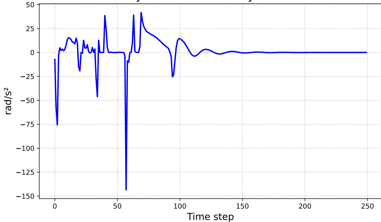
Joint Accelerations - Joint 6
