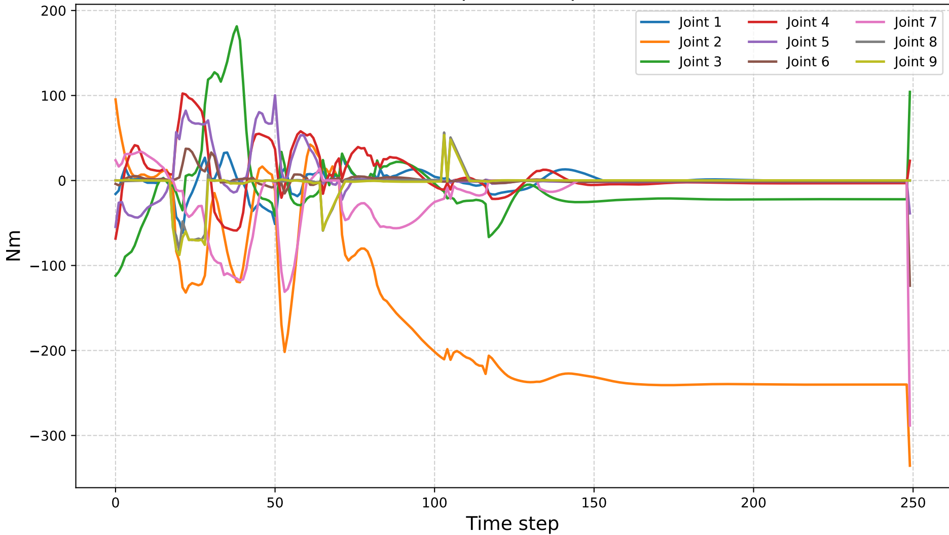
Computed Torques
