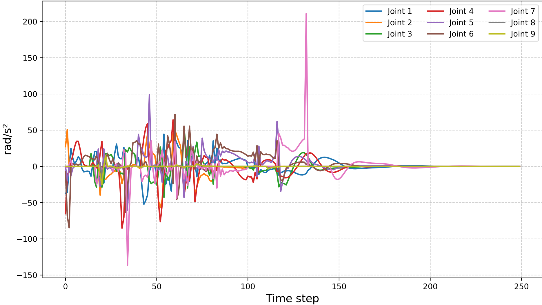
Joint Accelerations
