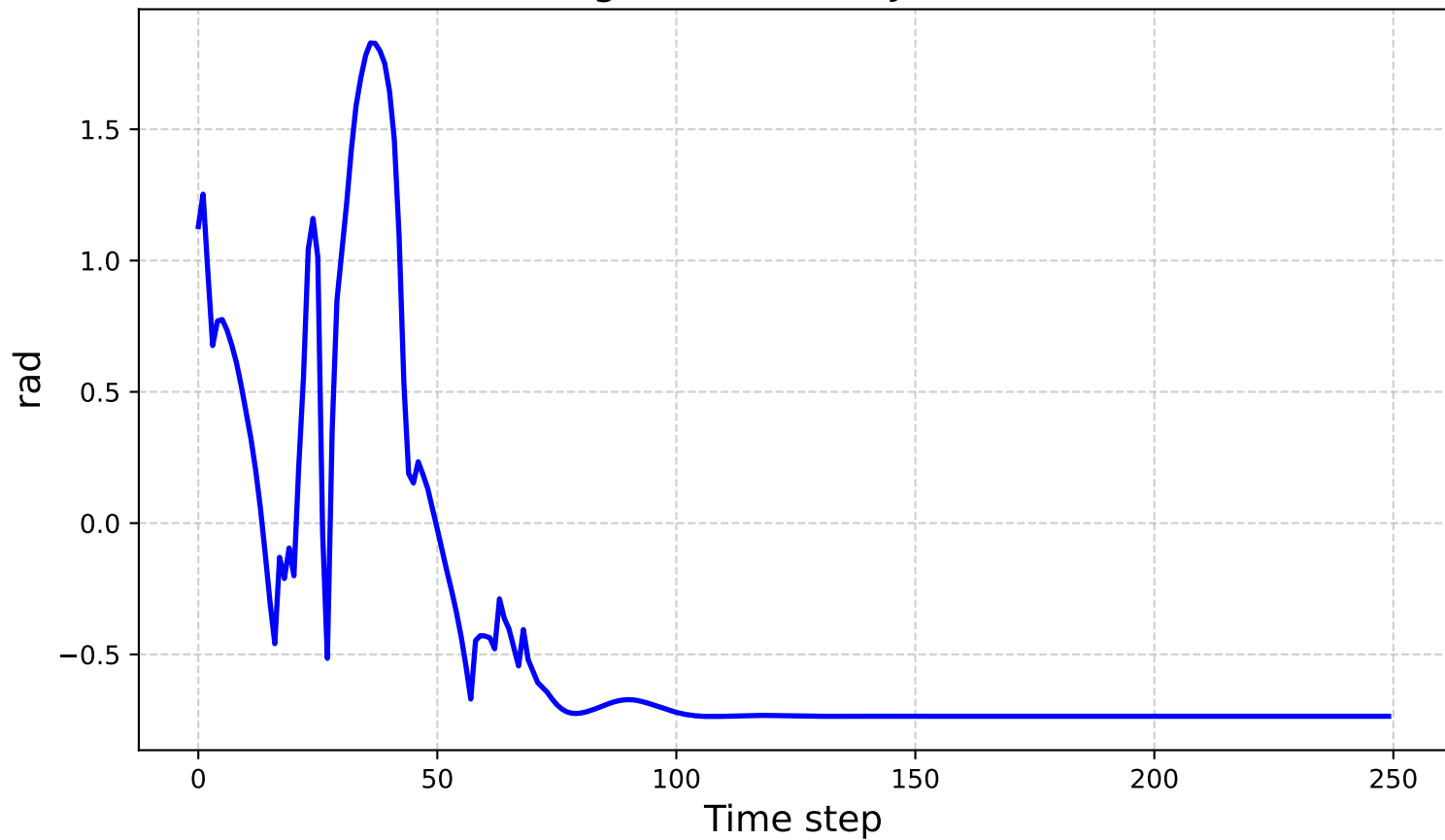
Agent Actions - Joint 5
