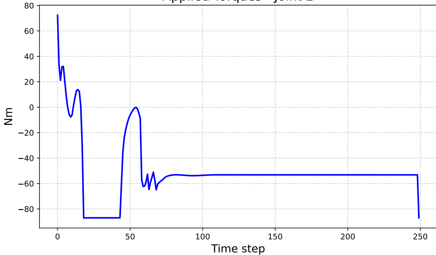
Applied Torques - Joint 2
