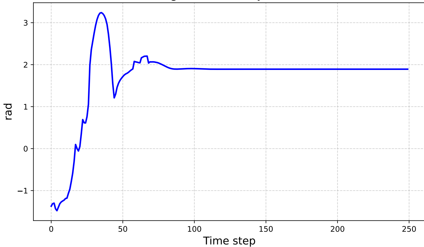
Agent Actions - Joint 6
