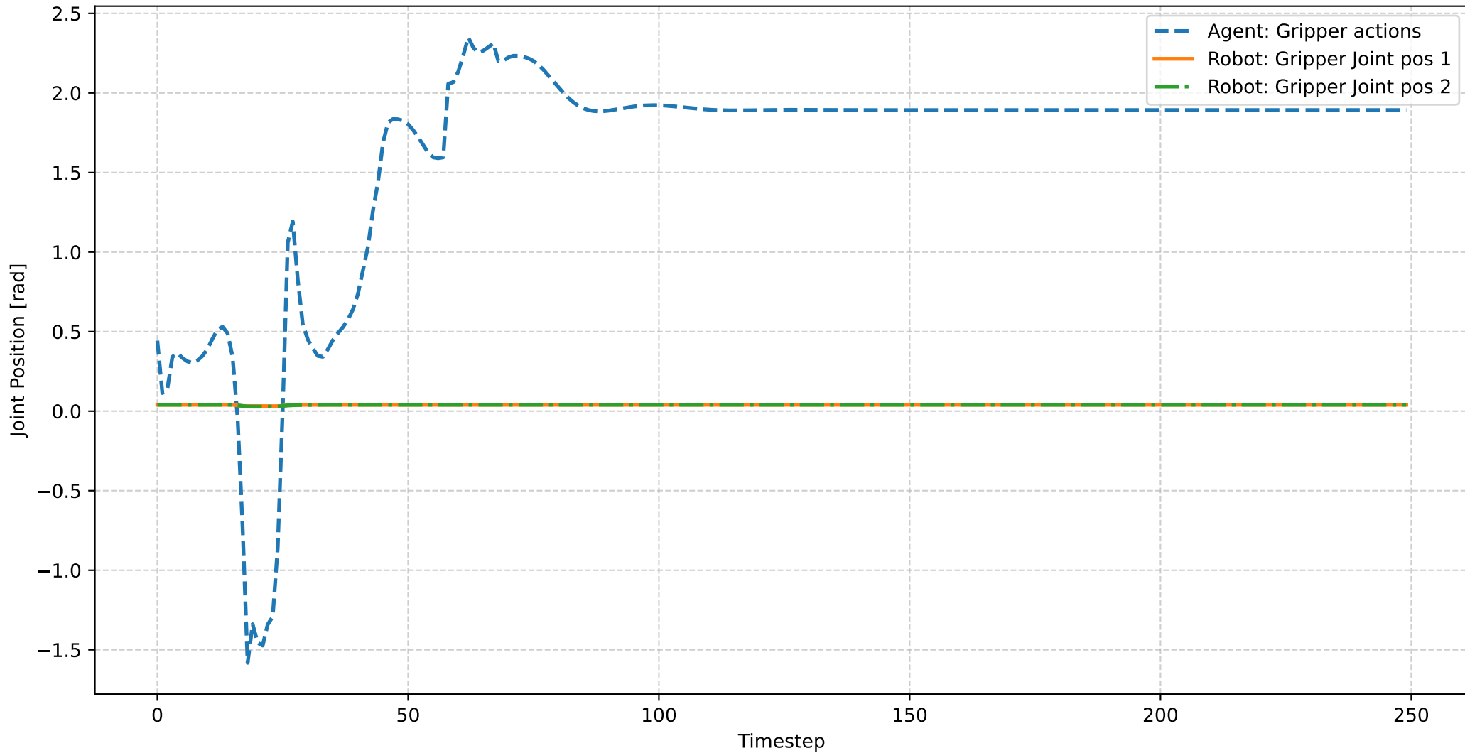
Time Series: Agent Gripper actions vs Robot Griper Joint positions
