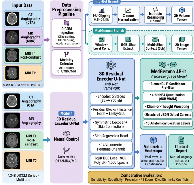
Fig. 1. End-to-end architecture of the proposed dual-model framework for intracranial aneurysm detection. DICOM series undergo modality-specific preprocessing before being routed to the nnU-Net volumetric branch and the MedGemma vision-language branch independently.
