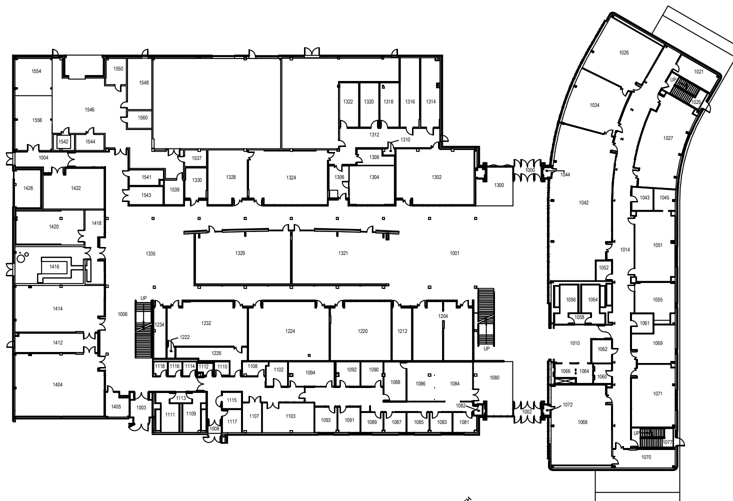
ENGINEERING LAB BUILDING 1001013 SCALE: 1"=50'-0" 1ST FLOOR
