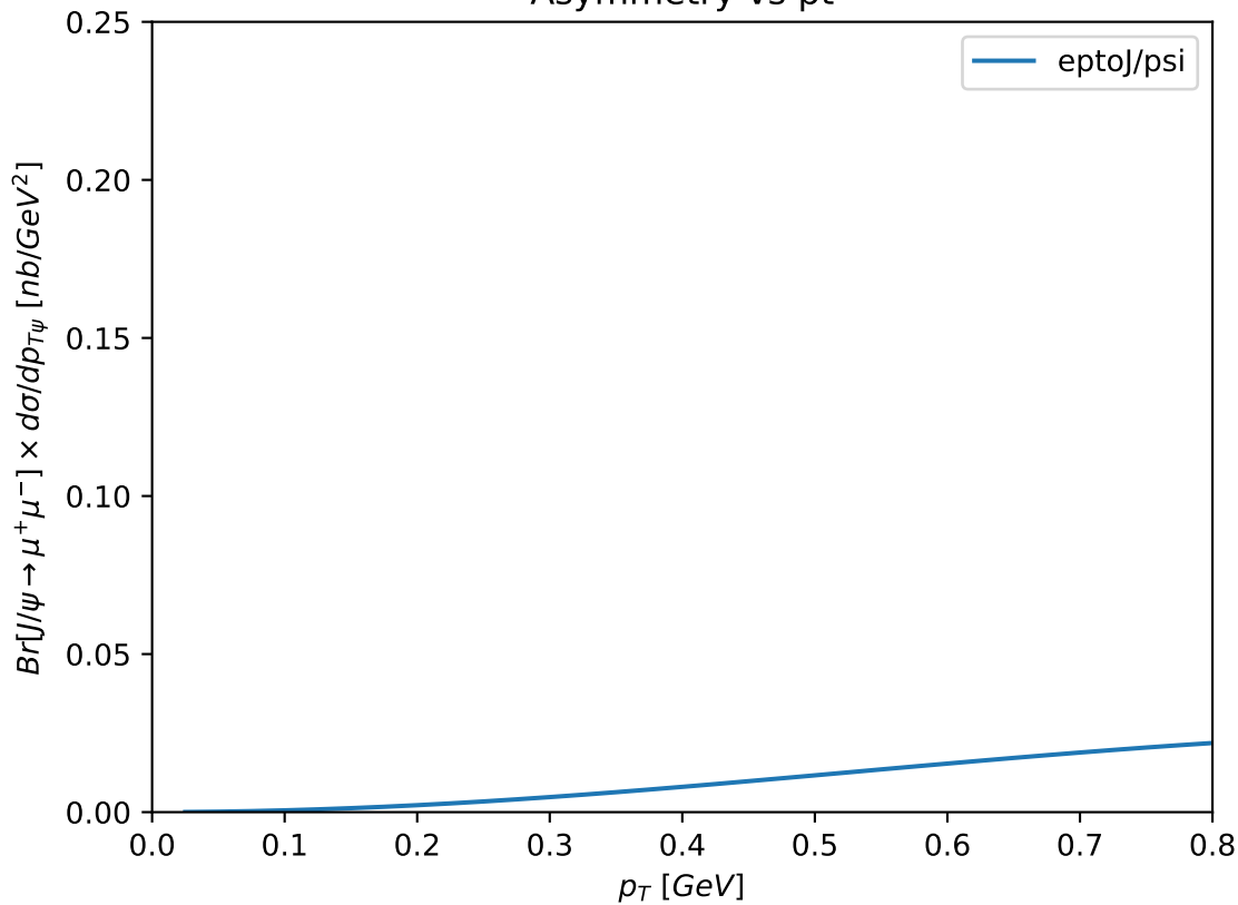
Asymmetry vs pt
