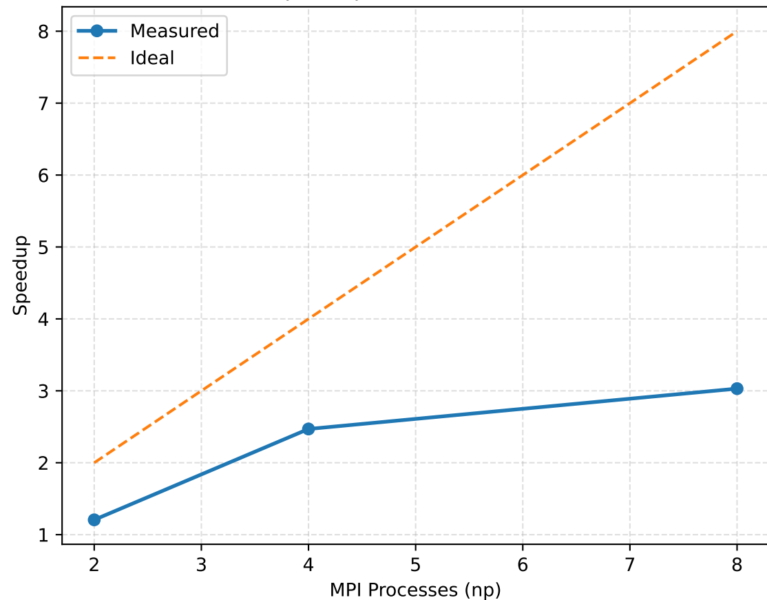
Speedup vs MPI Processes
