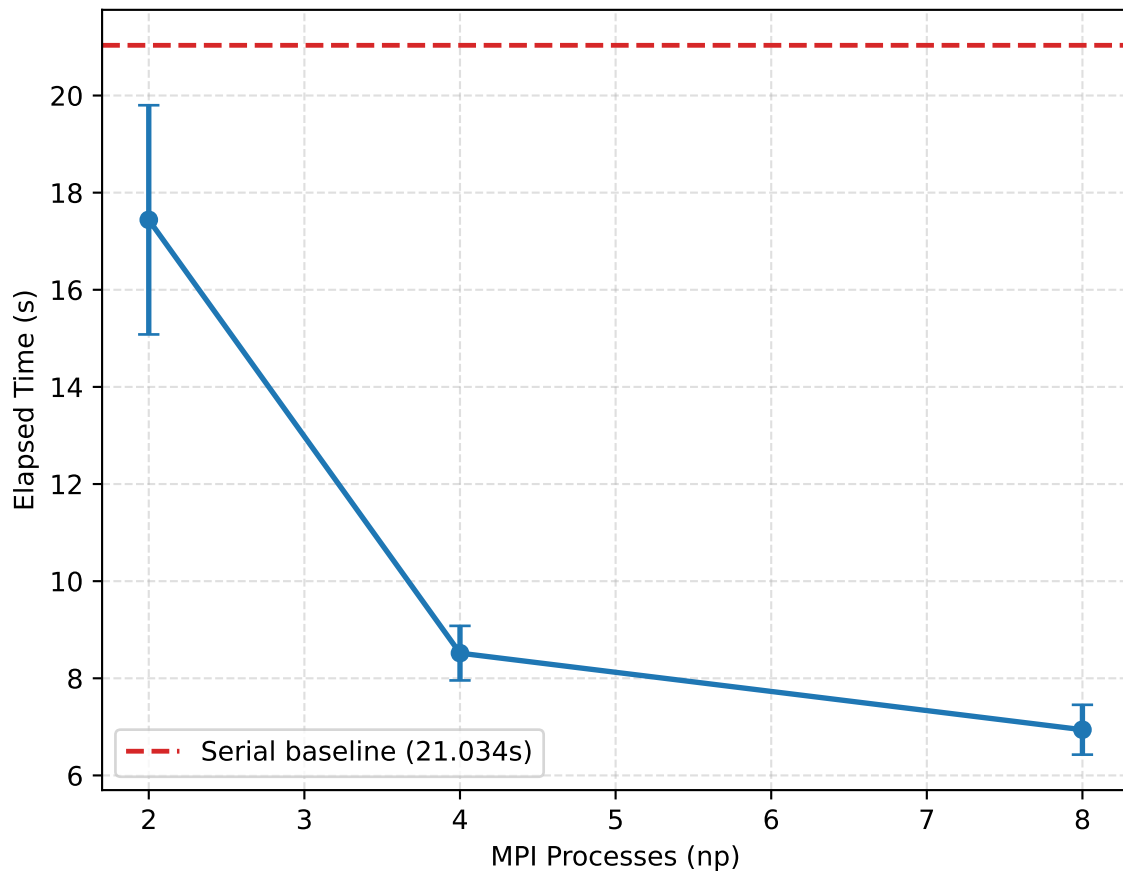
Time vs MPI Processes
