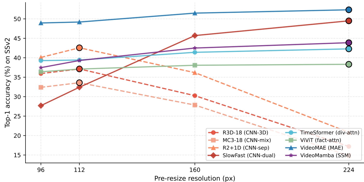
Input-Scale Sensitivity — Accuracy vs. Pre-resize Resolution (SSv2) Native checkpoint; filled = native resolution; dashed = CNN (native 112px)
