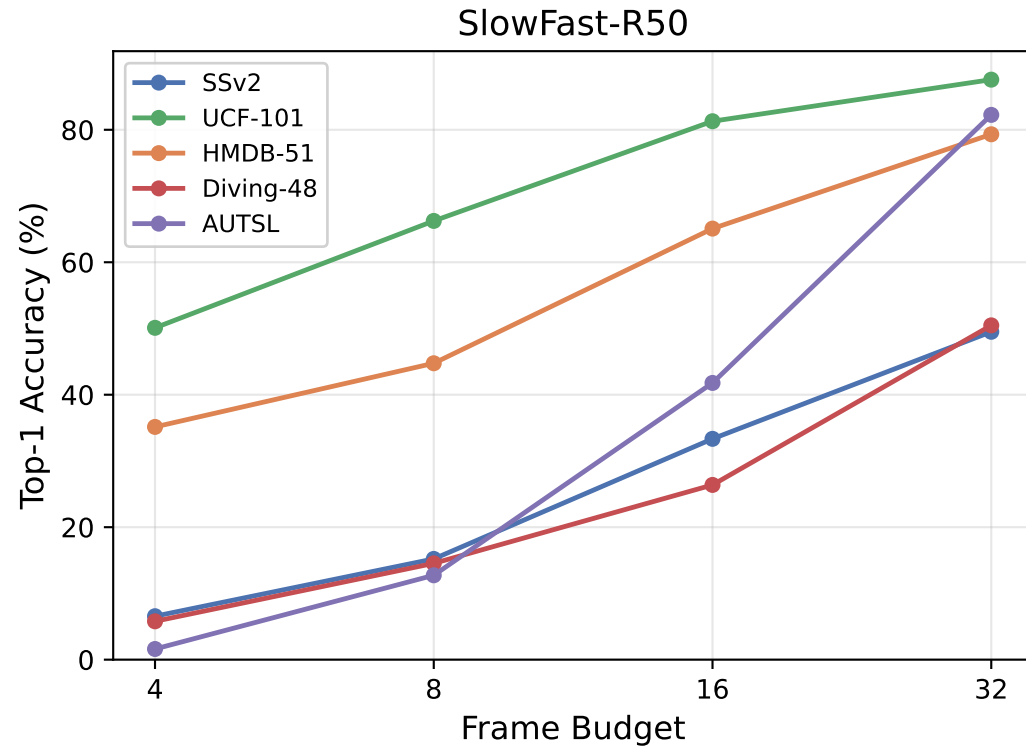
Cross-Dataset: Accuracy vs Frame Budget
