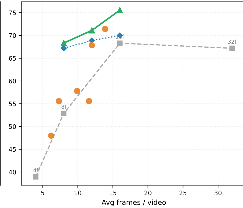
Drive&Act (driving)
