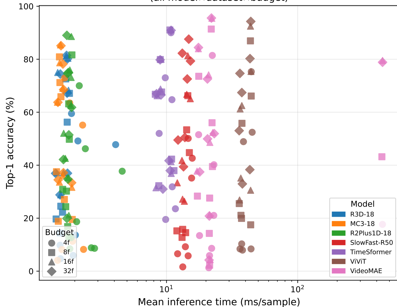
Accuracy vs Inference Latency (all model×dataset×budget)
